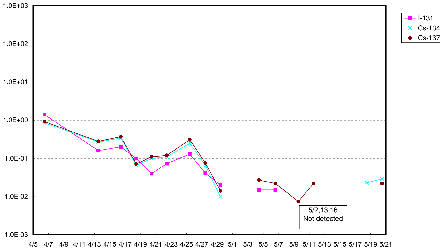
Fukushima Daiichi Nuclear Power Station : Radioactivity Density of Sub-drain at Unit 5 (Bq/cm 3 )
