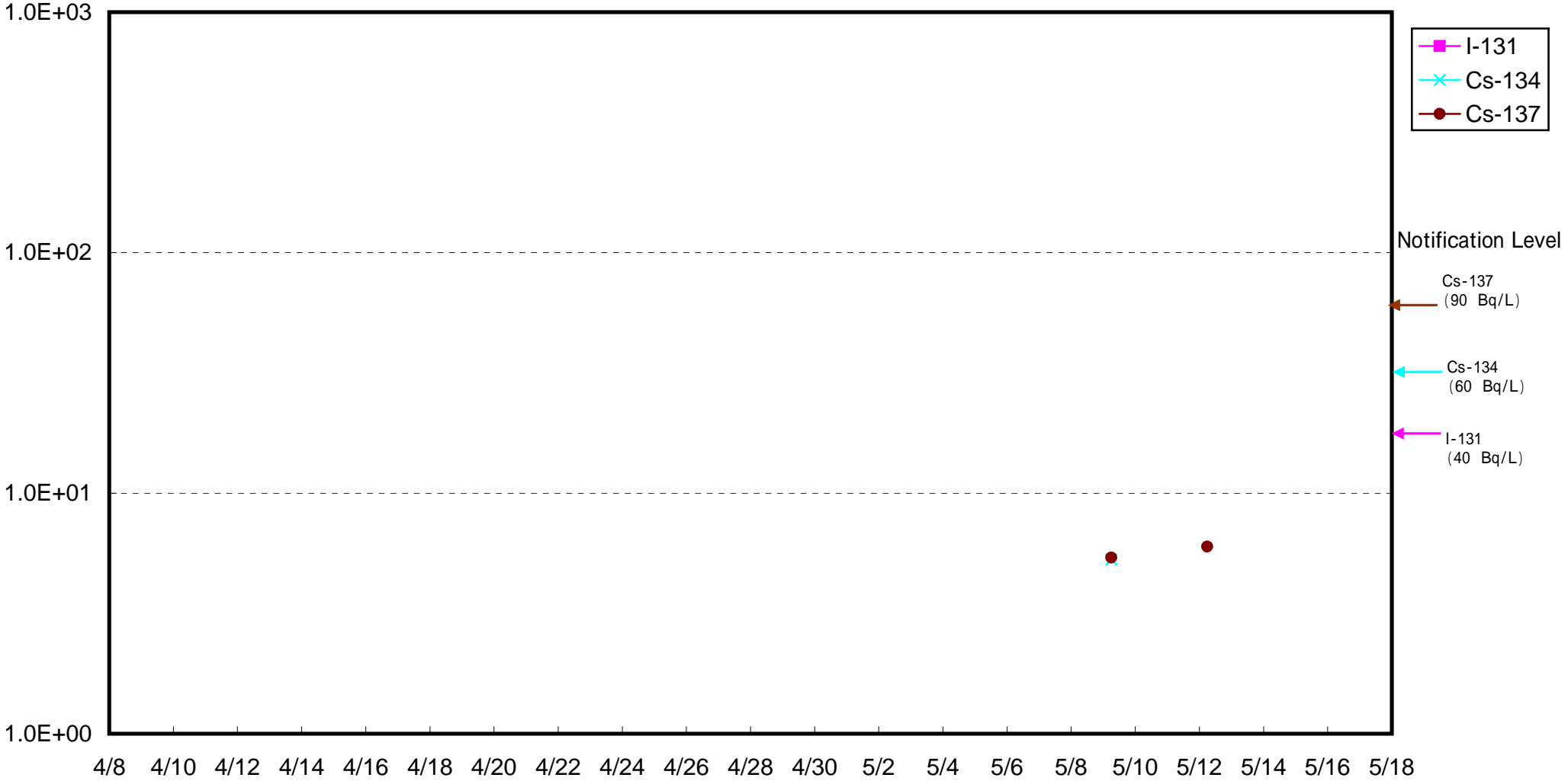
Radioactivity density of Seawater around 3 km offshore of Toyoma port (Bq/L) (Lower layer)
