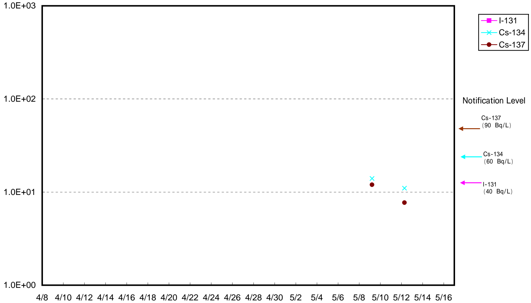
Radioactivity Density of Seawater around 3 km northern offshore of Iwaki city (Bq/L) (Lower layer)
