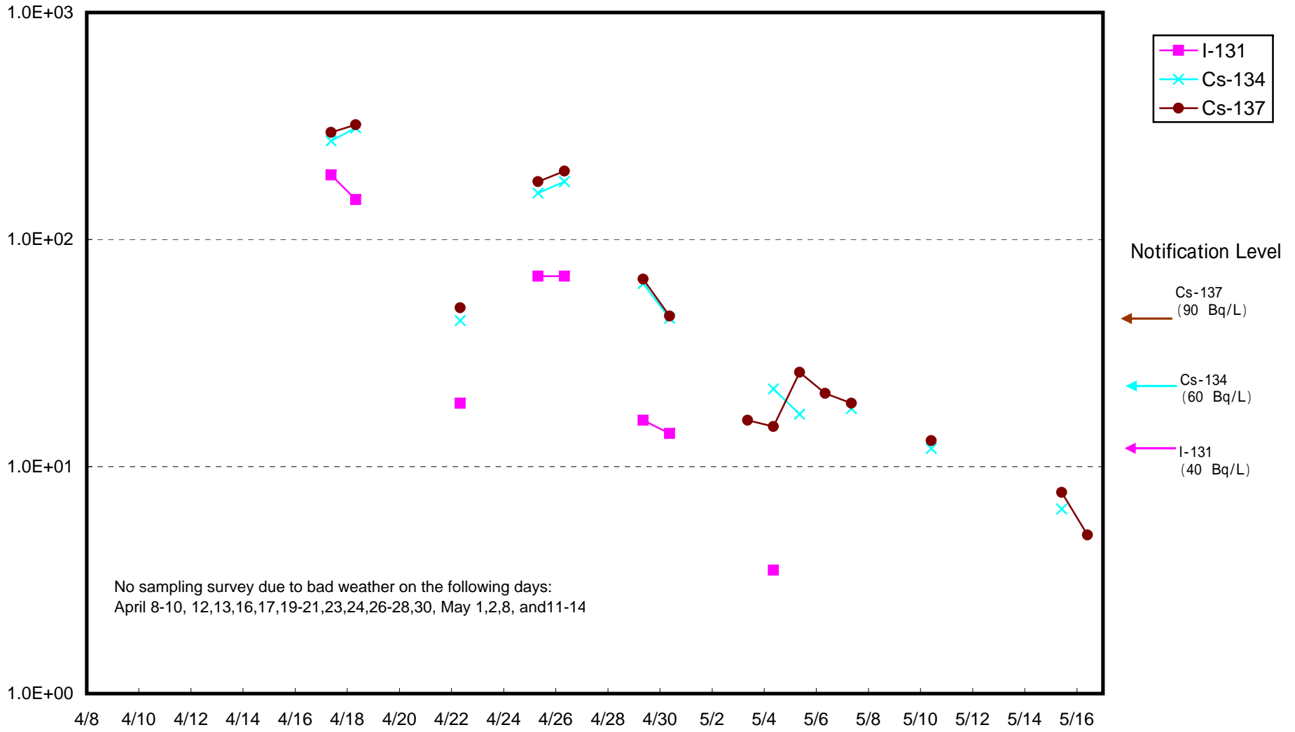
Radioactivity Density of Seawater around 8 km offshore of Iwasawa Shore (Bq/L) (Upper layer)
