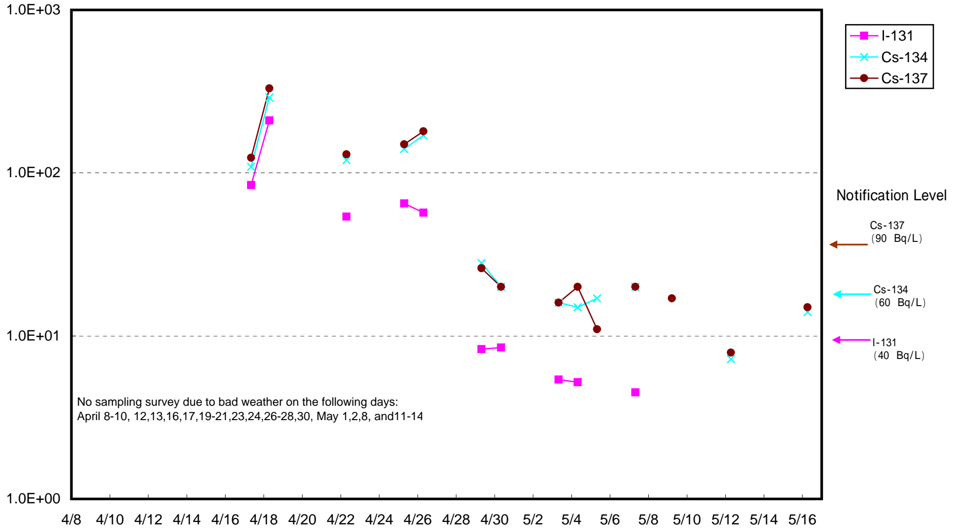
Radioactivity Density of Seawater around 3 km northern offshore of Iwaki city (Bq/L) (Upper layer)
