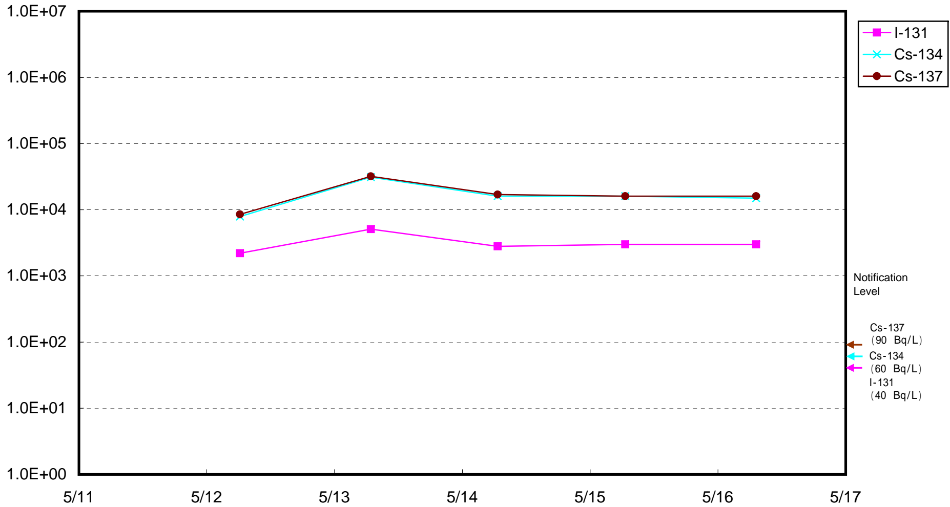
Radioactivity Density of Seawater around the Bar Screen of Unit 1 of Fukushima Daiichi NPS (inside of the Silt Fence) (Bq/ L)
