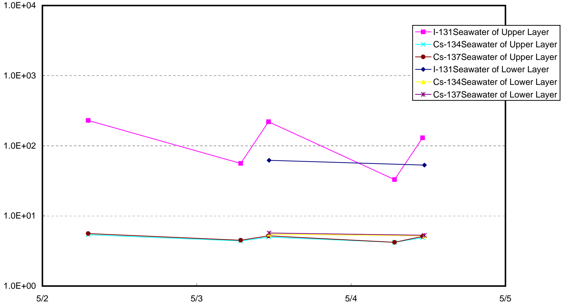
Fukushima Daiichi Nuclear Power Station: Radioactivity density of Seawater at around the Bar Screen of 1F Unit 2 (inside of the silt fence) (Bq/cm 3 )
