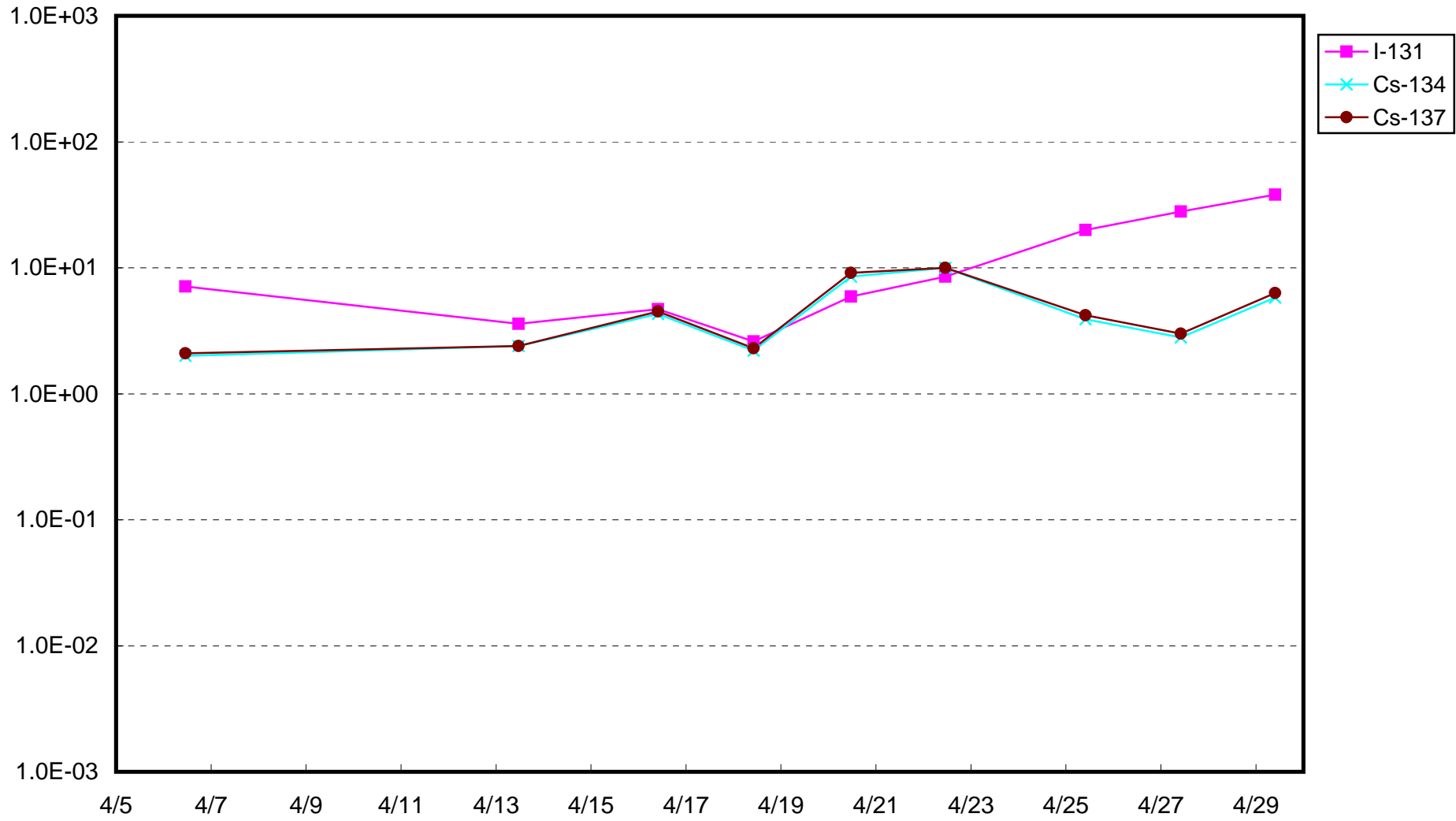
Fukushima Daiichi Nuclear Power Station : Radioactivity Density of Sub-drain of Unit 3 (Bq/cm 3 )
