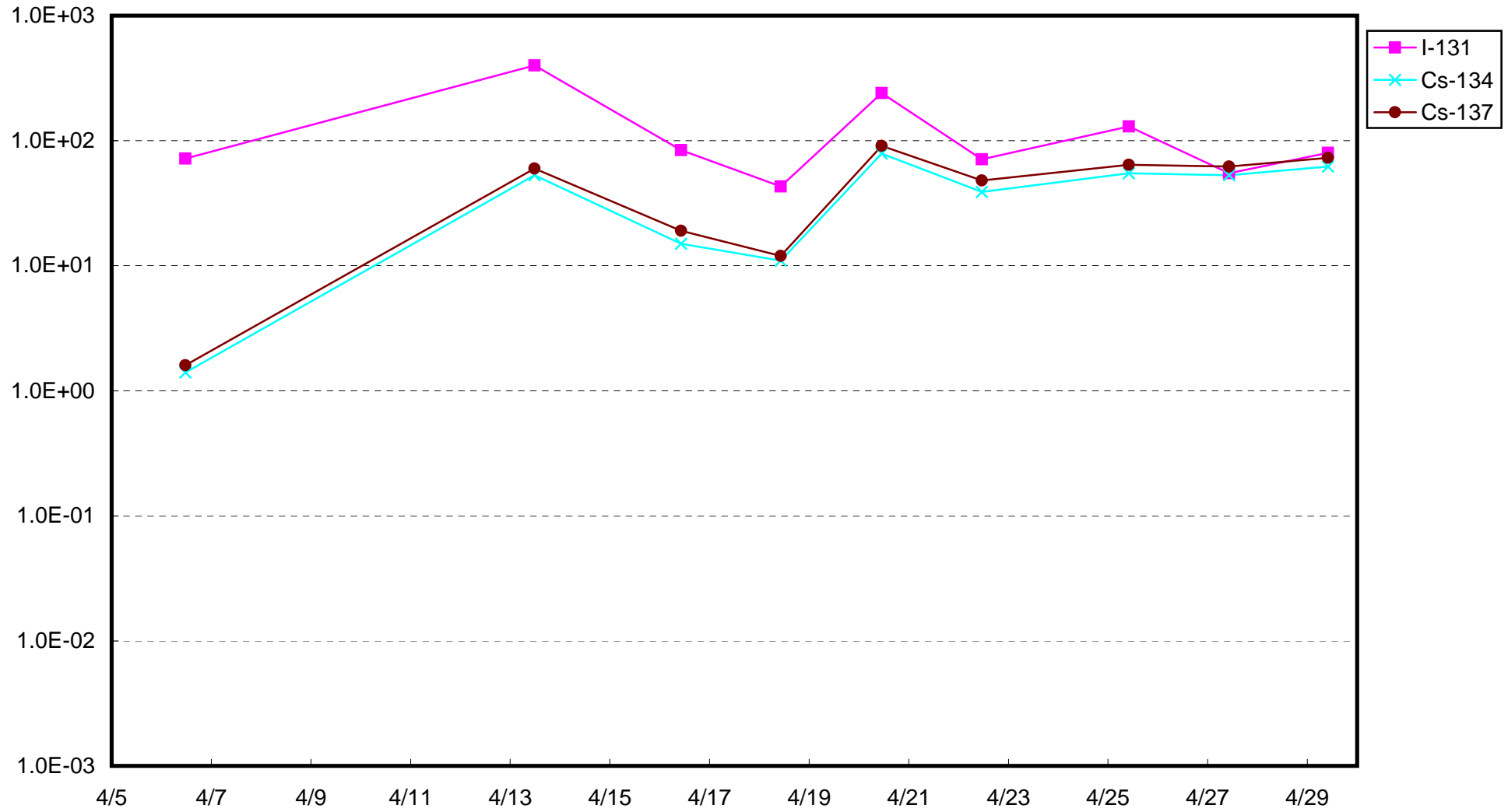
Fukushima Daiichi Nuclear Power Station : Radioactivity Density of Sub-drain of Unit1 (Bq/cm 3 )
