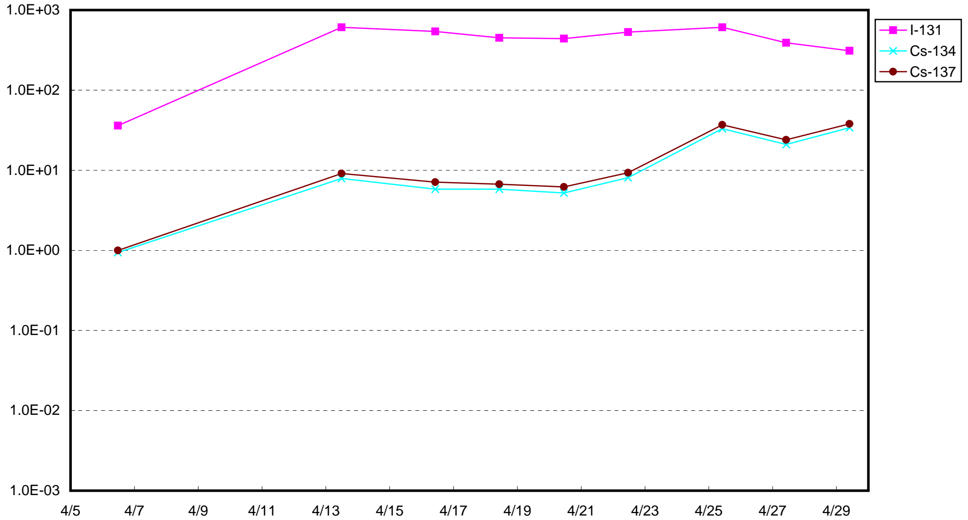
Fukushima Daiichi Nuclear Power Station : Radioactivity Density of Sub-drain of Unit 2 (Bq/cm 3 )
