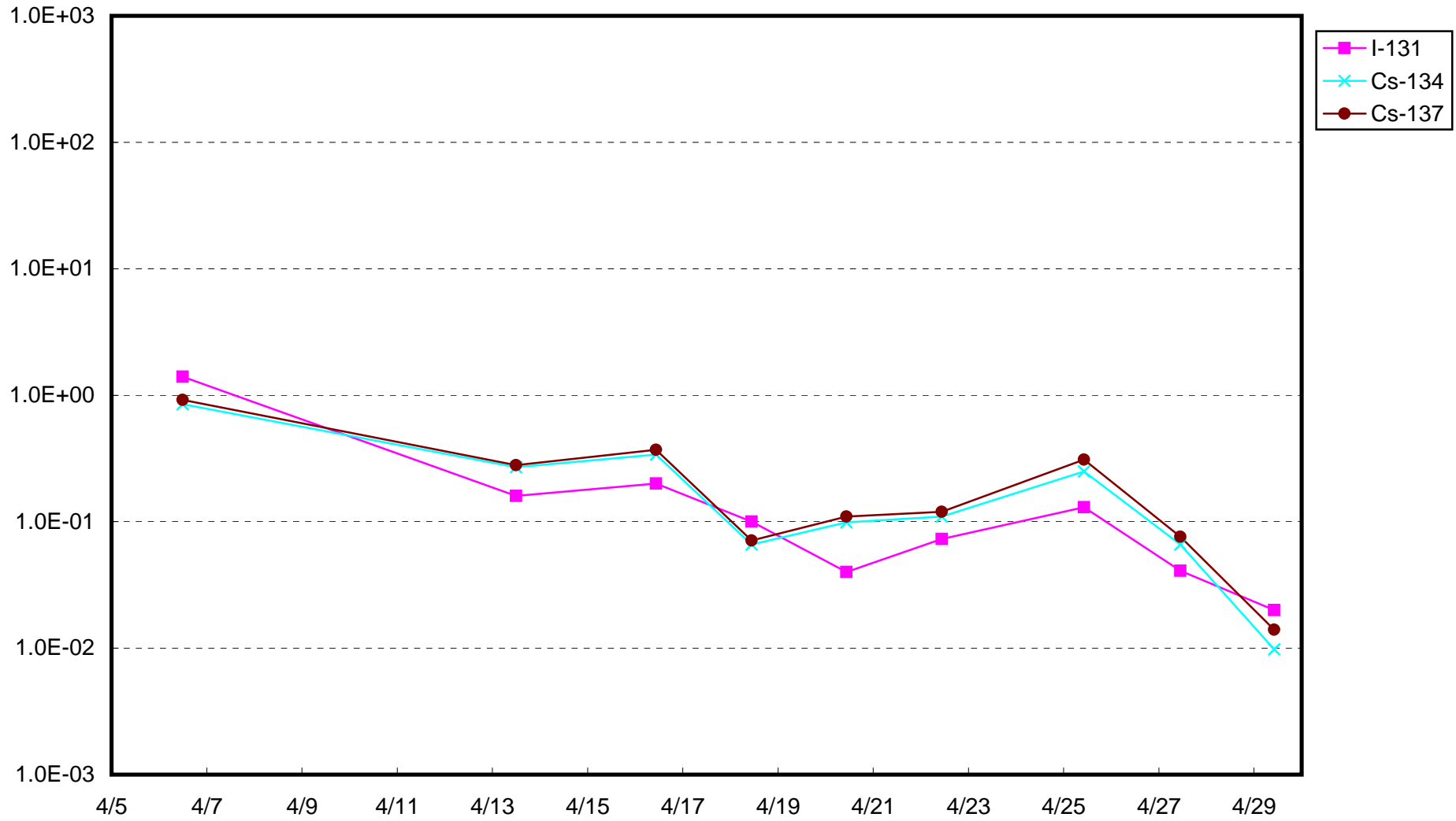
Fukushima Daiichi Nuclear Power Station : Radioactivity Density of Sub-drain of Unit 5 (Bq/cm 3 )
