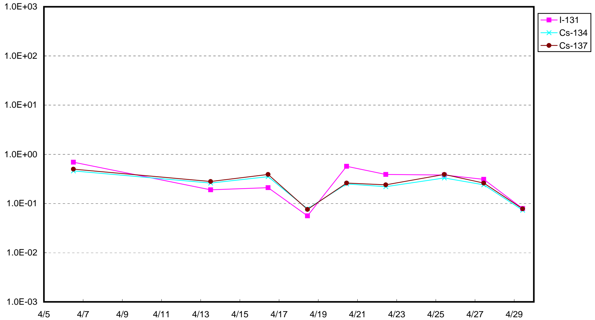
Fukushima Daiichi Nuclear Power Station : Radioactivity Density of Sub-drain of Unit 6 (Bq/cm 3 )
