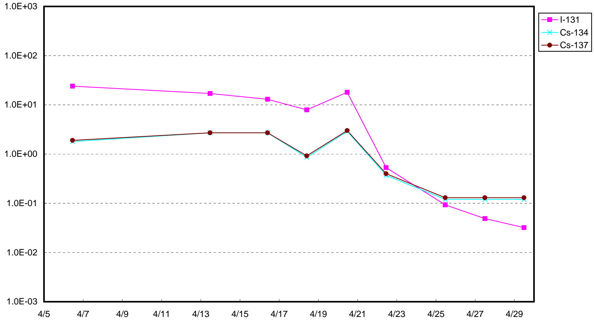
Fukushima Daiichi Nuclear Power Station : Radioactivity Density of Sub-drain of Unit 4 (Bq/cm 3 )
