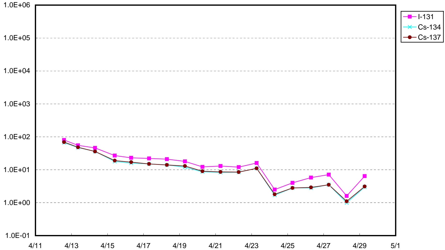
Radioactivity density of seawater at the north of Unit 1-4 water intake of Fukushima Daiichi NPS (Bq / cm 3 )
