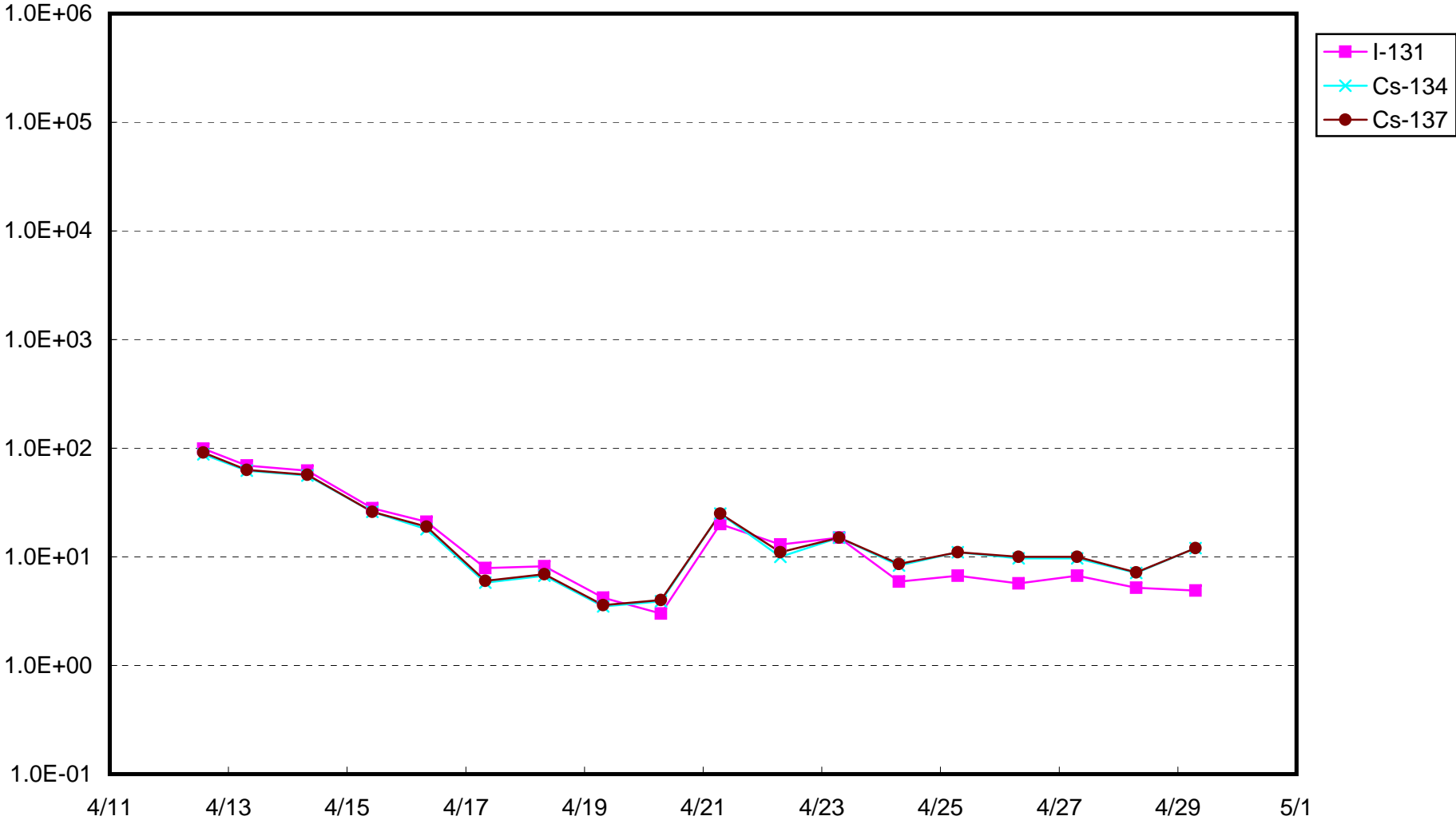
Radioactivity density of seawater at the south of Unit 1-4 water intake of Fukushima Daiichi NPS (Bq / cm 3 )
