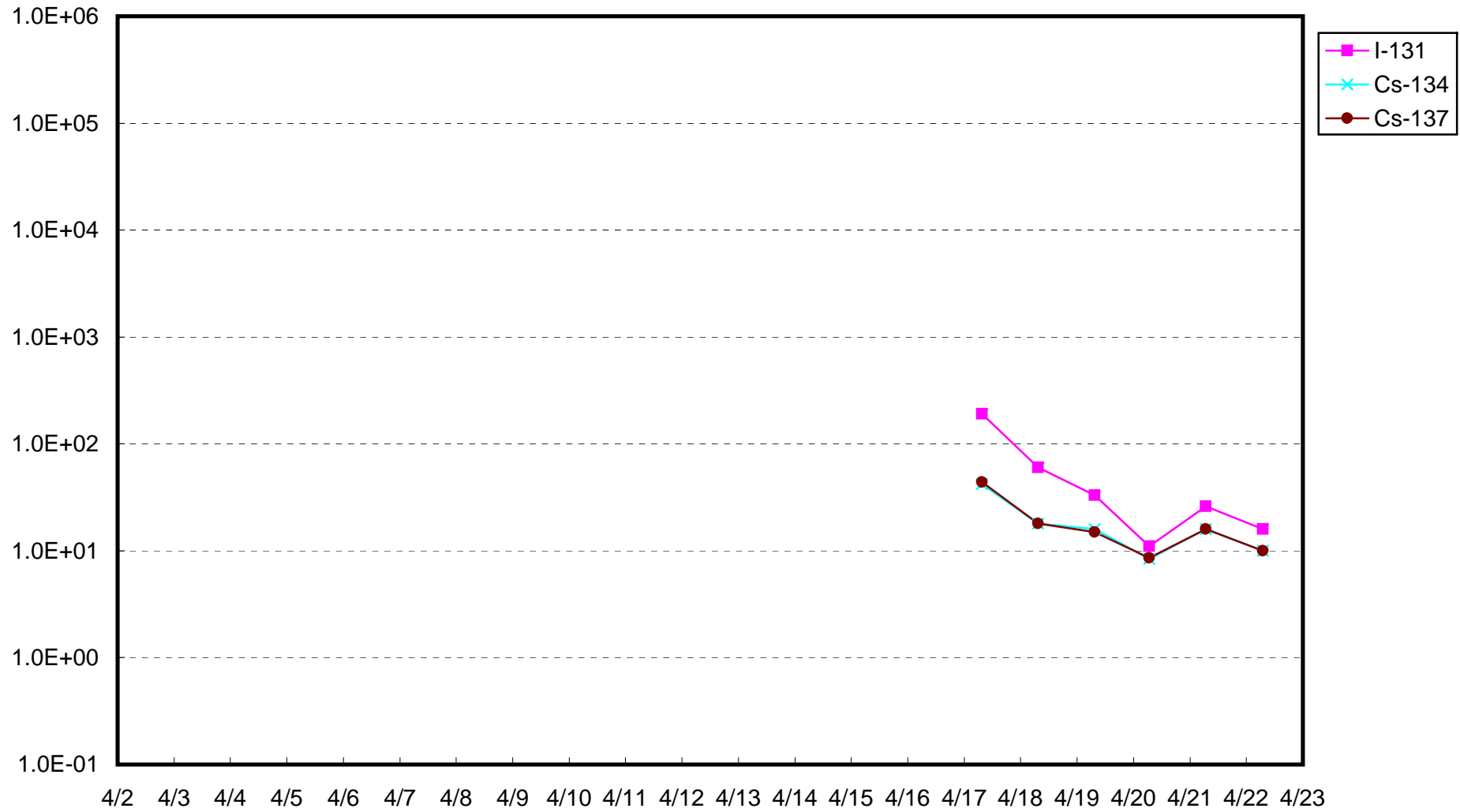
Radioactivity density of seawater around the bar screen of Unit 2 (the outside of the silt fence ), Fukuchima Daiichi NPS( Bq / cm 3 )
