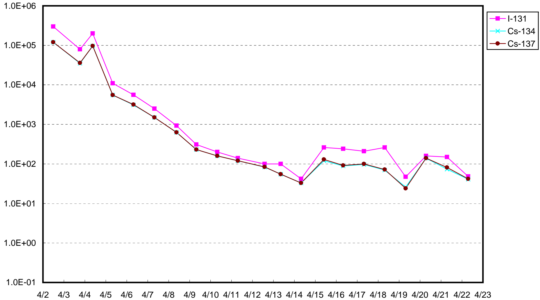
Radioactivity density of seawater around the bar screen of Unit2 (the inside od the silt fence) ( B q / c m 3 )
