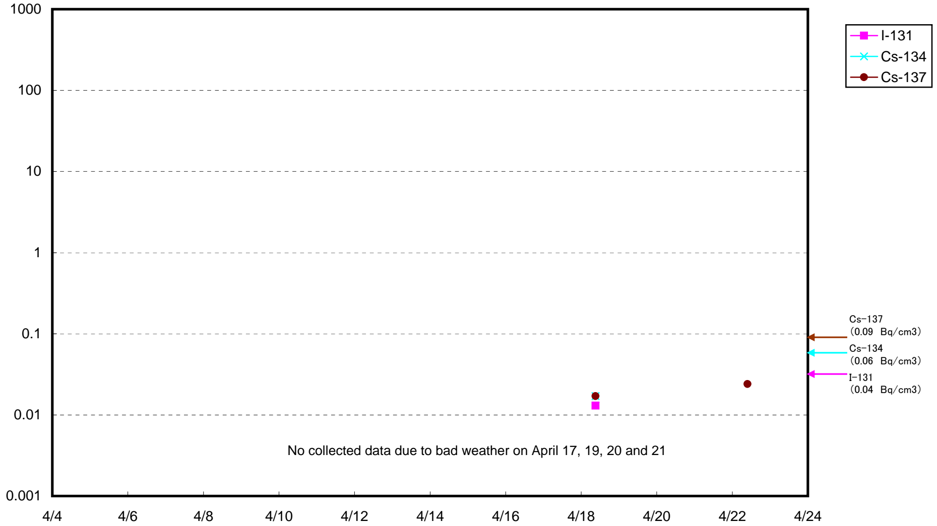
Radioactivity Density of Seawater at 8 km offshore of Odaka-ku (Bq/cm 3 )
