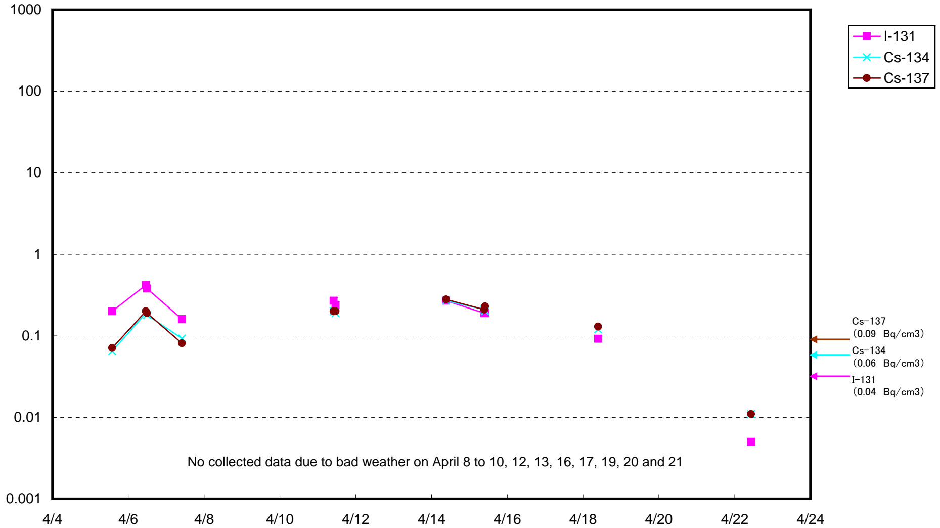
Radioactivity Density of Seawater at 15 km offshore of Ukedo-gawa (Bq/cm 3 )
