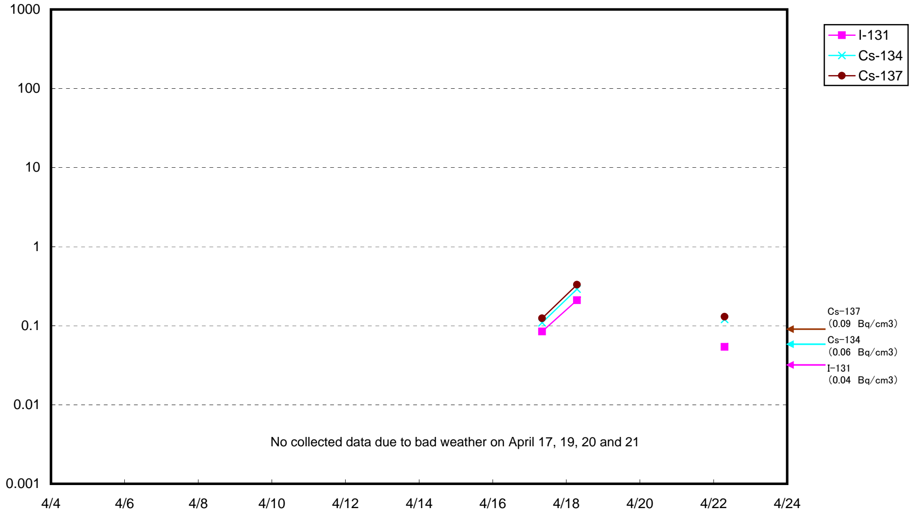
Radioactivity Density of Seawater at 3 km offshore of Iwaki City (Bq/cm 3 )
