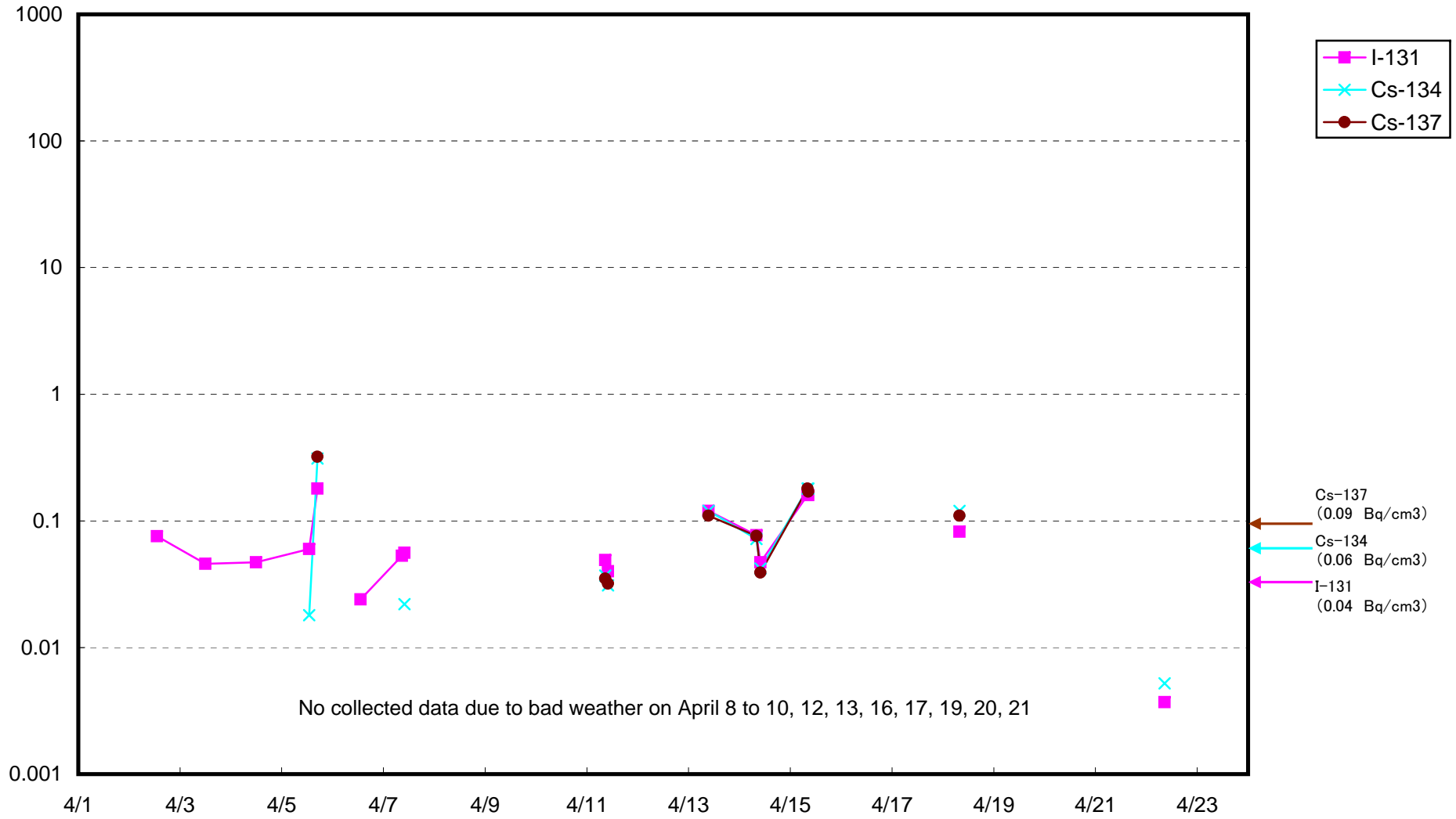
Radioactivity Density of Seawater at 15 km offshore of Iwasawa Shore (Bq/cm 3 )
