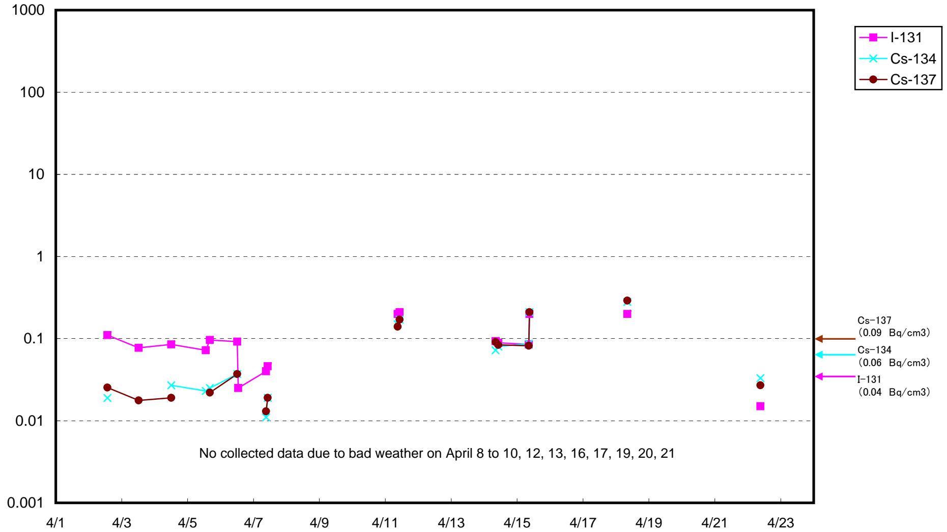
Radioactivity Density of Seawater at 15 km offshore of Fukushima Daini (Bq/cm 3 )
