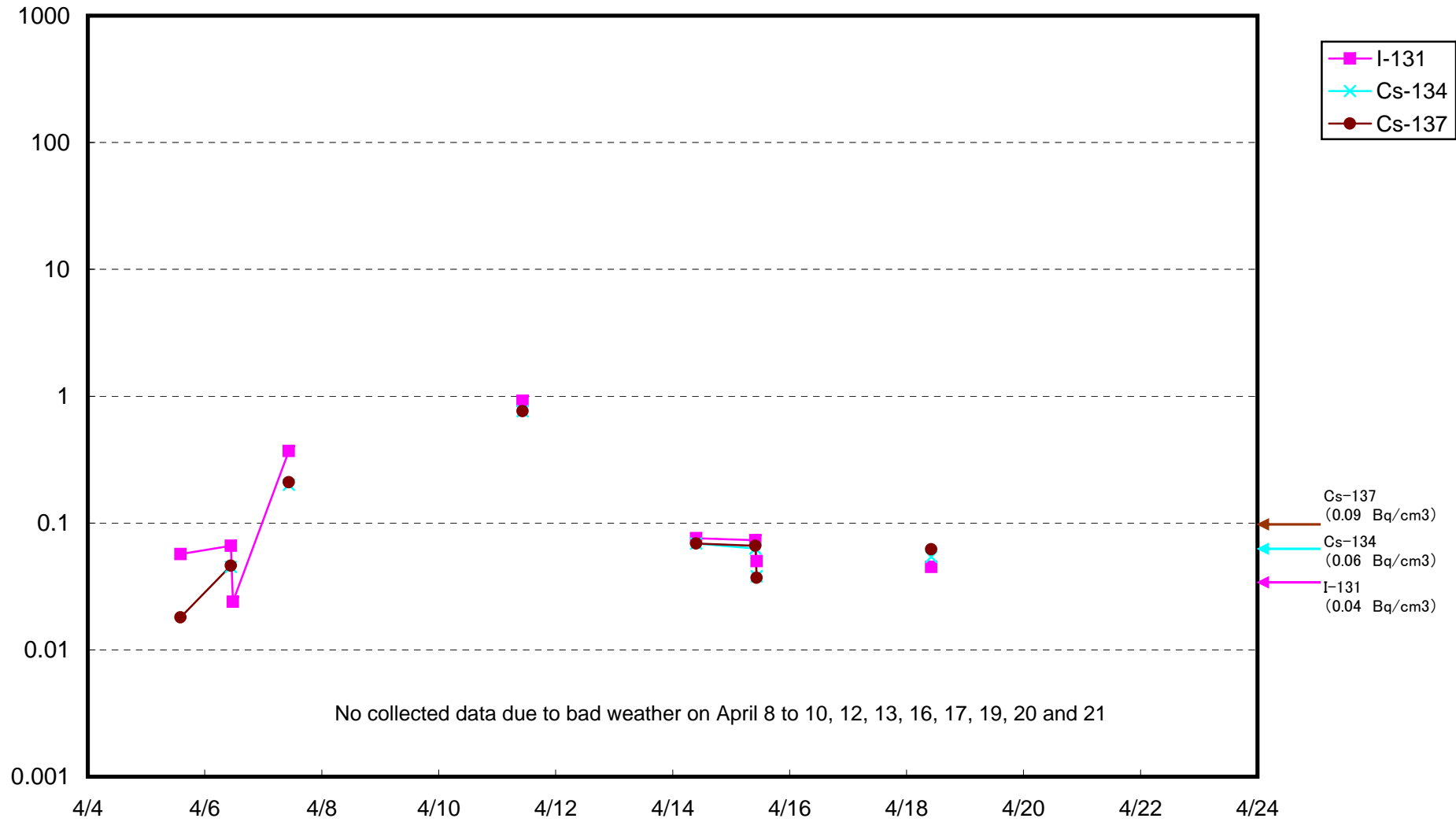
Radioactivity Density of Seawater at 15 km offshore of Minami Souma City (Bq/cm 3 )
