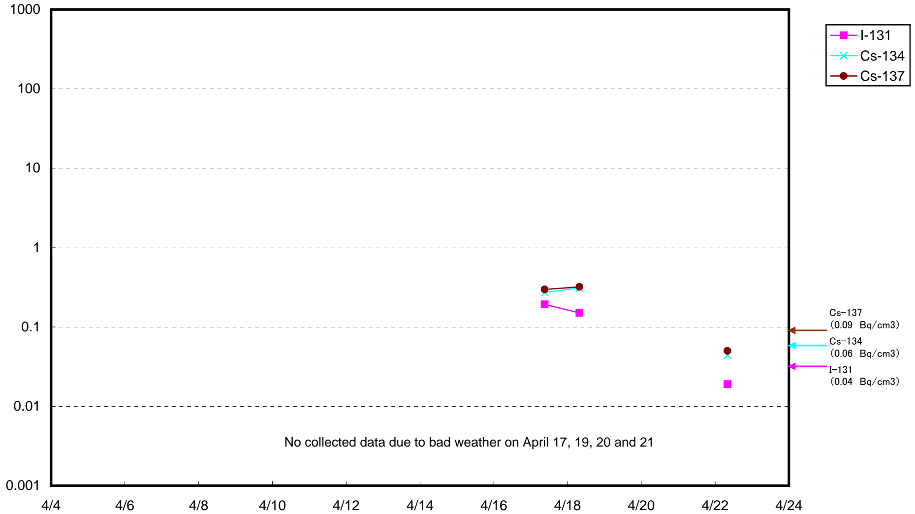
Radioactivity Density of Seawater at 8 km offshore of Iwasawa Shore (Bq/cm 3 )
