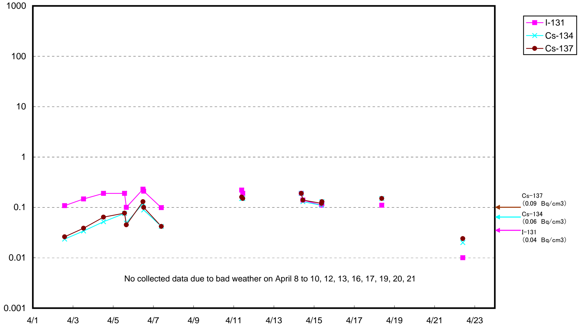
Radioactivity Density of Seawater at 15 km offshore of Fukushima Daiichi (Bq/cm 3 )
