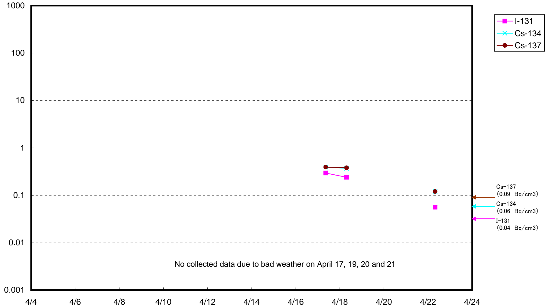
Radioactivity Density of Seawater at 3 km offshore of Iwasawa Shore (Bq/cm 3 )
