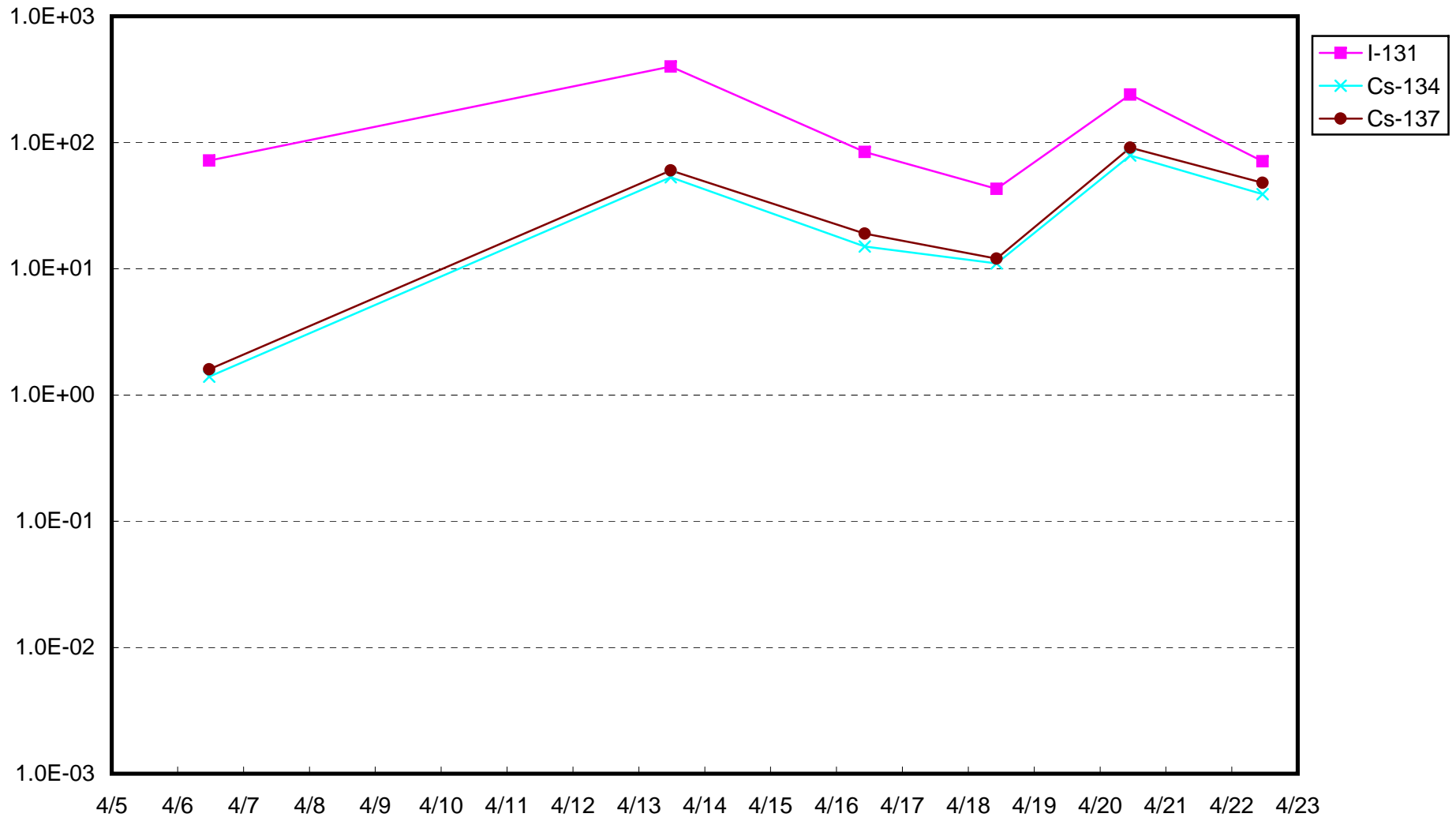
Fukushima Daiichi Nuclear Power Station : Density of Sub-drain of Unit1 (Bq/cm 3 )
