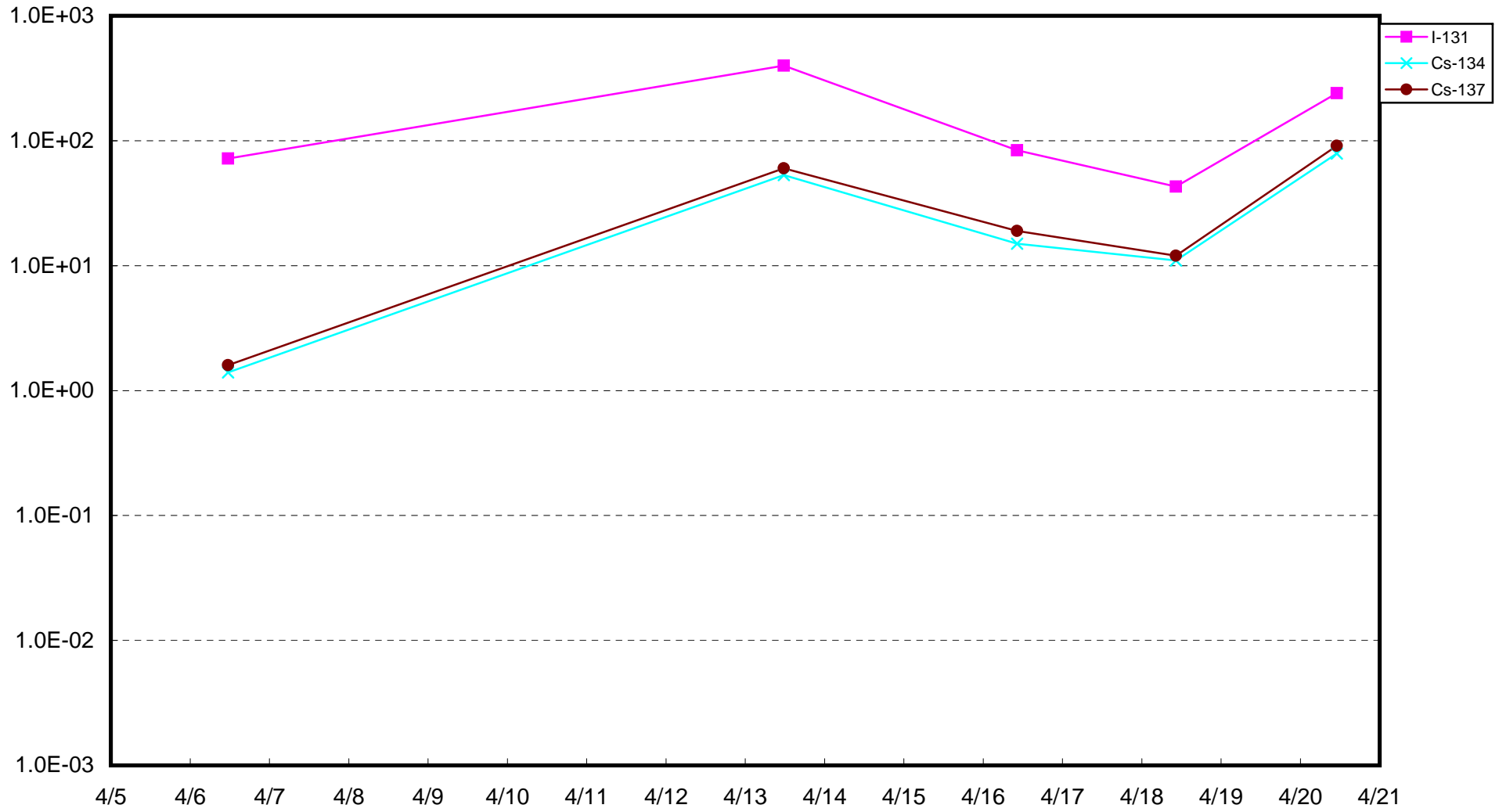
Fukushima Daiichi Nuclear Power Station : Density of Sub-drain of Unit1 (Bq/cm 3 )
