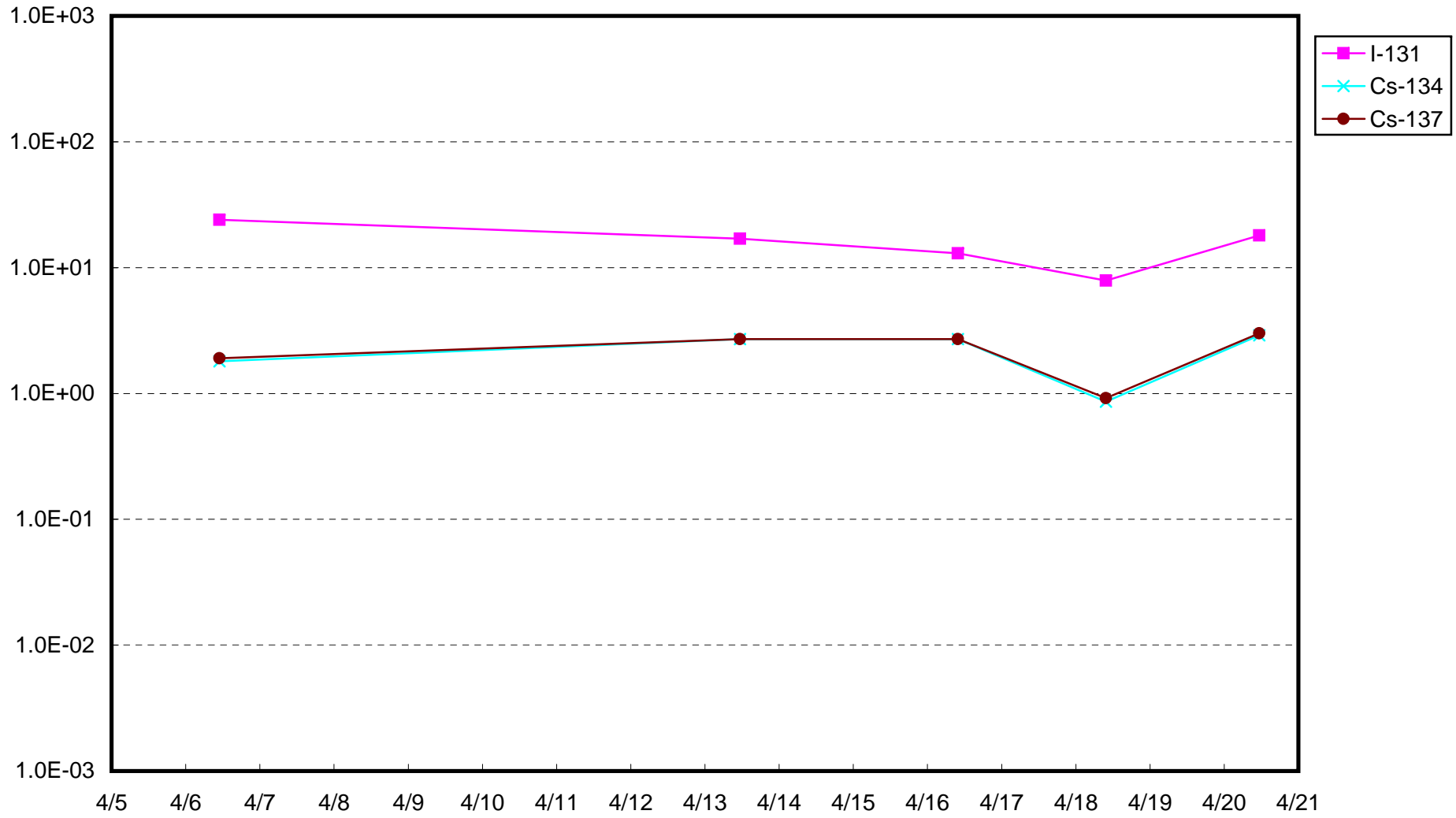
Fukushima Daiich Nuclear Power Station : Radioactivity Density of Sub-drain of Unit 4(Bq/cm 3 )
