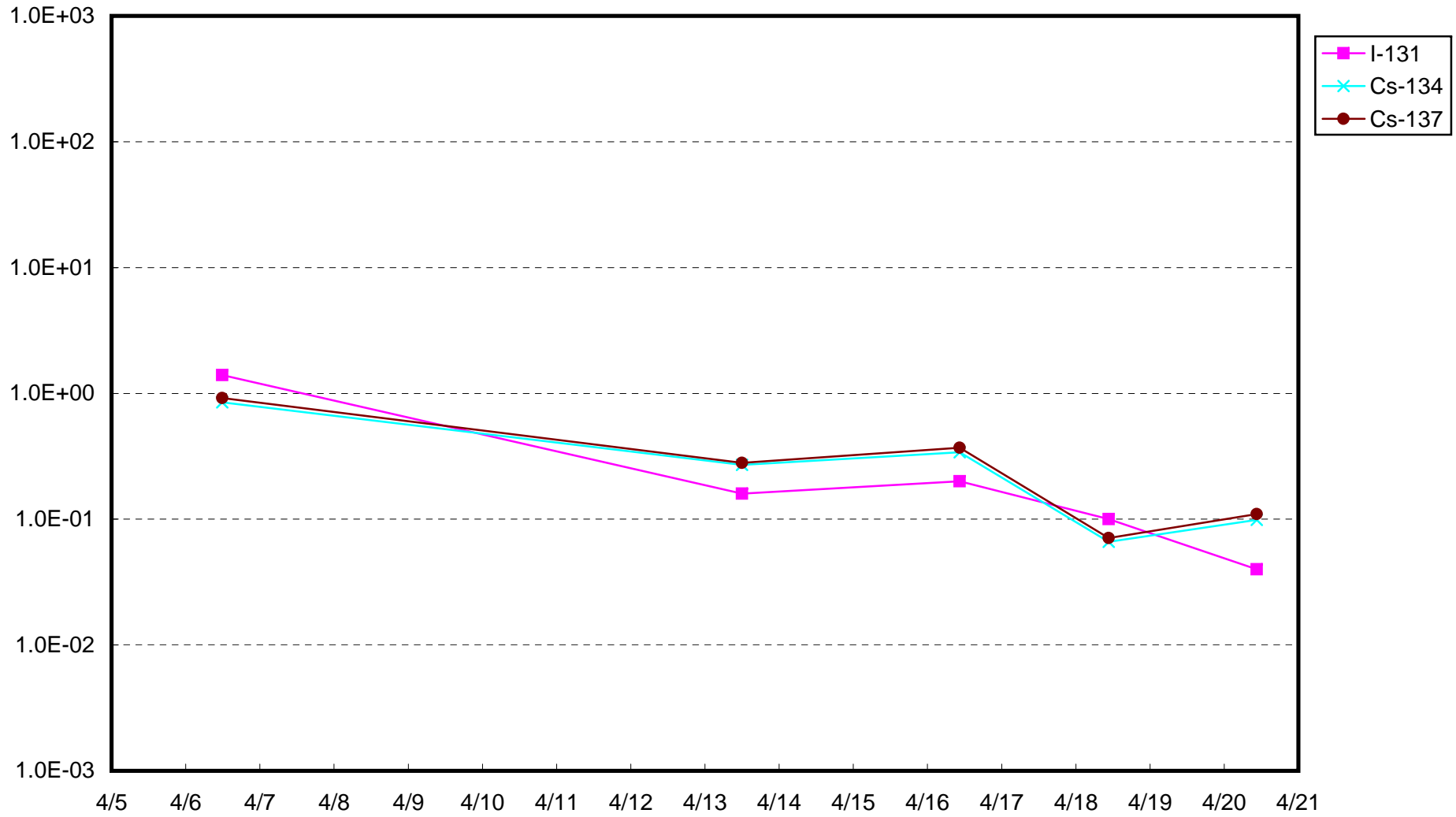
Fukushima Daiich Nuclear Power Station : Radioactivity Density of Sub-drain of Unit 5 (Bq/cm 3 )
