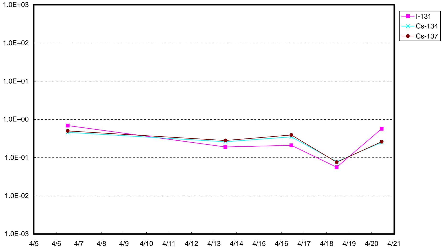
Fukushima Daiich Nuclear Power Station : Radioactivity Density of Sub-drain of Unit 6 (Bq/cm 3 )
