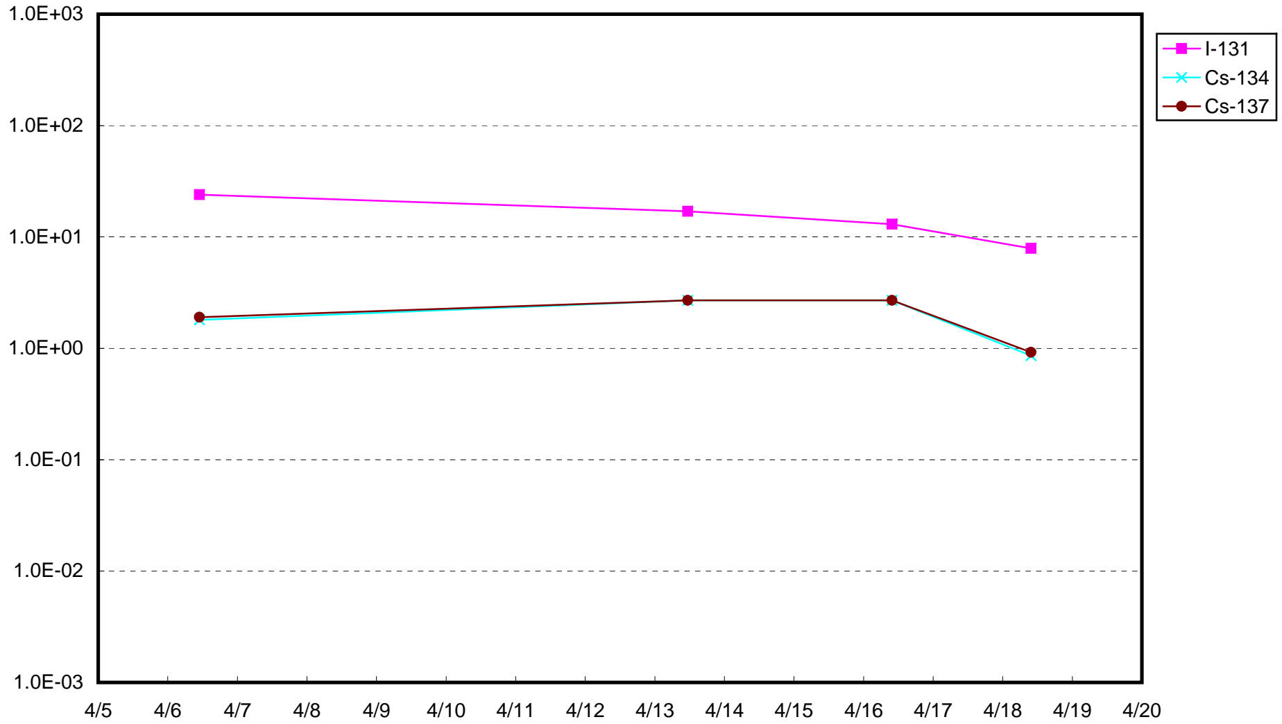
Fukushima Daiich Nuclear Power Station : Radioactivity Density of Sub-drain of Unit 4(Bq/cm 3 )
