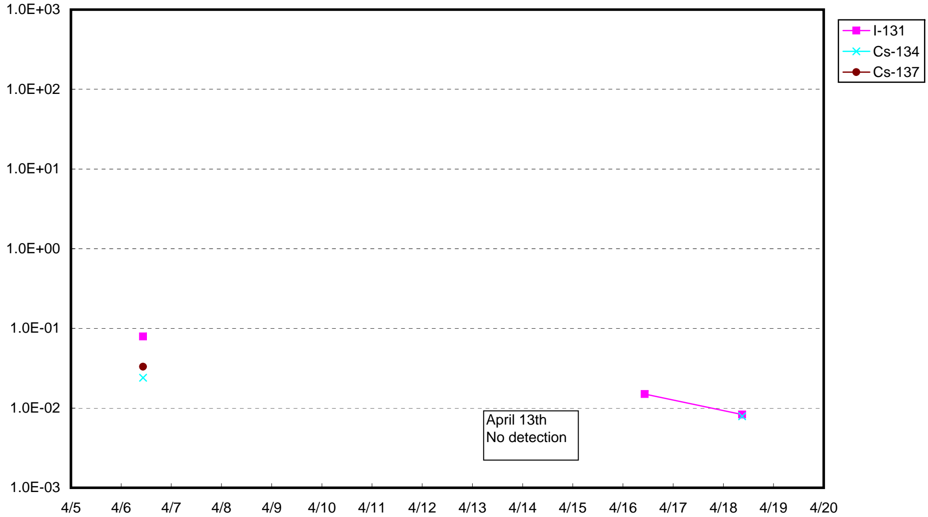
Fukushima Daiich Nuclear Power Station : Radioactivity Density of the deep well at the site (Bq/cm 3 )
