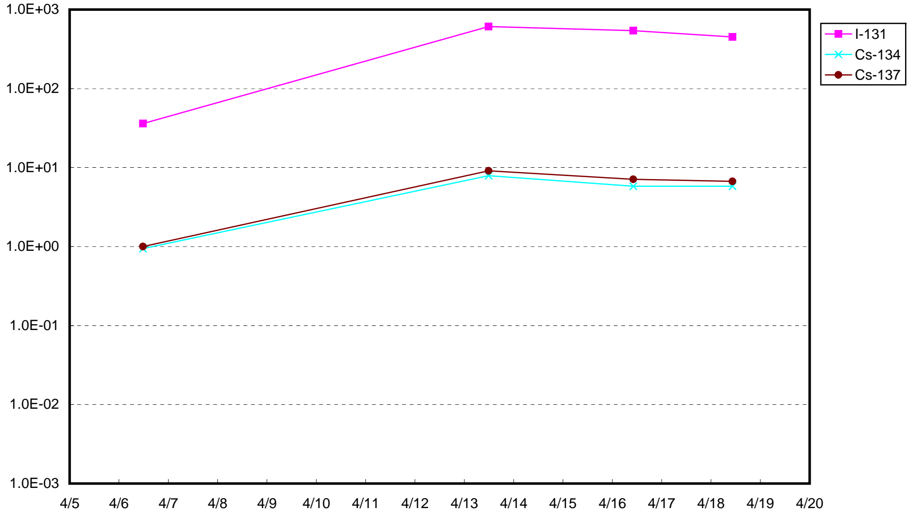
Fukushima Daiich Nuclear Power Station : Radioactivity Density of Sub-drain of Unit 2(Bq/cm 3 )
