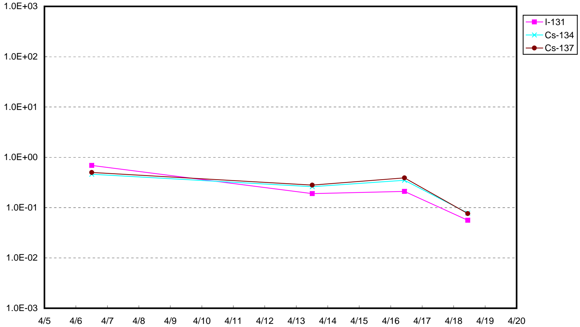
Fukushima Daiich Nuclear Power Station : Radioactivity Density of Sub-drain of Unit 6(Bq/cm 3 )
