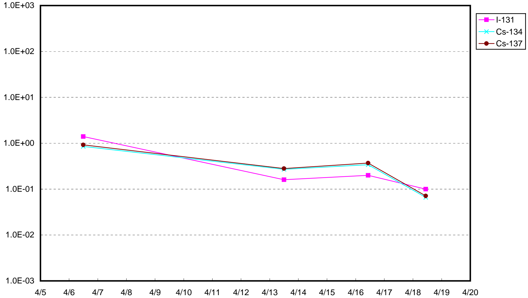
Fukushima Daiich Nuclear Power Station : Radioactivity Density of Sub-drain of Unit 5(Bq/cm 3 )
