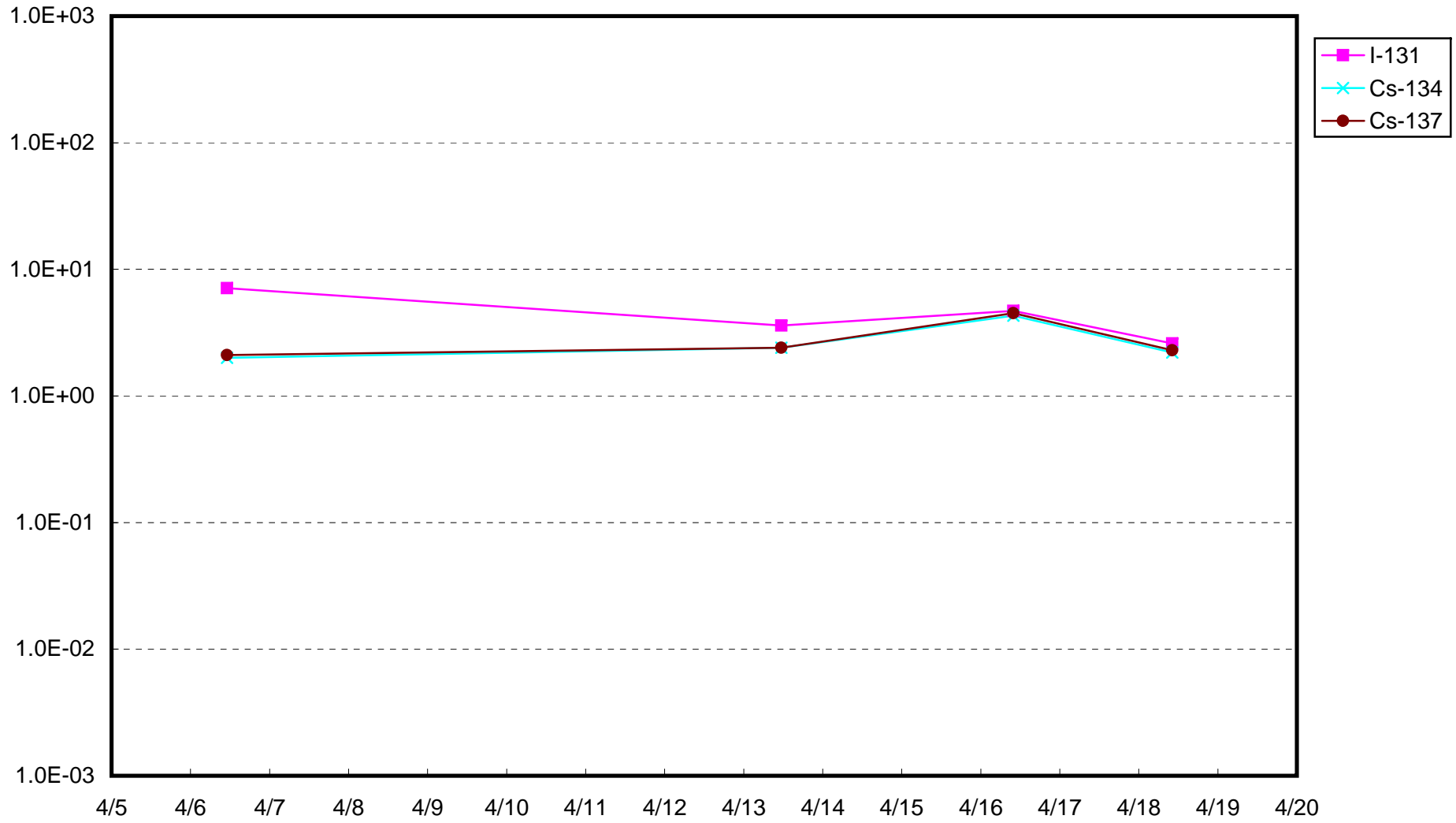
Fukushima Daiich Nuclear Power Station : Radioactivity Density of Sub-drain of Unit 3(Bq/cm 3 )
