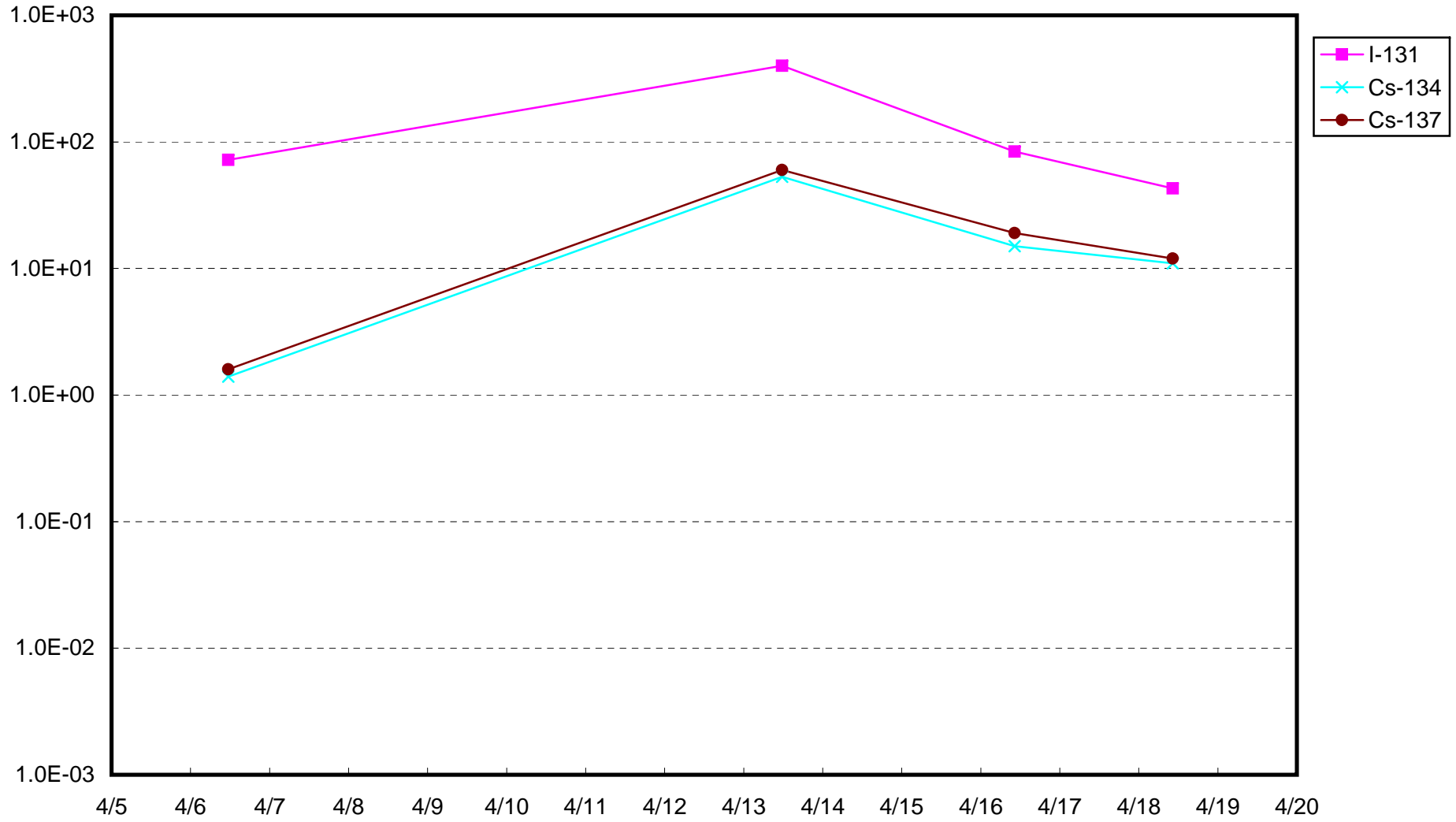
Fukushima Daiich Nuclear Power Station : Radioactivity Density of Sub-drain of Unit 1 (Bq/cm 3 )
