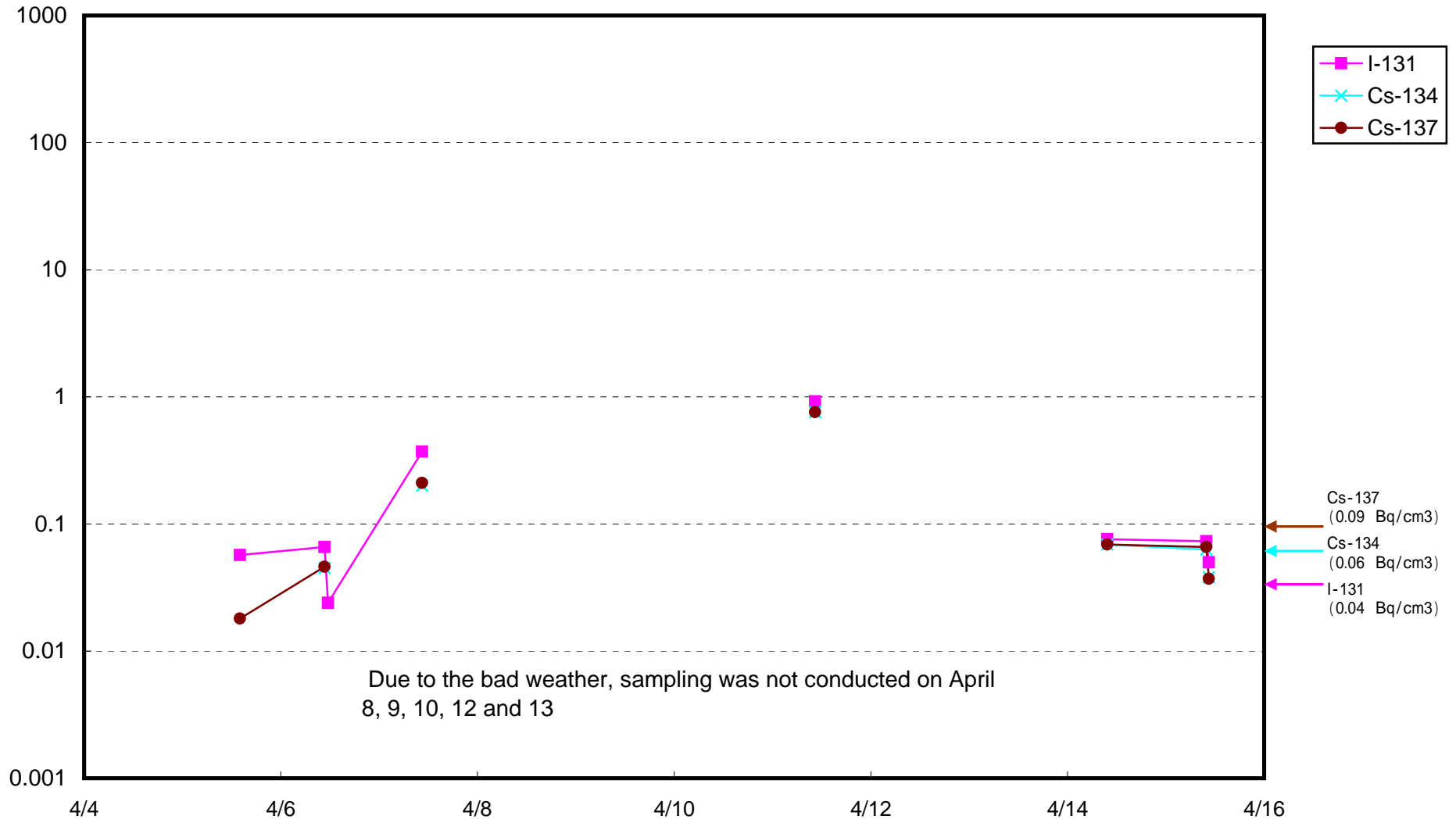
Radioactivity Density of Seawater at 15km off the coast of Minami Souma City ( B q / c m 3 )
