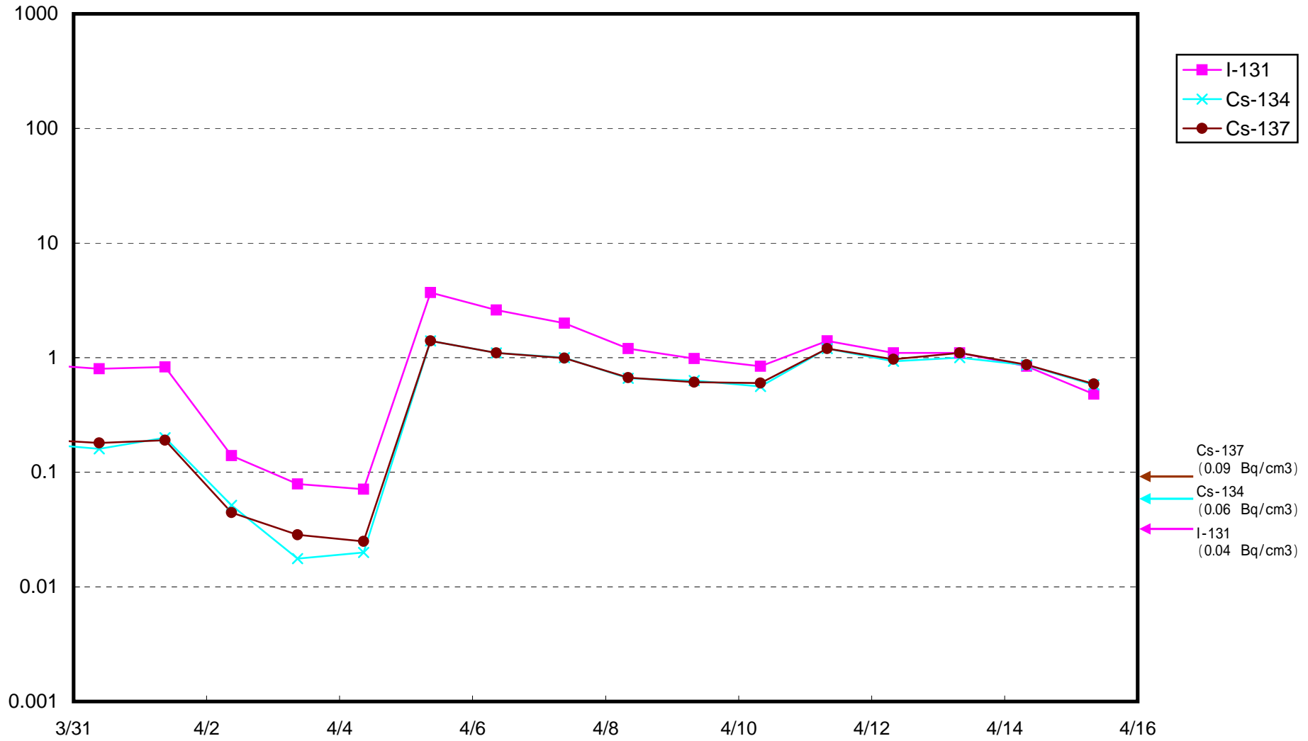
Radioactivity Density of Seawater at Iwasawa Shore at 2F ( B q / c m 3 )
