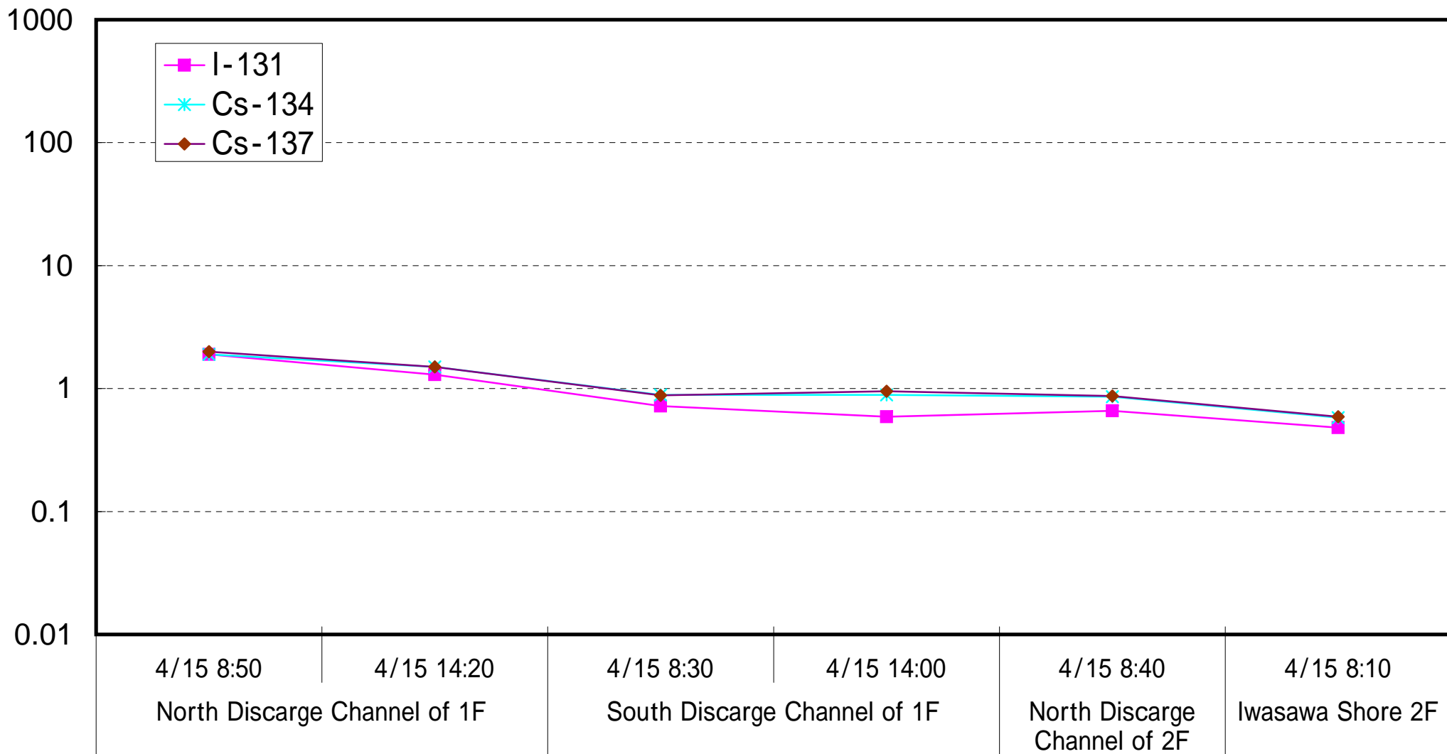
Radioactivity Density of Seawater ( B q / c m3 )
