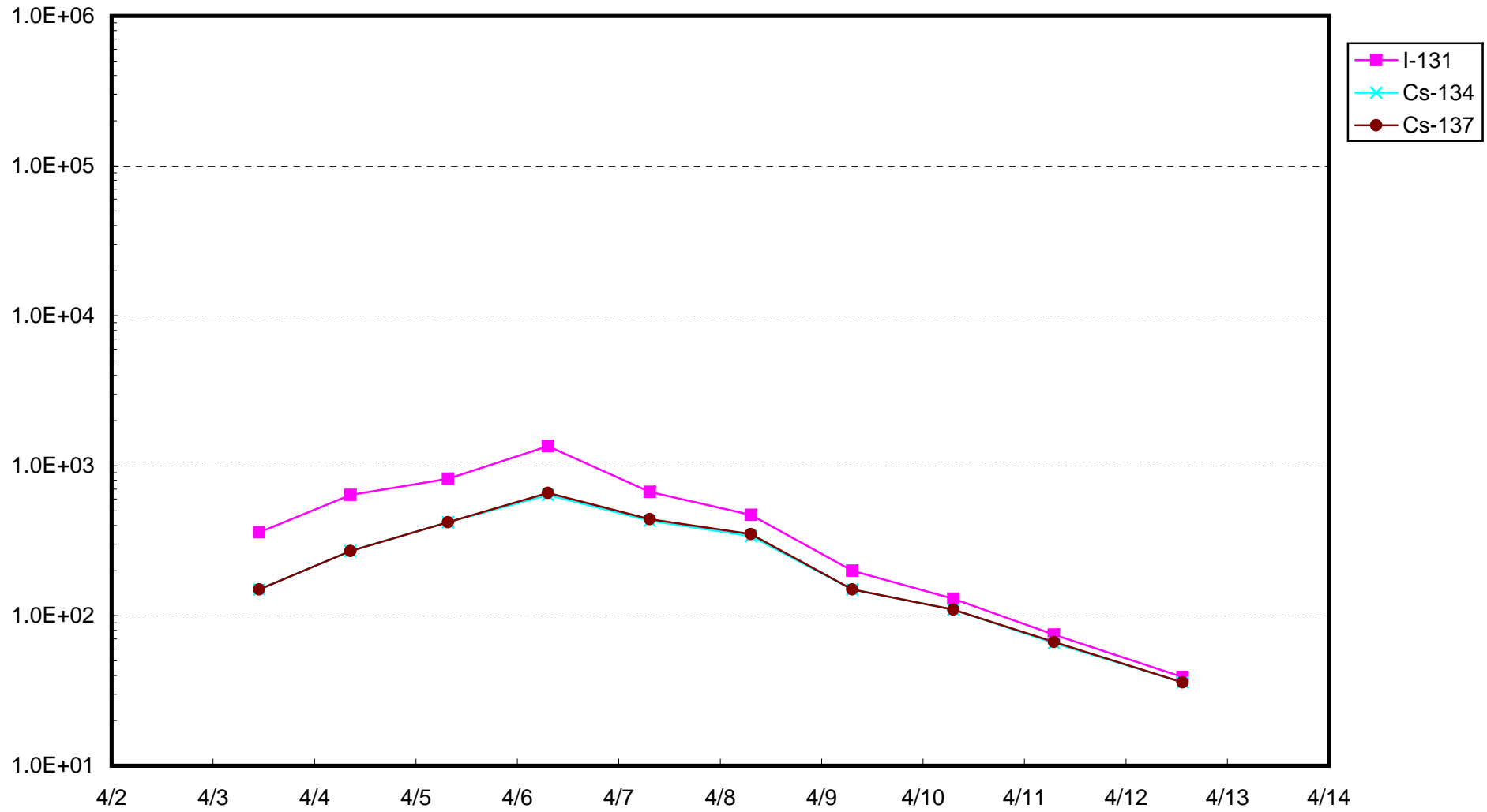
Radioactivity density of seawater at the quay of Fukushima Daiichi Nuclear Power Station (Bq/cm 3 )
