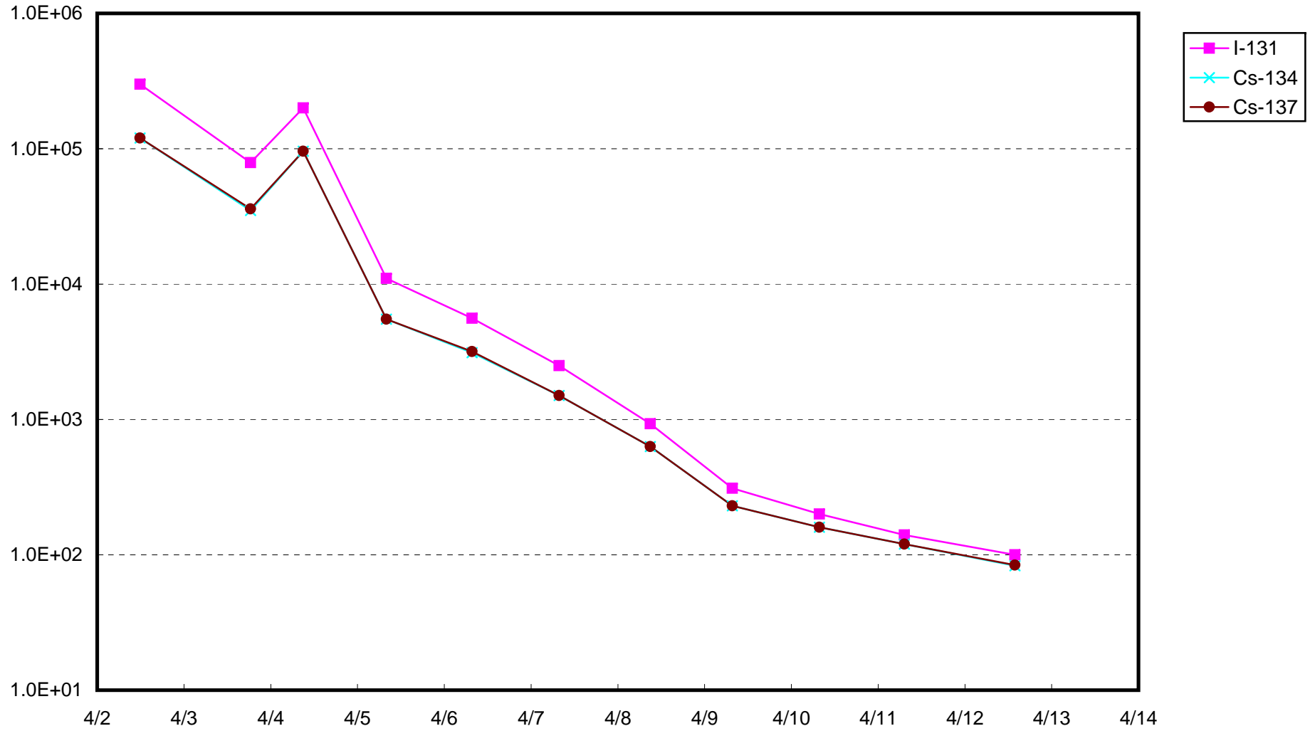
Radioactivity density of seawater at the bar screen of Fukushima Daiichi Nuclear Power Station Unit 2 (Bq/cm 3 )
