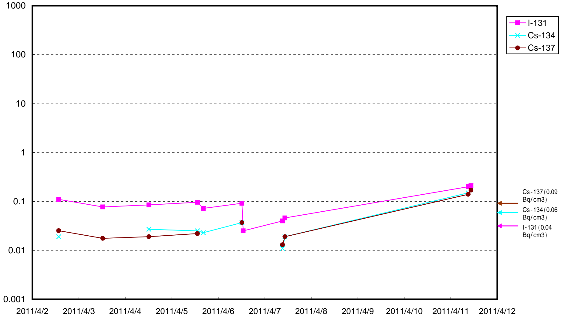
Radioactivity Density of Seawater around 15km off the coast of 2F s property (Bq/ cm3)
