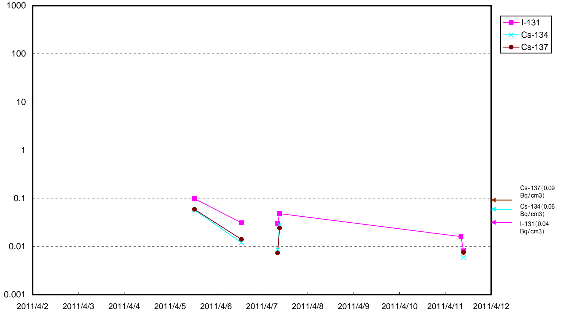
Radioactivity Density of Seawater around 15km off the coast of Hirono Town (Bq/ cm3)
