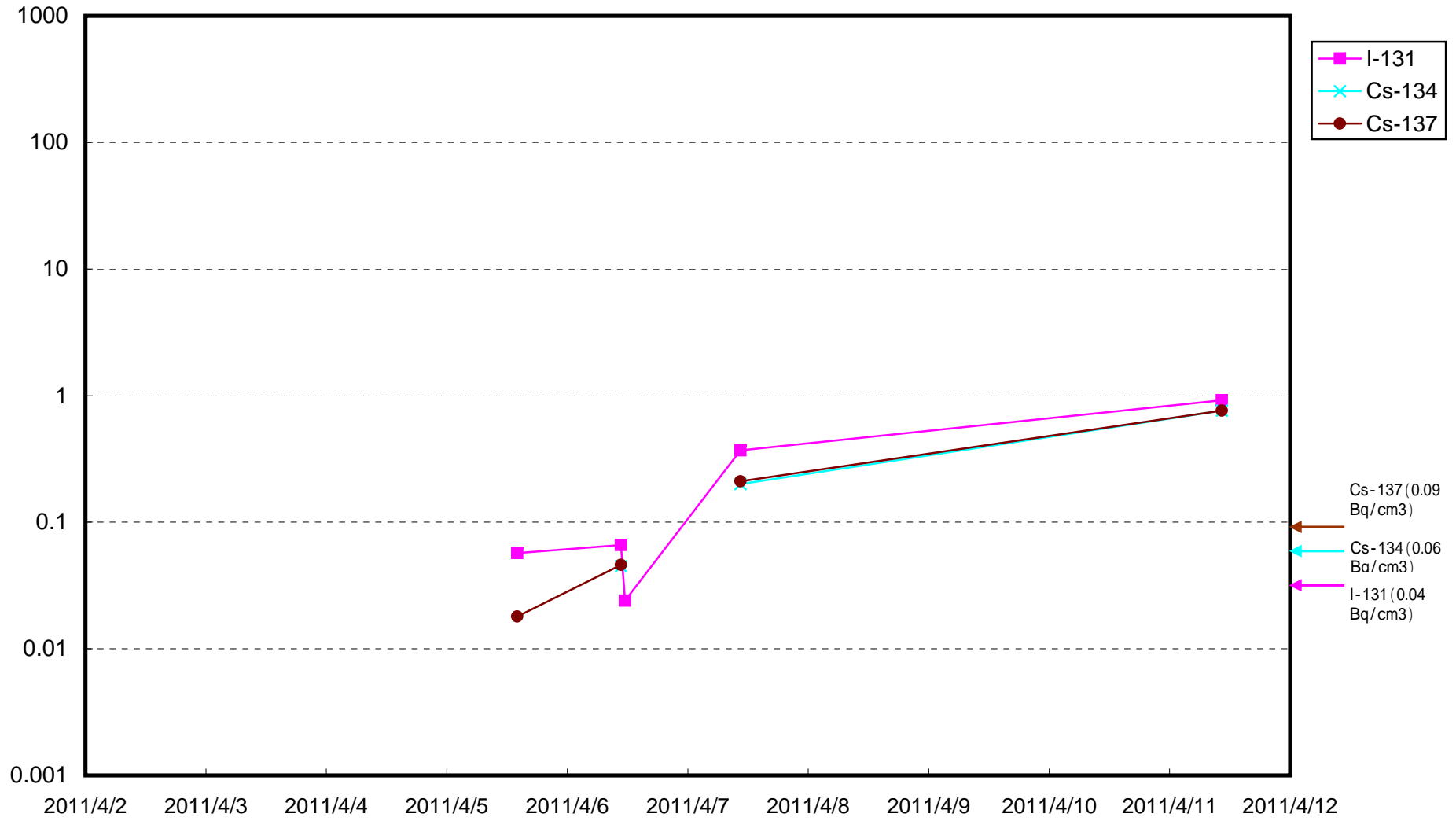
Radioactivity Density of Seawater around 15km off the coast of Minami Soma city (Bq/ cm 3 )
