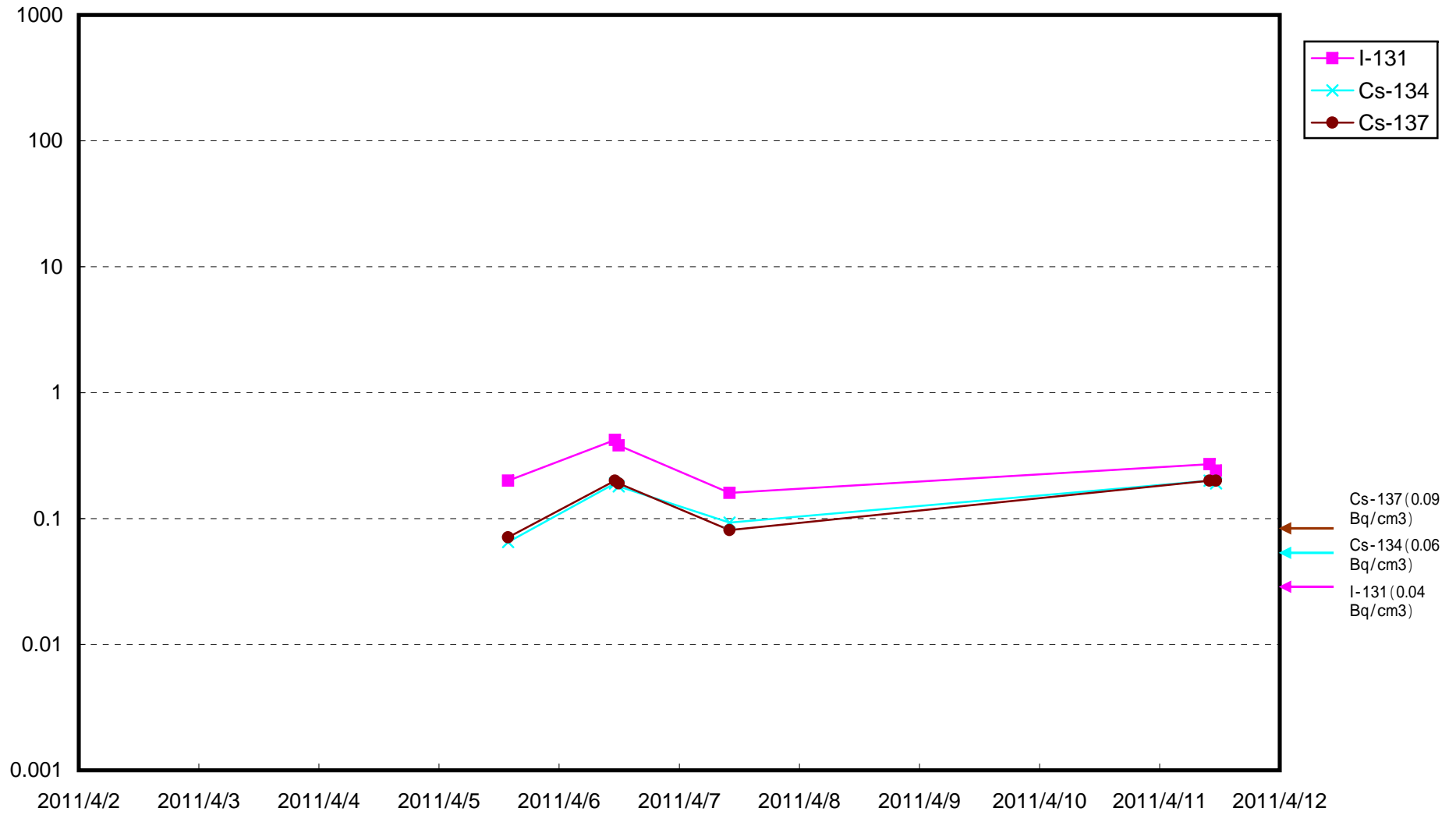
Radioactivity Density of Seawater around 15km off the coast of Ukedogawa River (Bq/ cm3)
