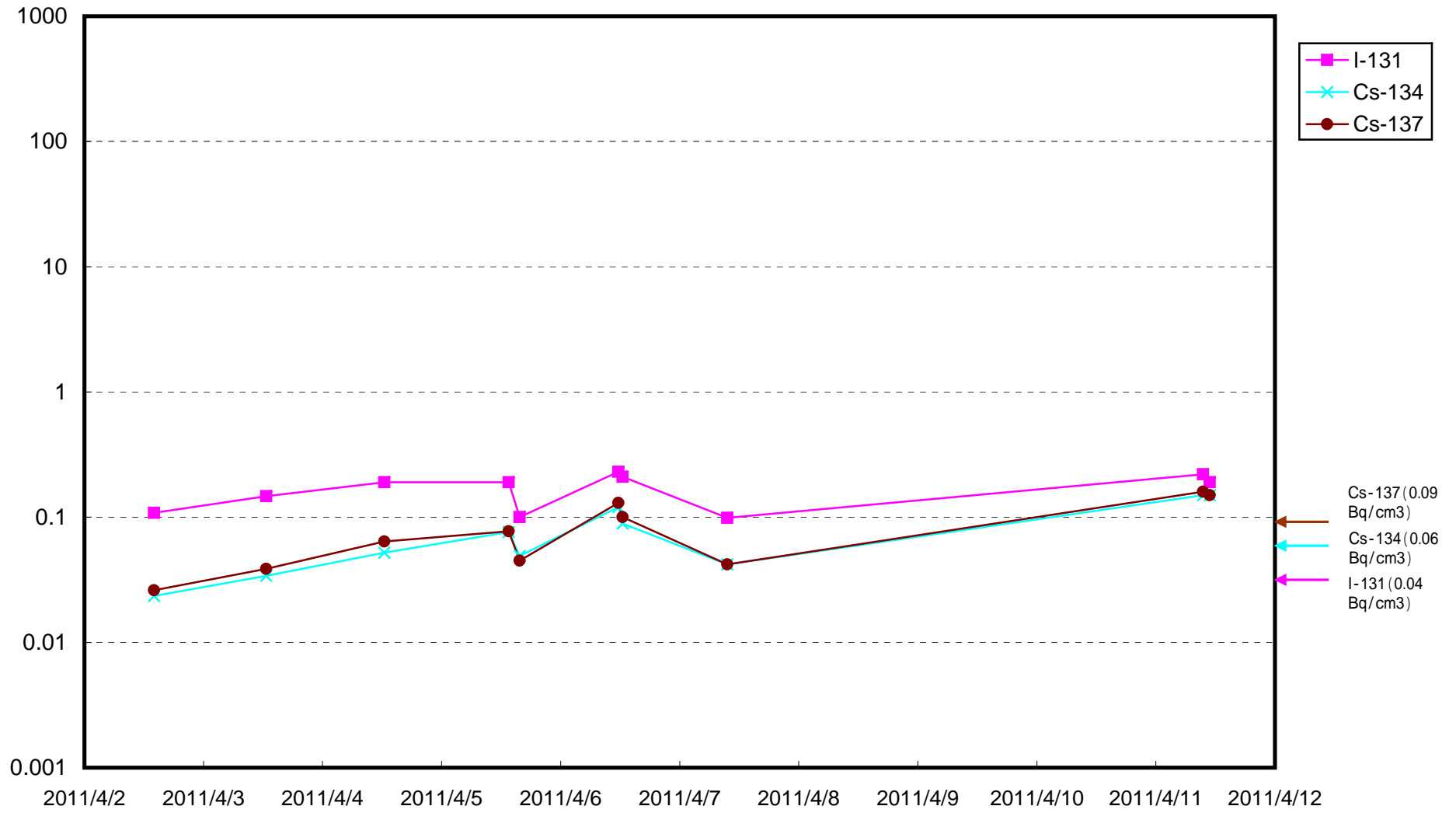
Radioactivity Density of Seawater around 15km off the coast of 1F s property (Bq/ cm3)
