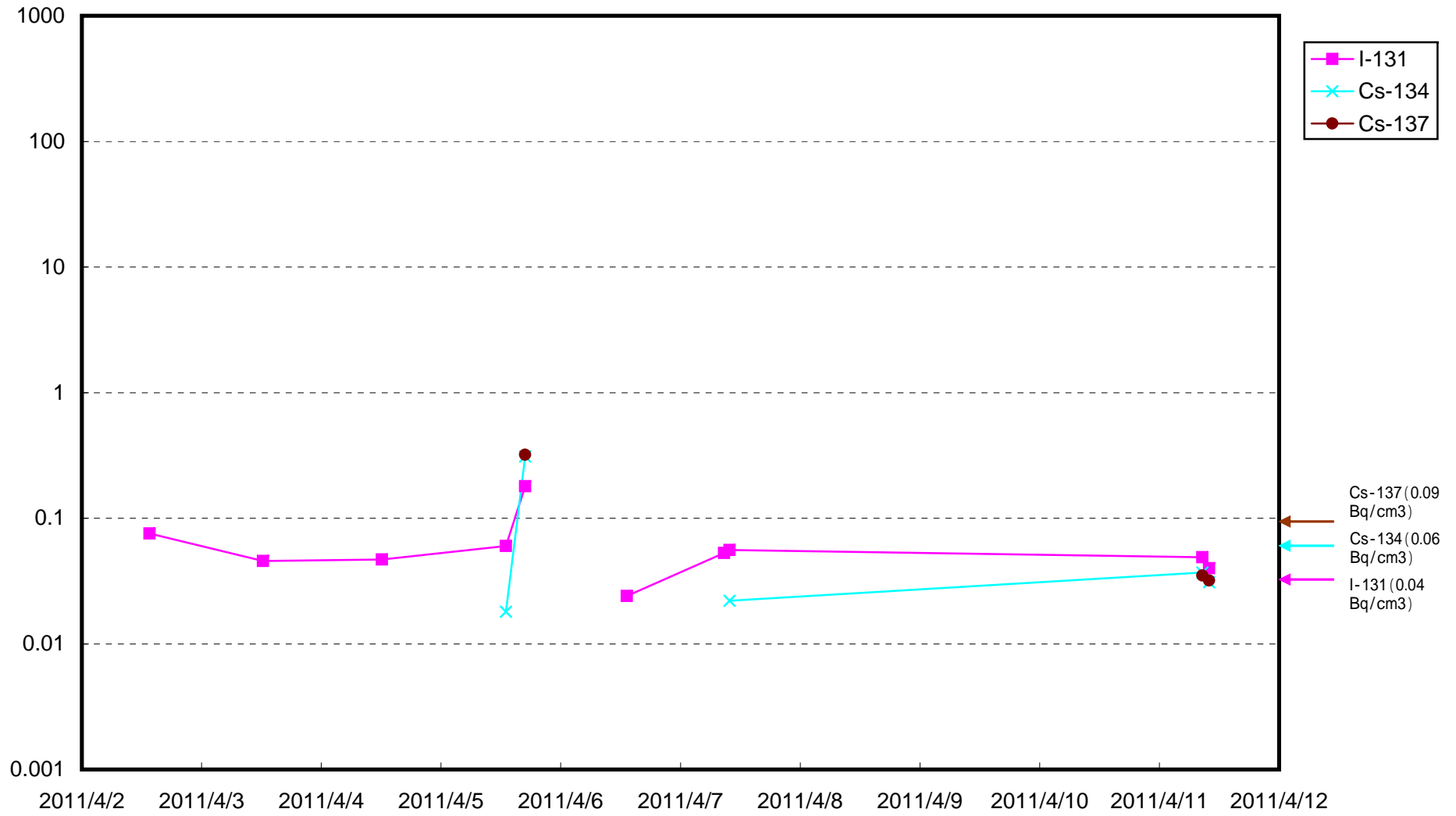
Radioactivity Density of Seawater around 15km off the coast of lawasawa Shore (Bq/ cm3)
