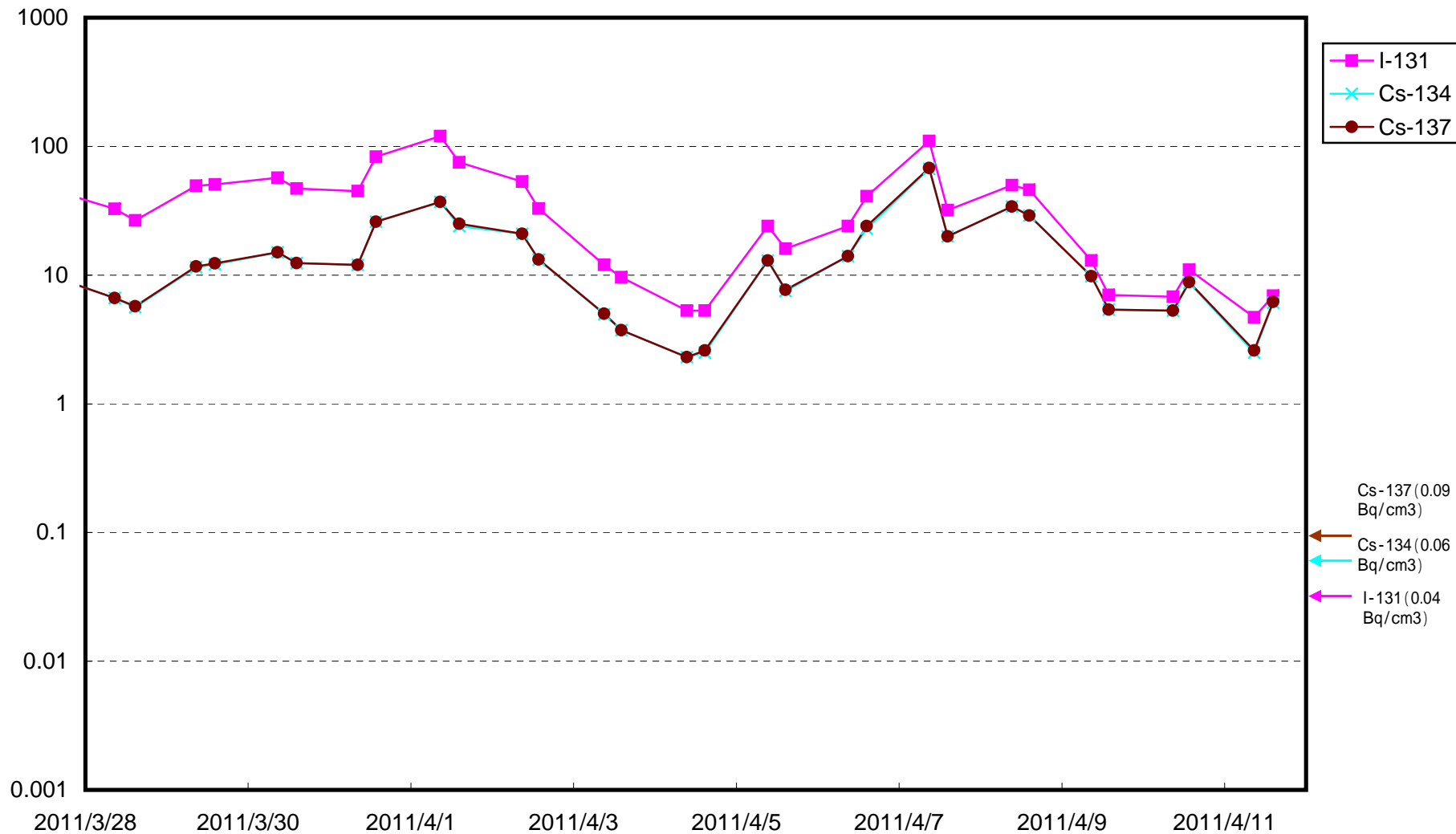
Radioactivity Density of Seawater at North of 1F 5 - 6 Discharge Channel (approx. 30 m north of 5-6u discharge channel) (Bq/cm 3 )
