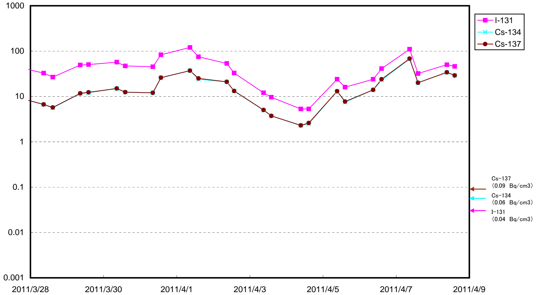
Radioactivity Density of Seawater at North of 1F 5 - 6 Discharge Canal (approx. 30 m north of 5-6u discharge canal) (Bq/cm 3 )
