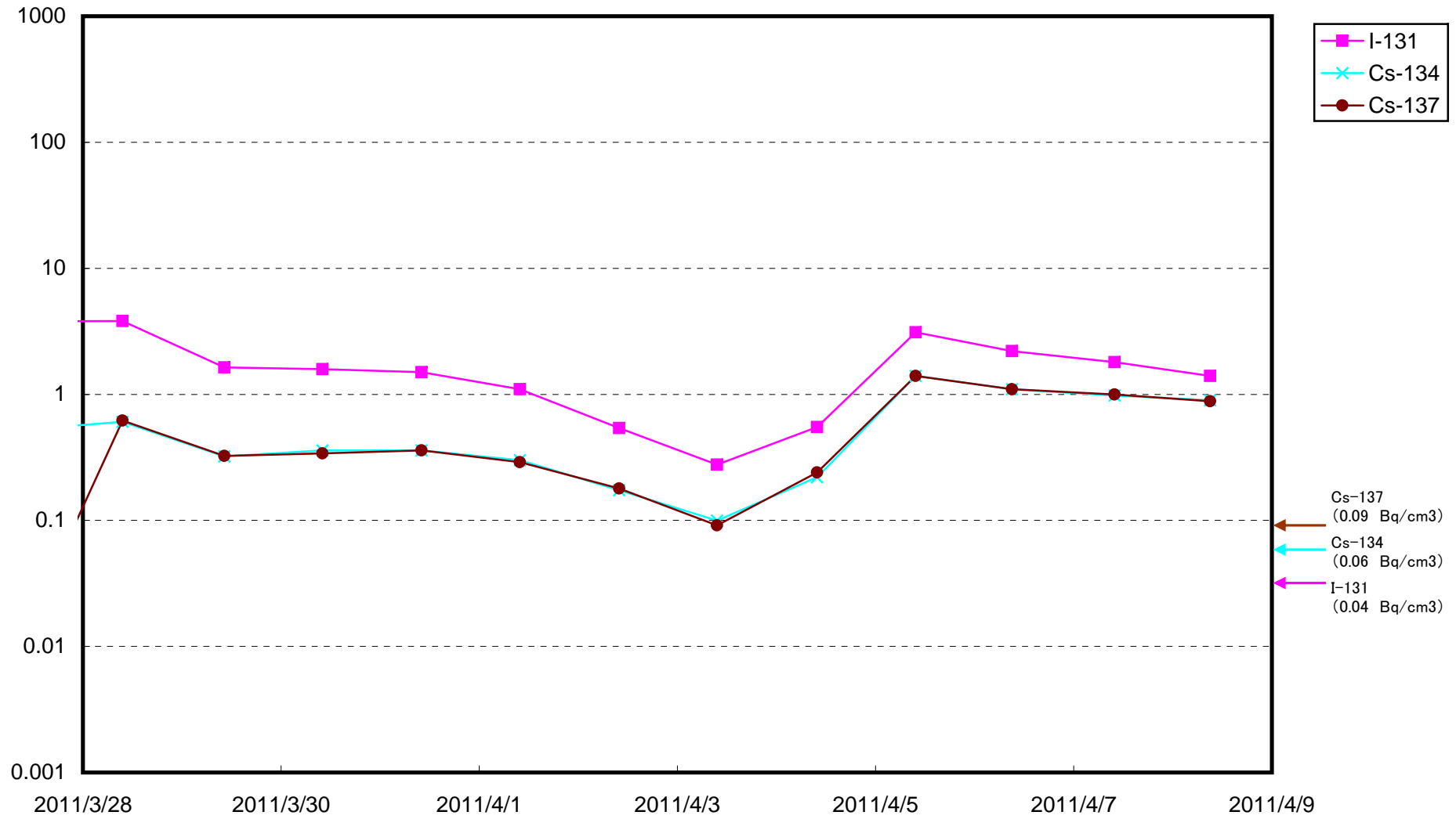
Radioactivity Density of Seawater at North Discharge Canal of 2F (Bq/cm 3 )
