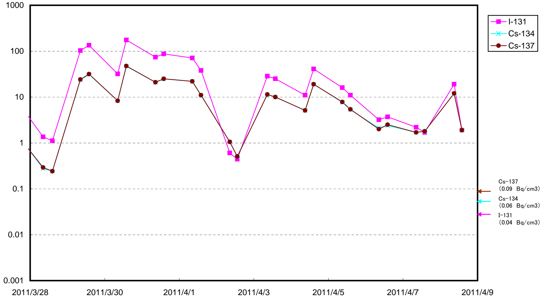
Radioactivity Density of Seawater at South Discharge Canal of 1F (Bq/cm 3 )
