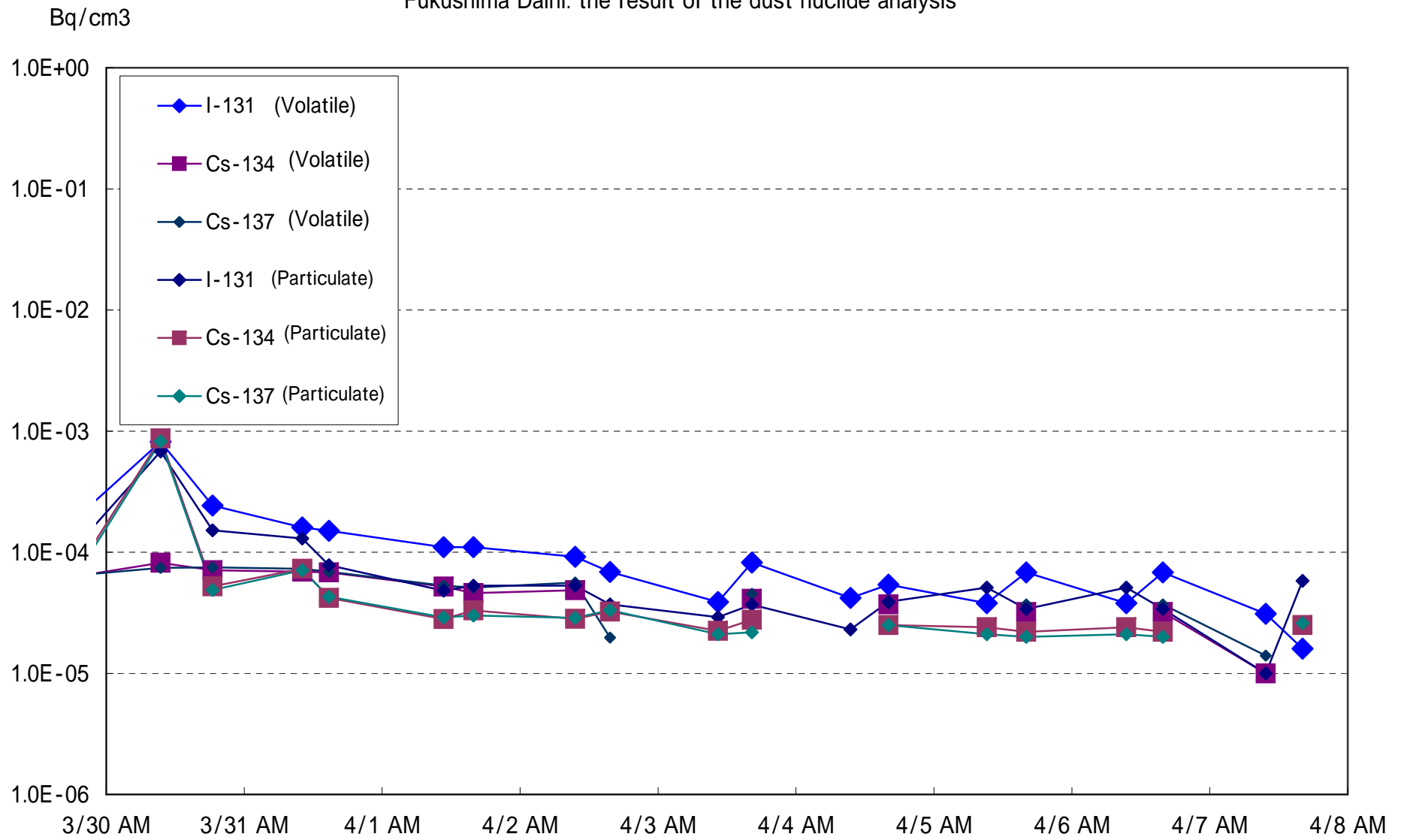
Fukushima Daini: the result of the dust nuclide analysis
