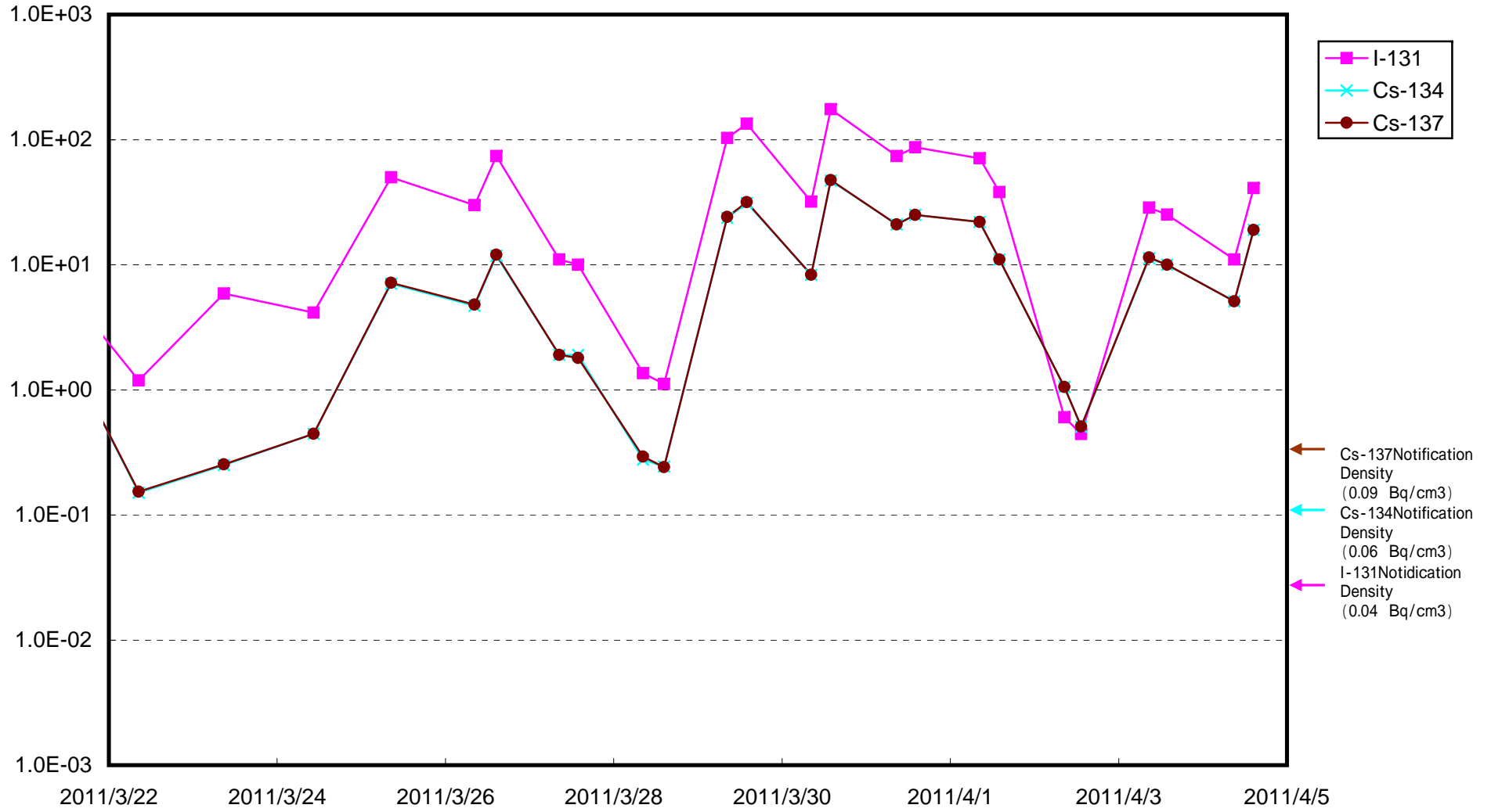
Radioactive Density at 1F 5 ~ 6 Discharge Canal (South) (Bq/cm 3 )
