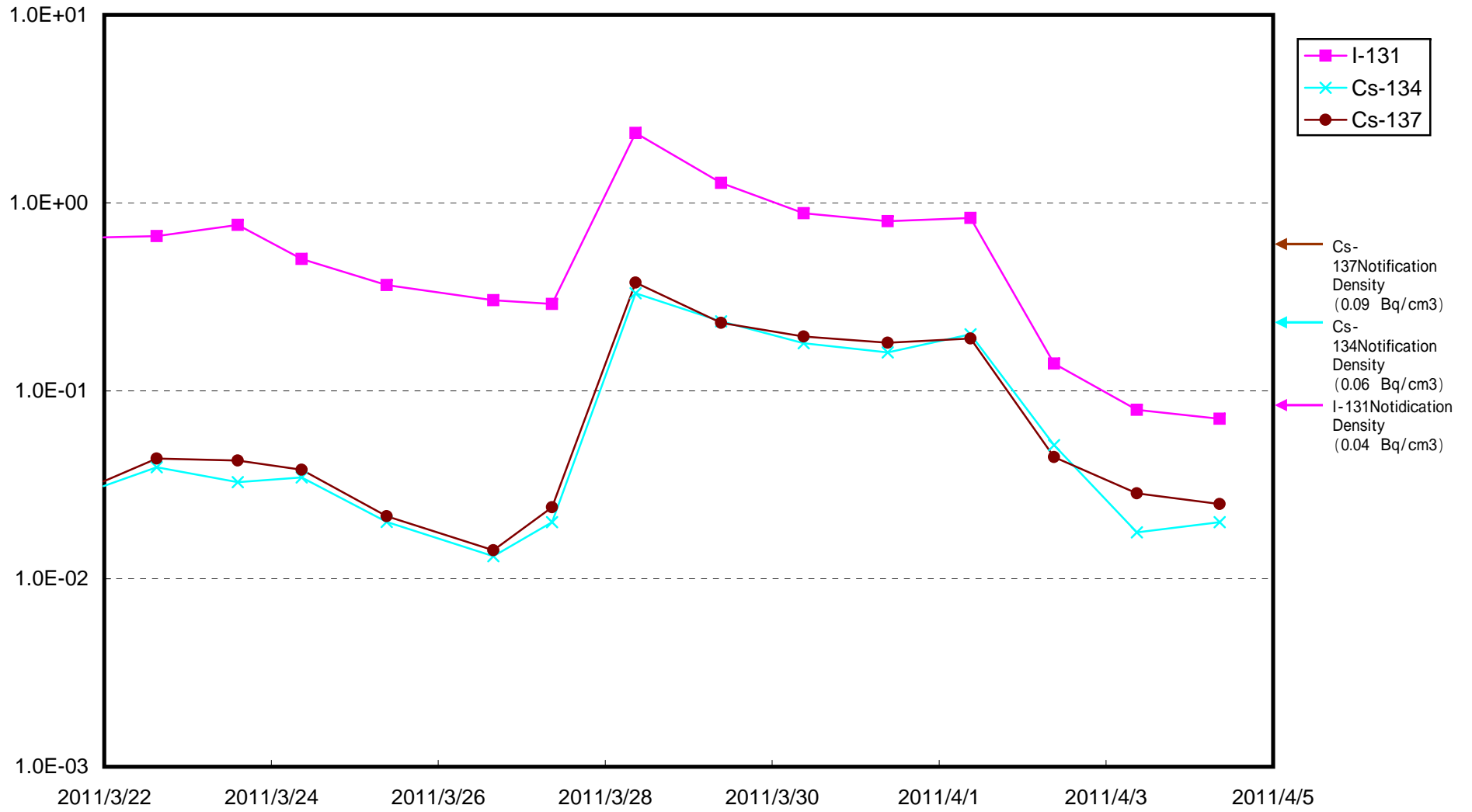
Radioactive Density at Iwasawa Shore at 2F (Bq/cm 3 )
