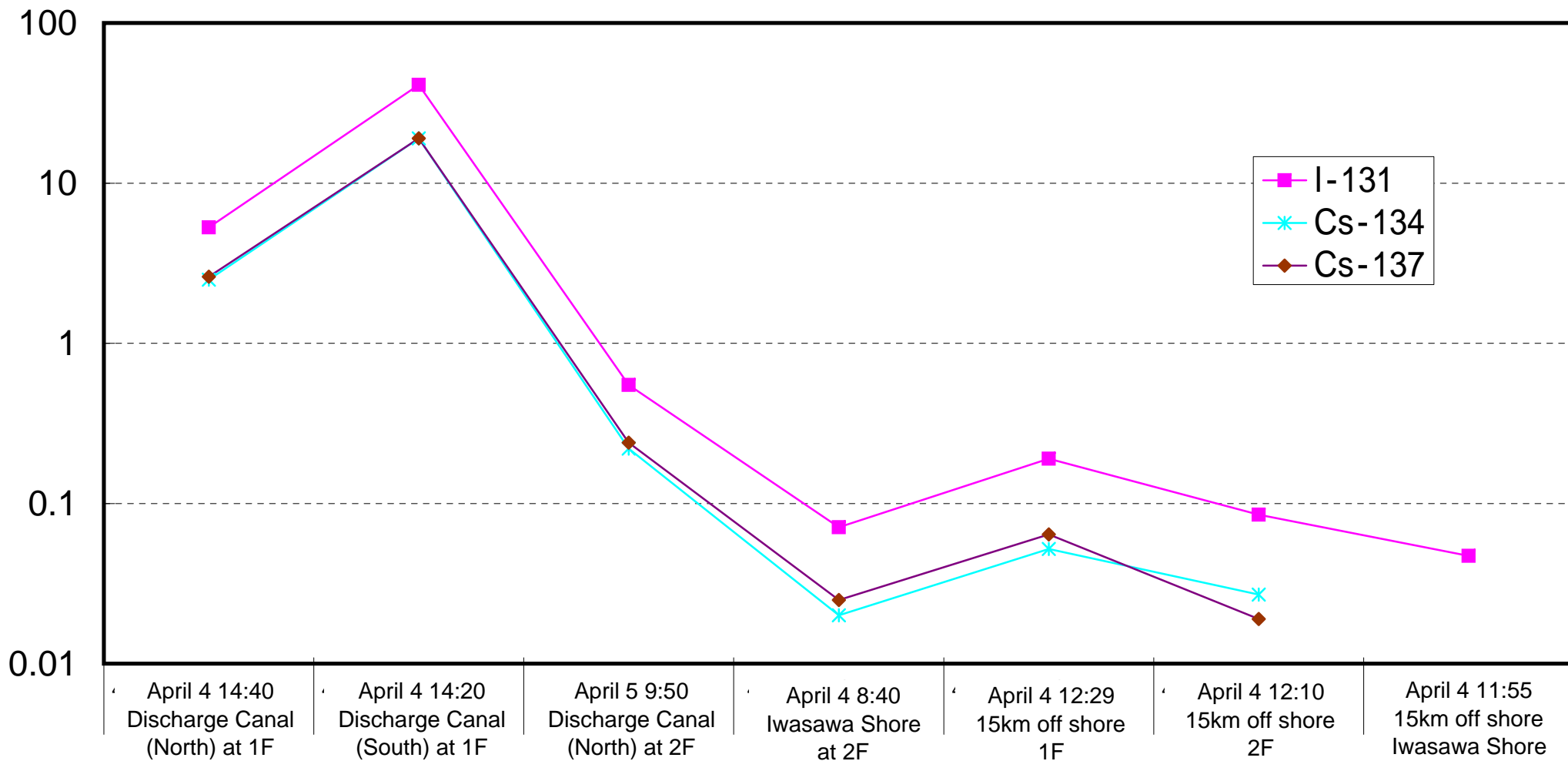
Radioactivity Density of Seawater ( B q / c m3 )
