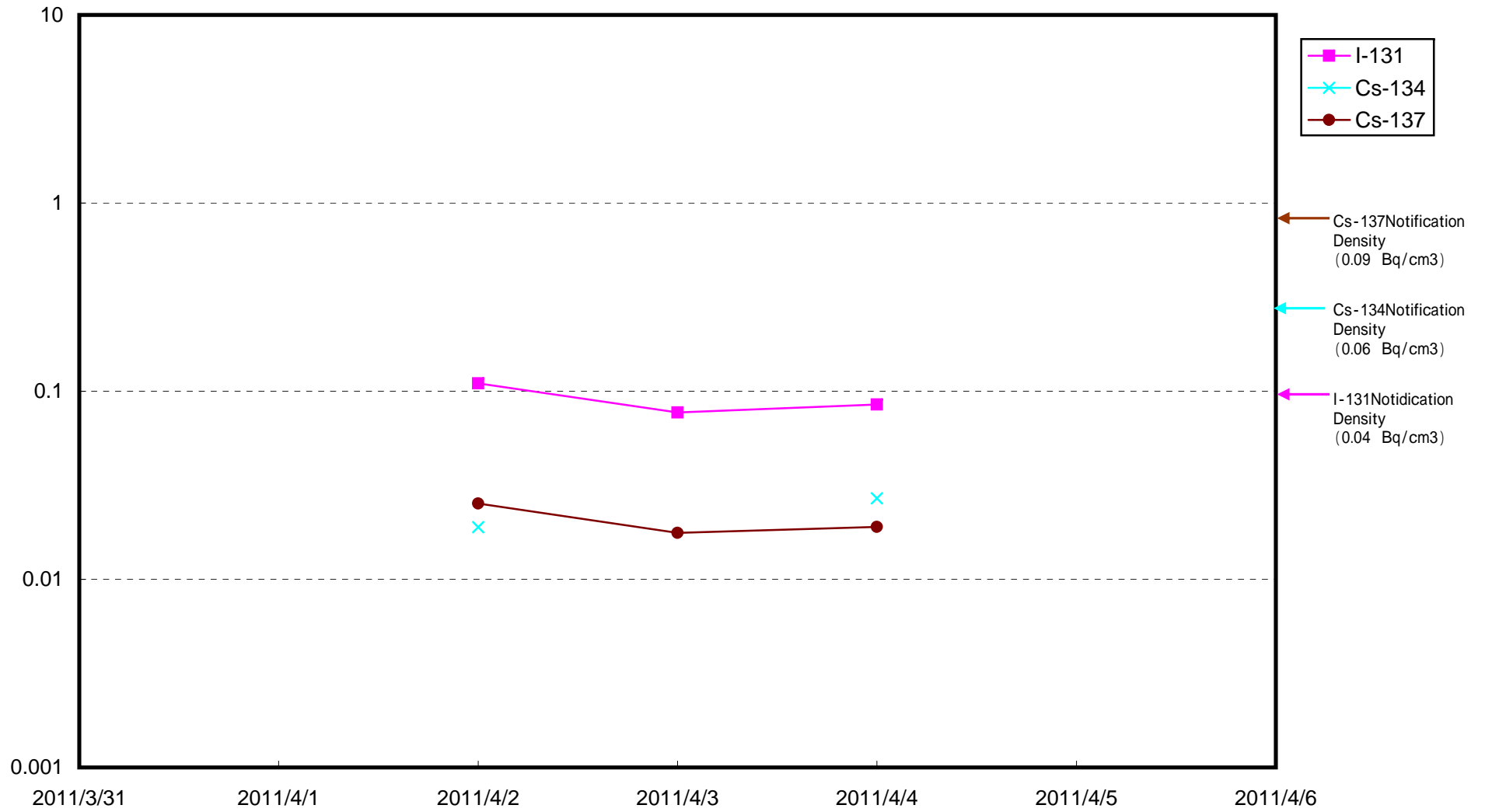
Radioactive Density at 15km offshore of Fukushima Daiichi Nuclear Power Station (Bq/cm 3 )
