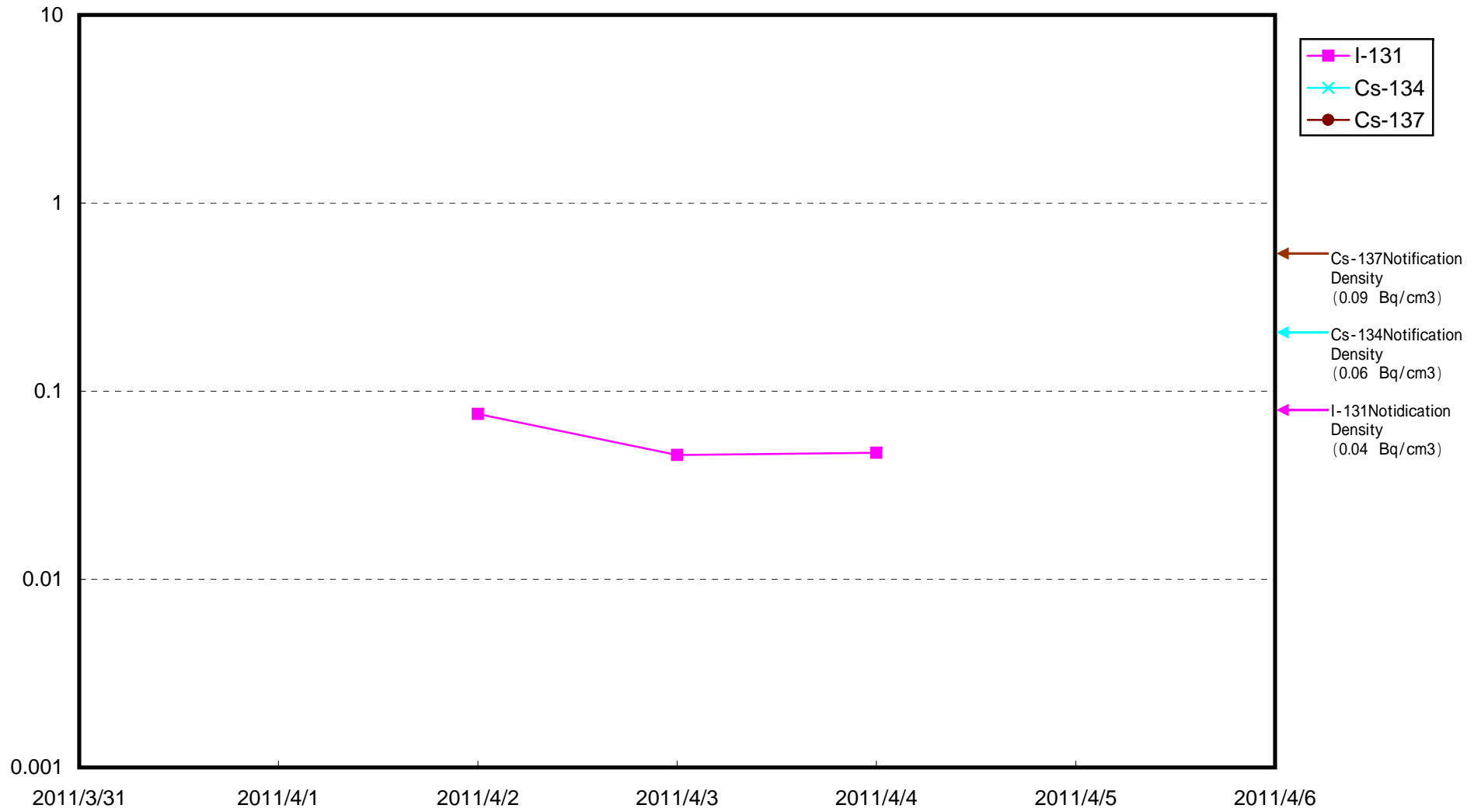
Radioactive Density at 15km offshore of Iwasawa Shore at 2F (Bq/cm 3 )
