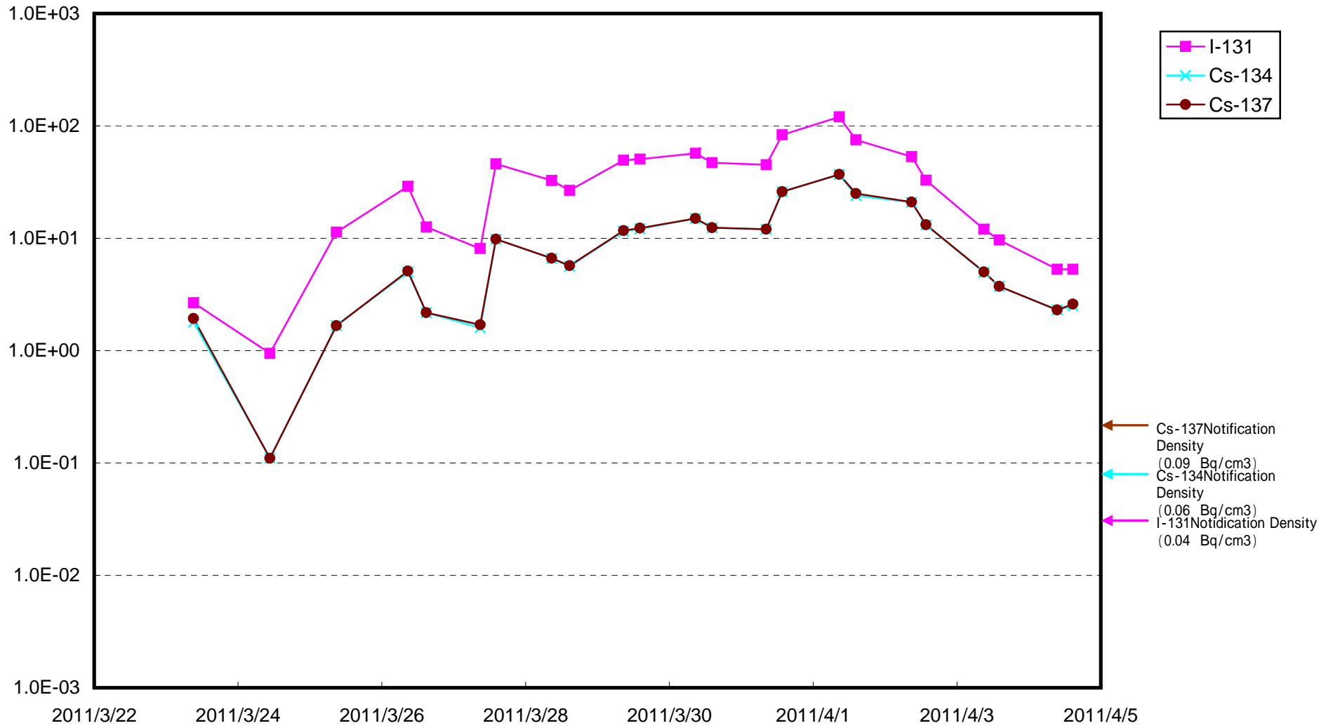
Radioactive Density at 1F 5 ~ 6 Discharge Canal (North) (approx. 30km north of 5 ~ 6u discharge canal) (Bq/cm 3 )
