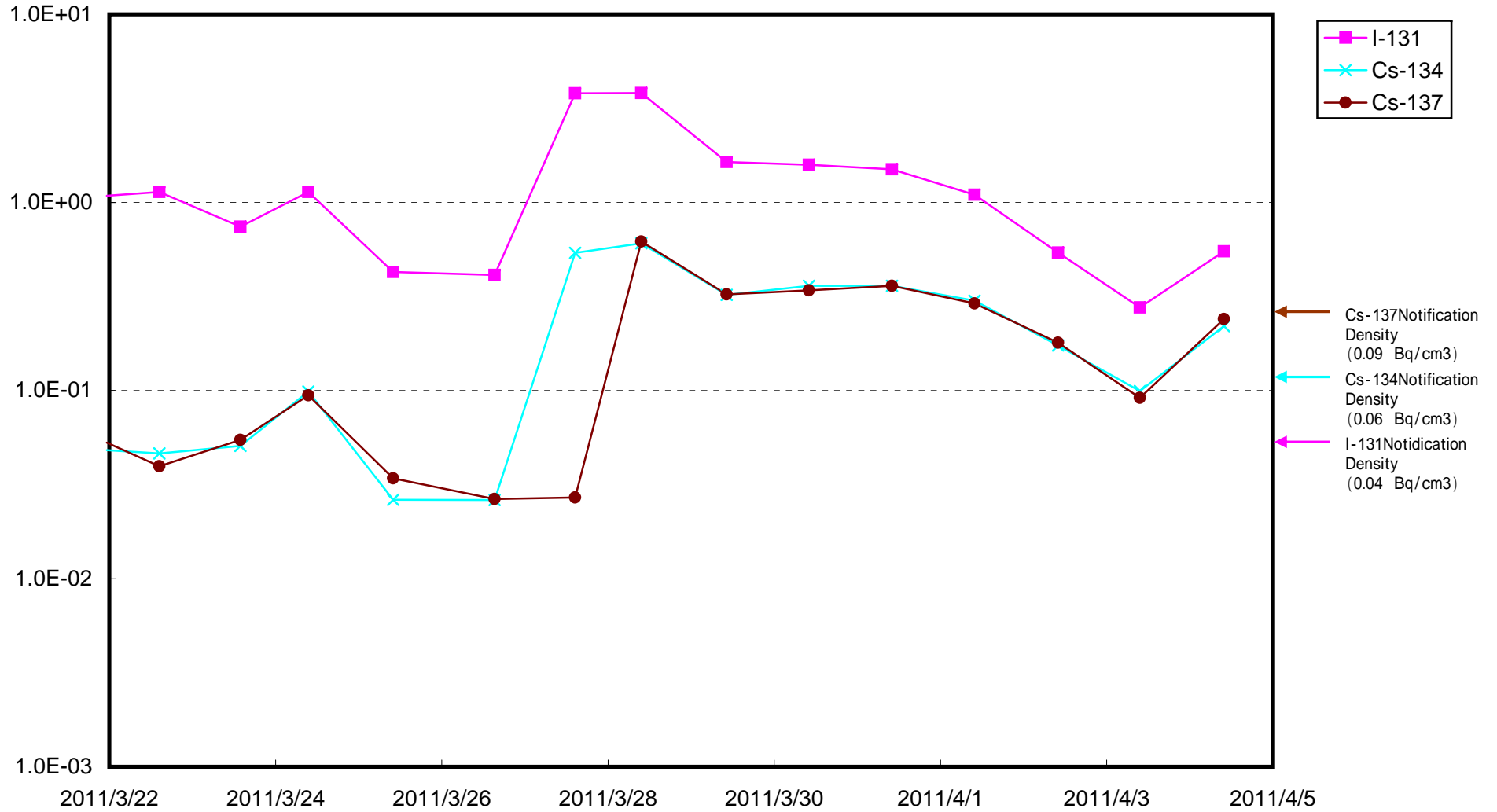
Radioactive Density at 2F Discharge Canal (North) (Bq/cm 3 )
