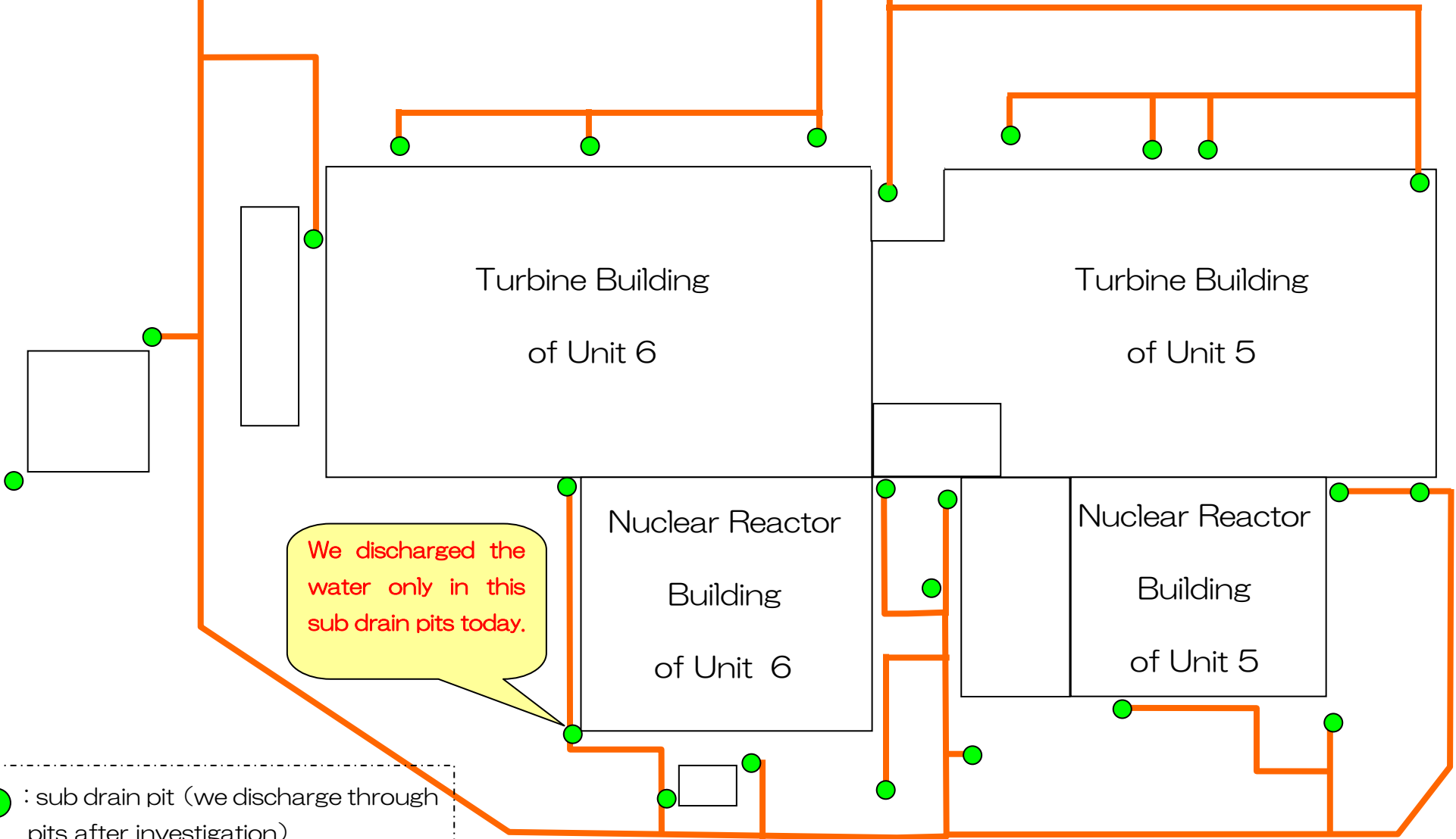
Outline of discharge routes of Unit 5 and 6
