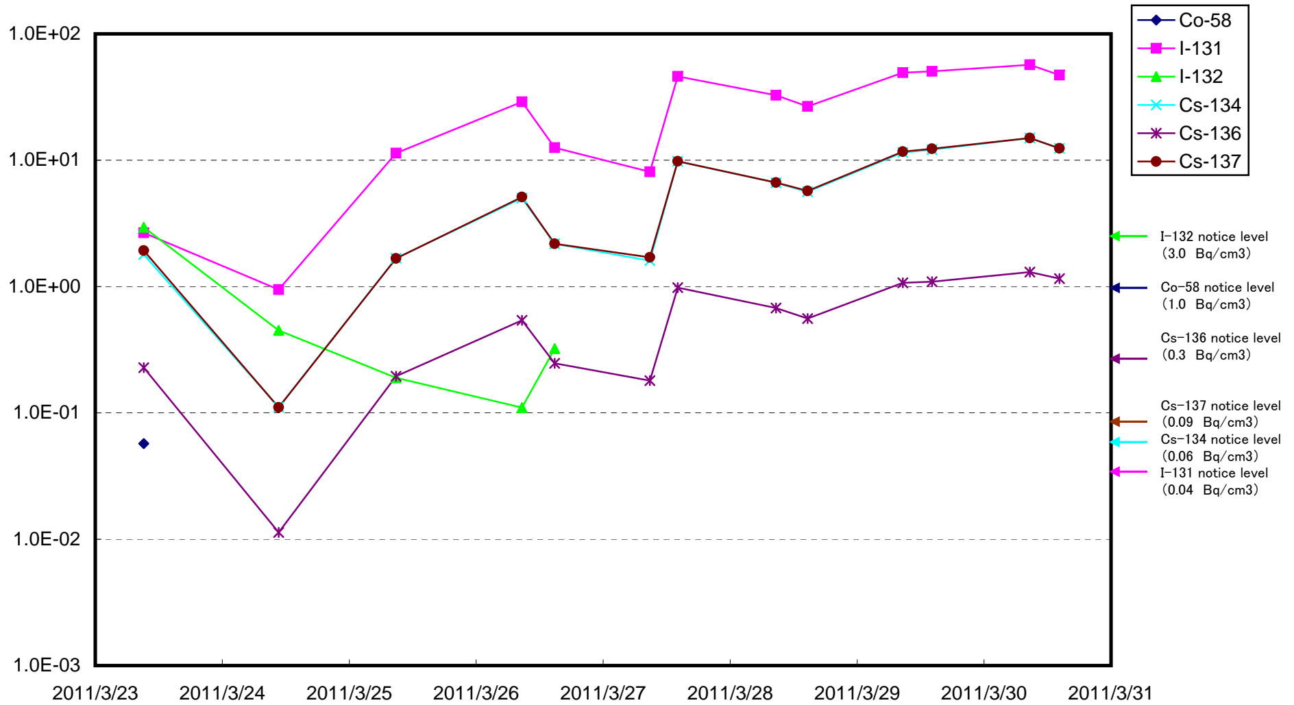
Radioactivity Density around the discharge canal (north) of Unit 5 and 6 Fukushima Daiichi Nuclear Power Station (approx. 30m north from the discharge canal of Unit 5 and 6) (Bq/cm 3 )
