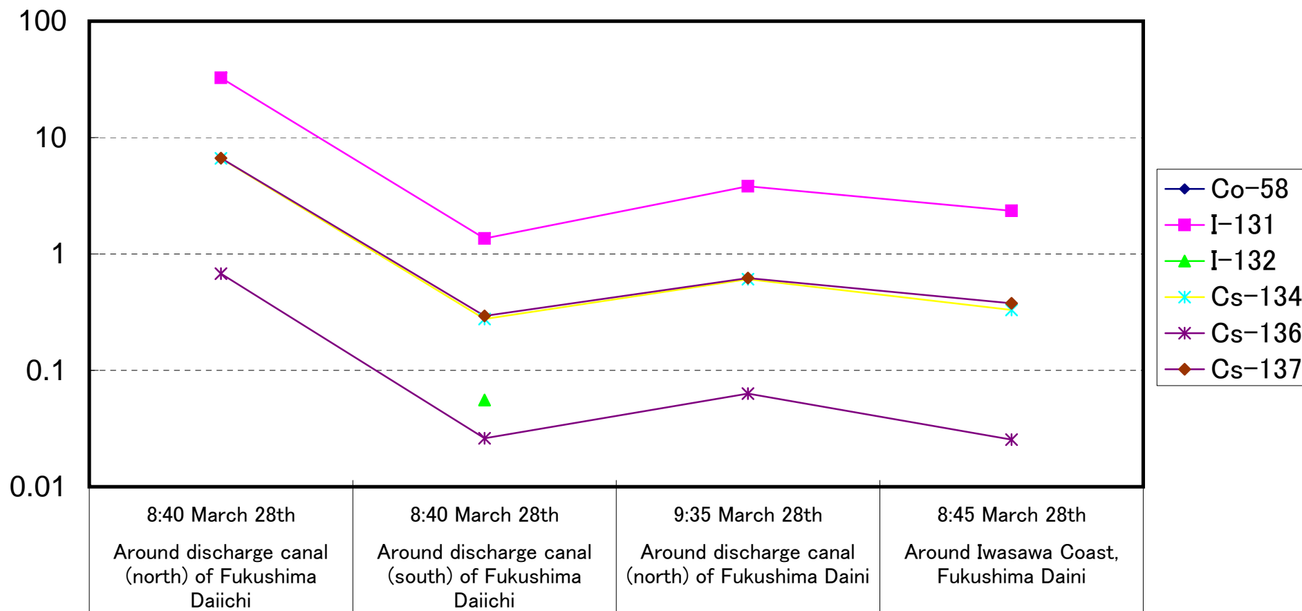
Radioactivity Density of Seawater (Bq/cm 3 )
