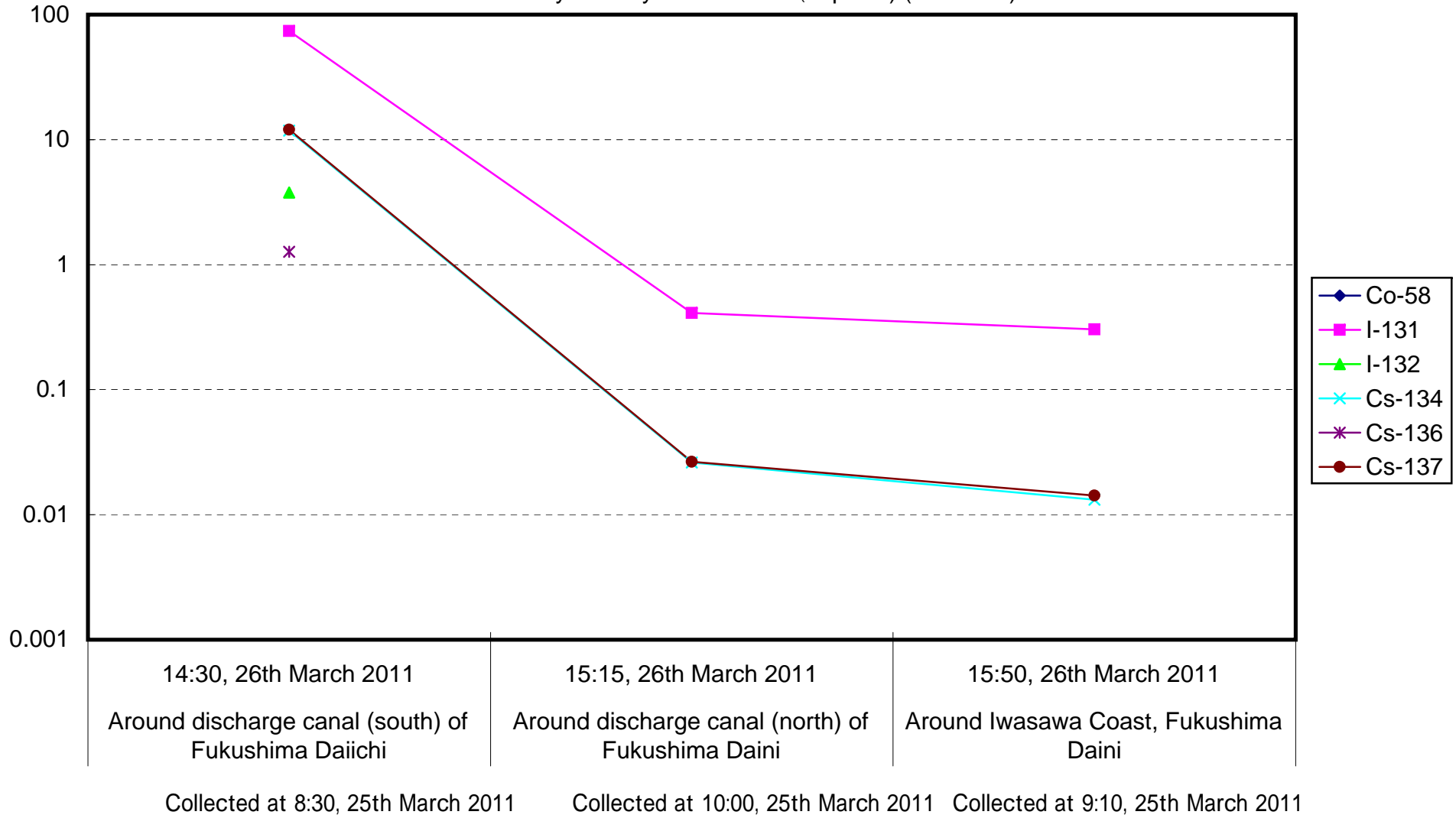
Radioactivity Density of Seawater (Bq/cm 3 ) (H23.3.26)
