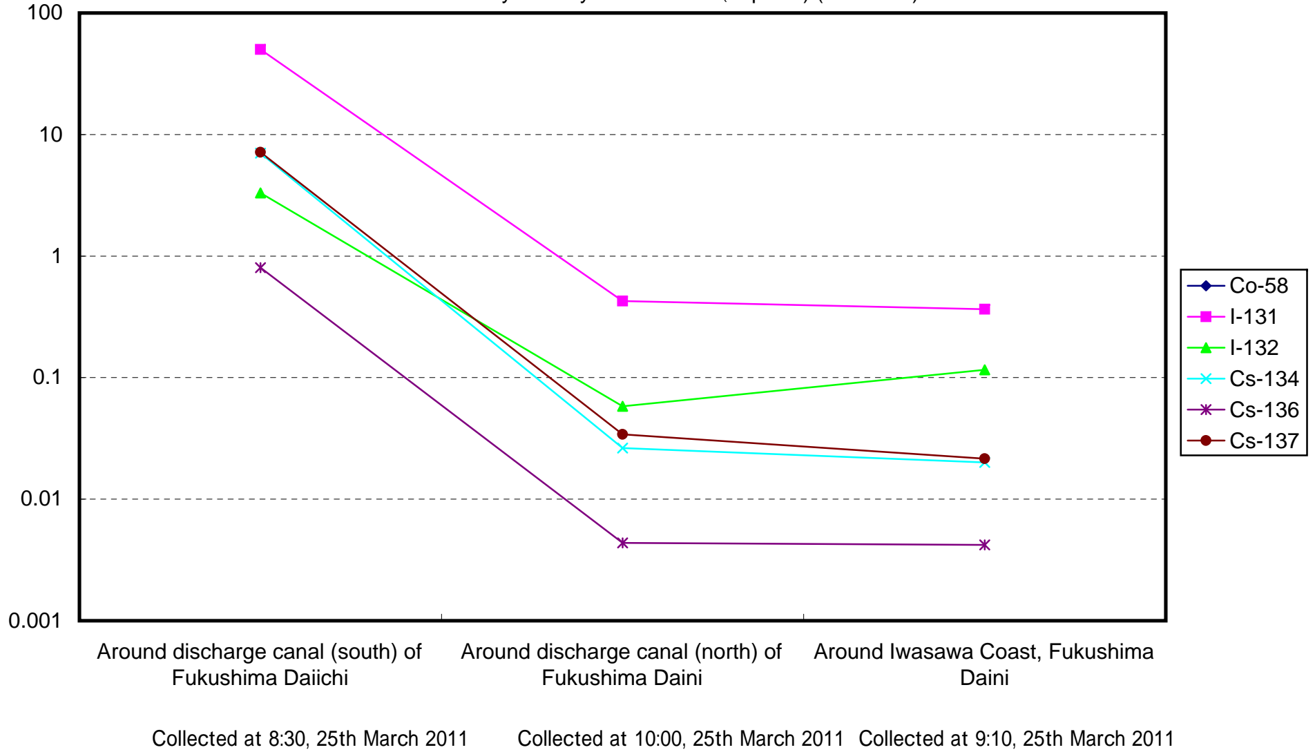
Radioactivity Density of Seawater (Bq/cm 3 ) (H23.3.25)
