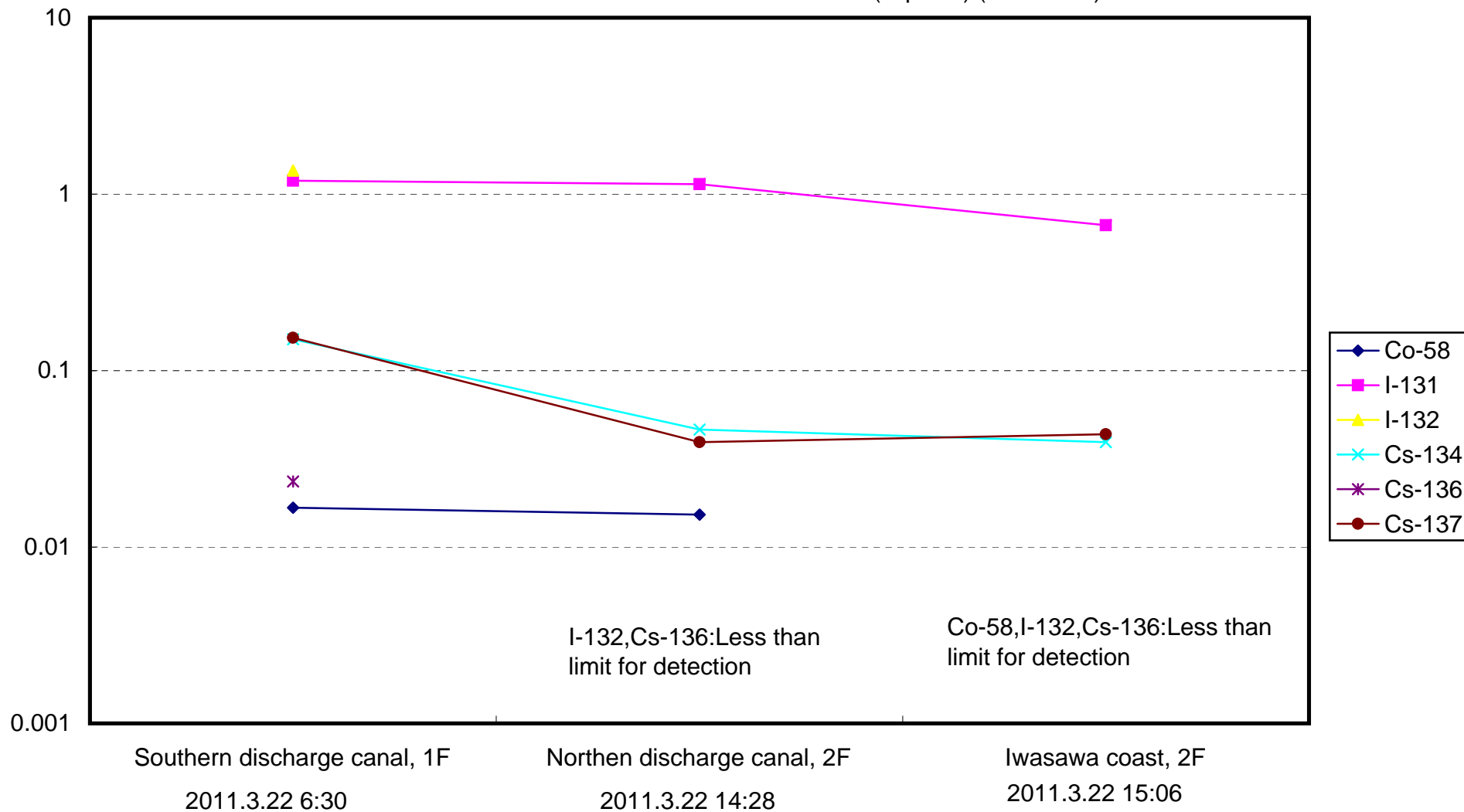
Seawater concentration of radioactive materials(Bq/cm 3 ) (2011.3.22)
