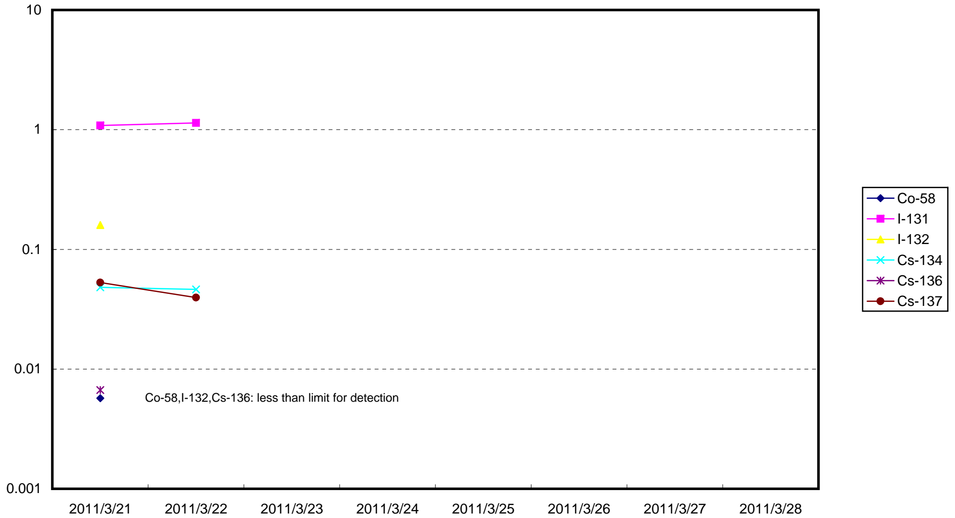
Northern discharge canal of 2F seawater concentration of radioactive materials(Bq/cm 3 )
