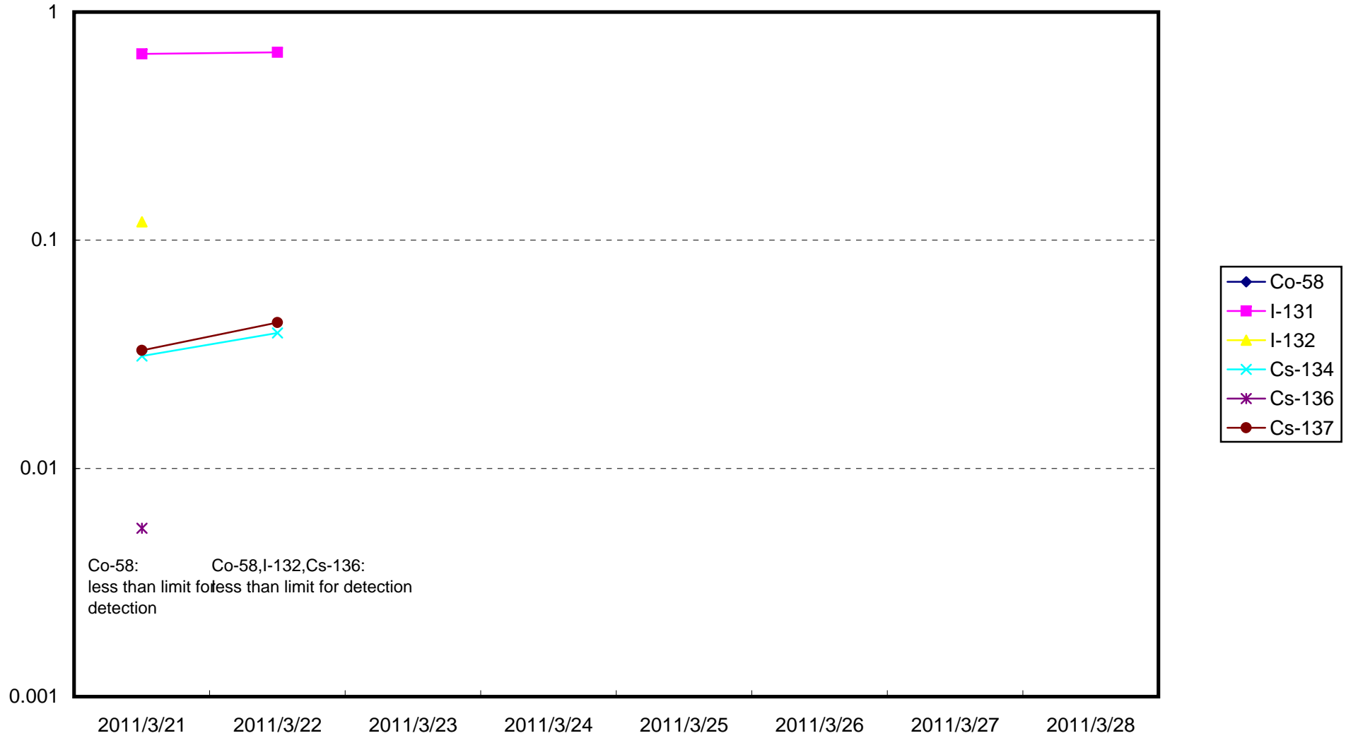
Iwasawa coast of 2F seawater concentration of radioactive materials(Bq/cm3)
