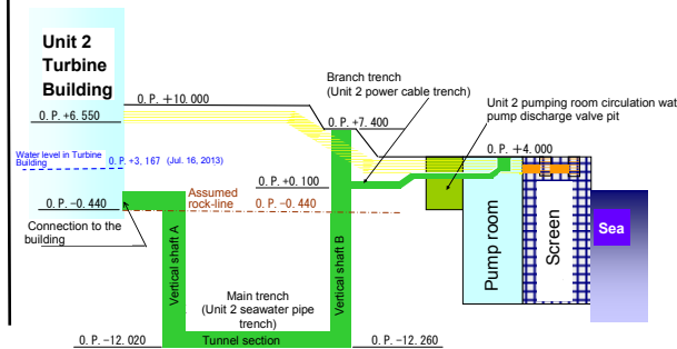
Blocking of the Unit 2 branch trench was completed.
