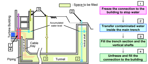
Water stop work of the main trench is scheduled to be started by the end of FY2013.
