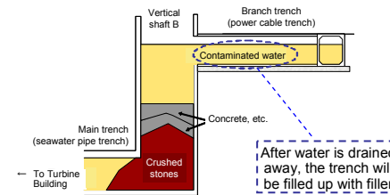
Blocking of the Unit 2 branch trench was completed.
