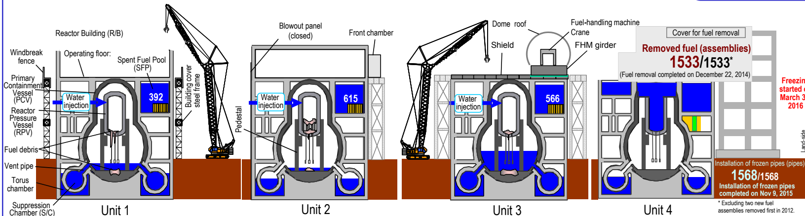
Installation of the fuel removal cover (December 19, 2017)
