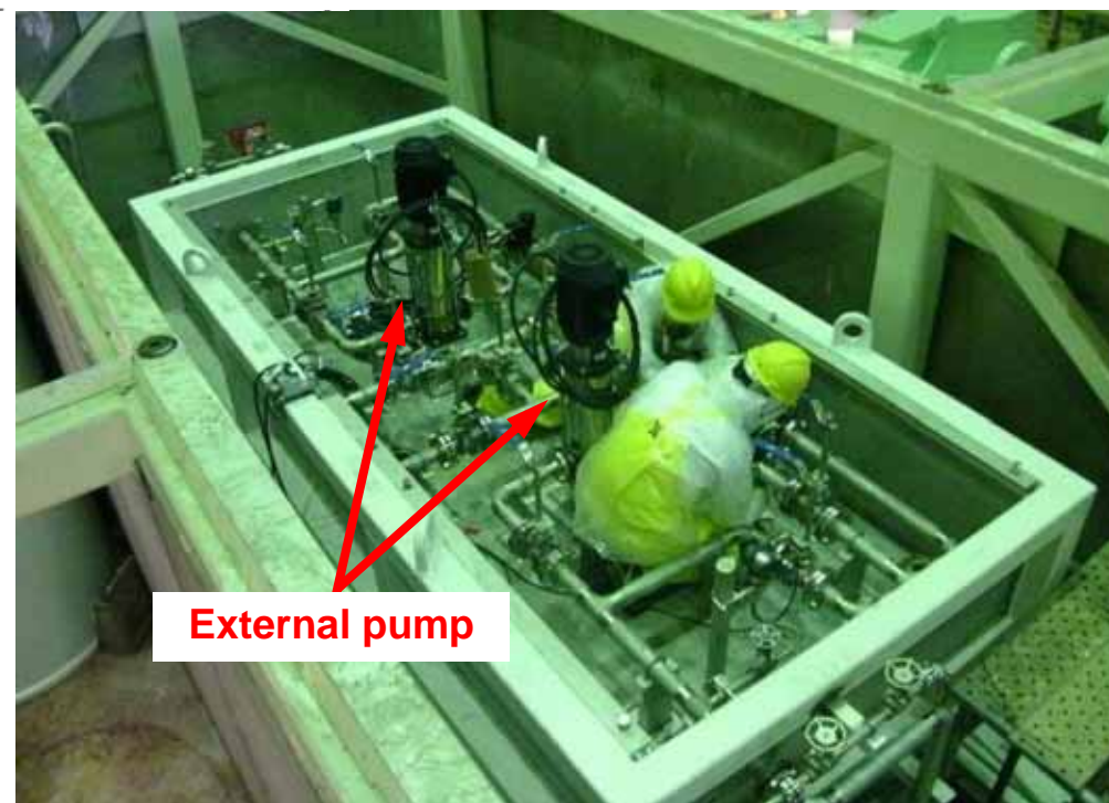
2. Cesium Absorption Apparatus (Pump Skid) (Photo taken by a TEPCO employee on May 31, 2012)
