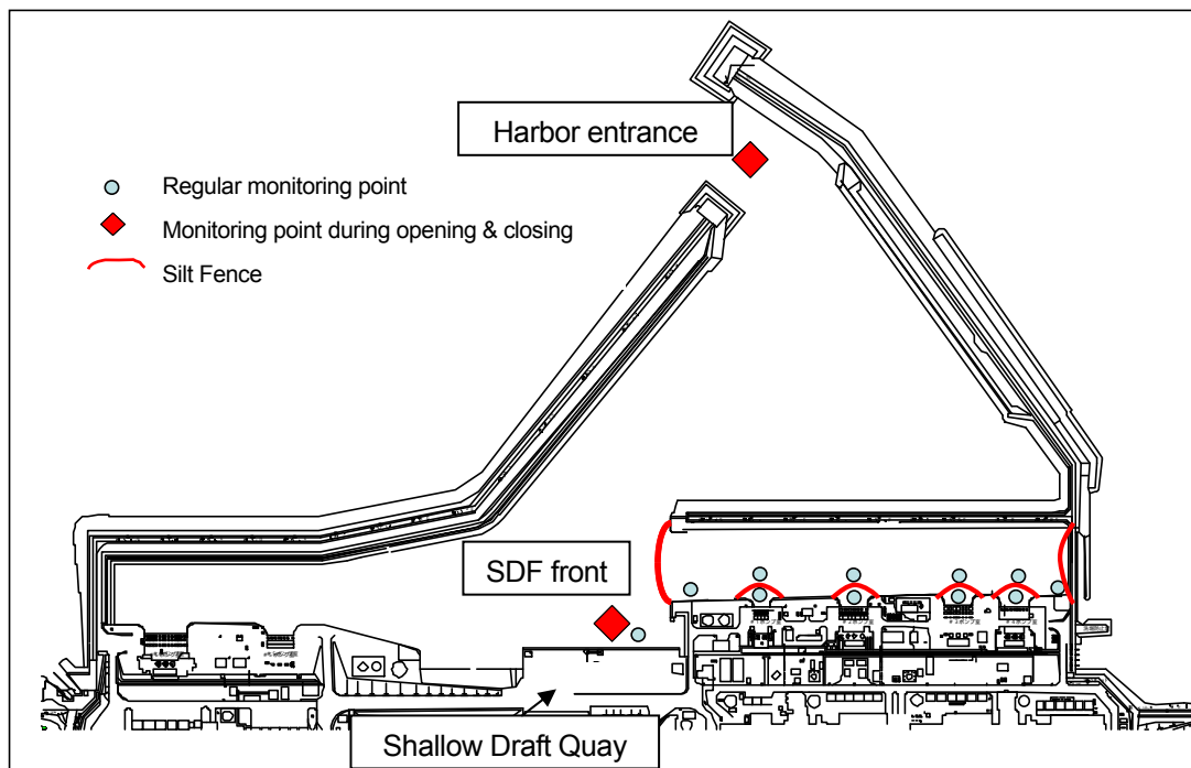
Figure 1: Harbor of Fukushima Daiichi Nuclear Power Station
