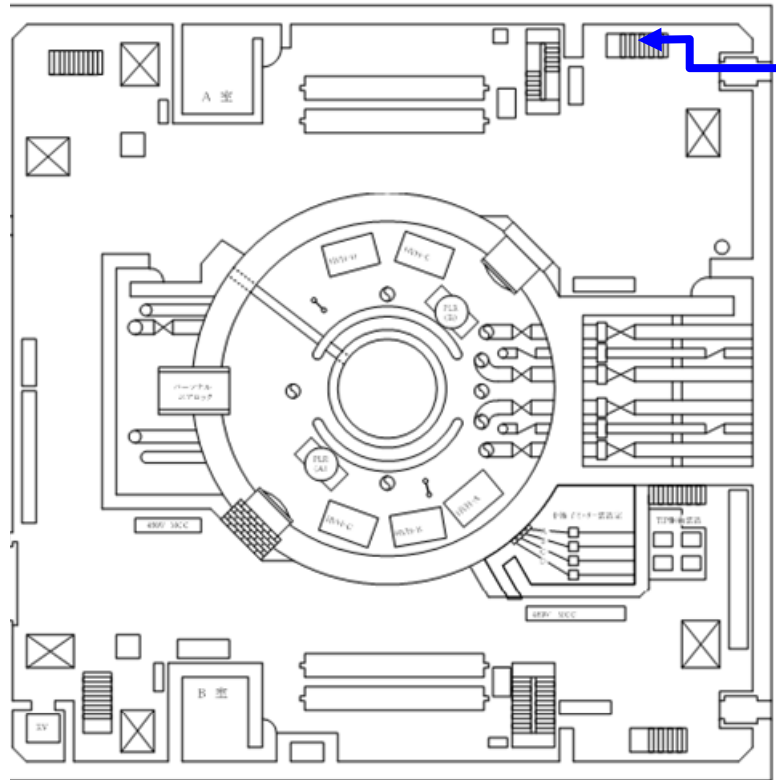
First Floor of the Reactor Building
