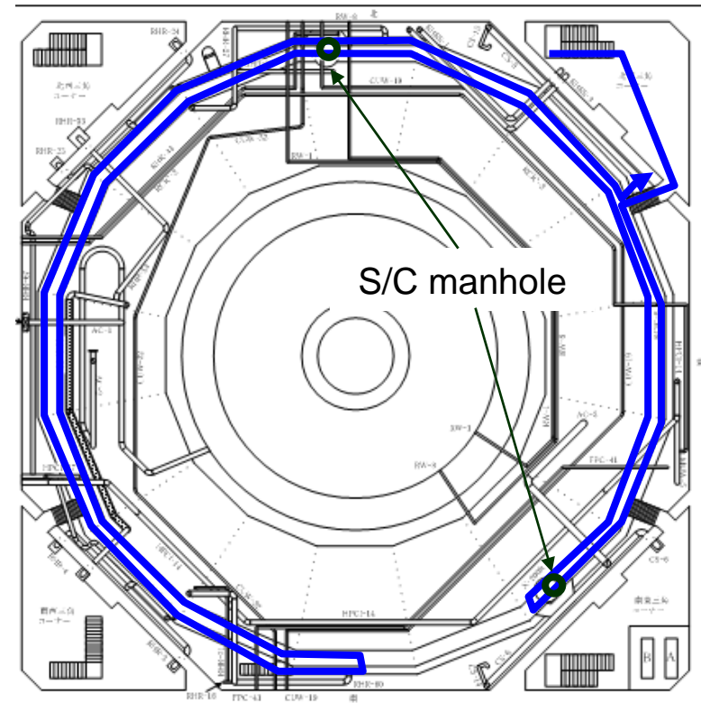
Basement Floor of the Reactor Building
