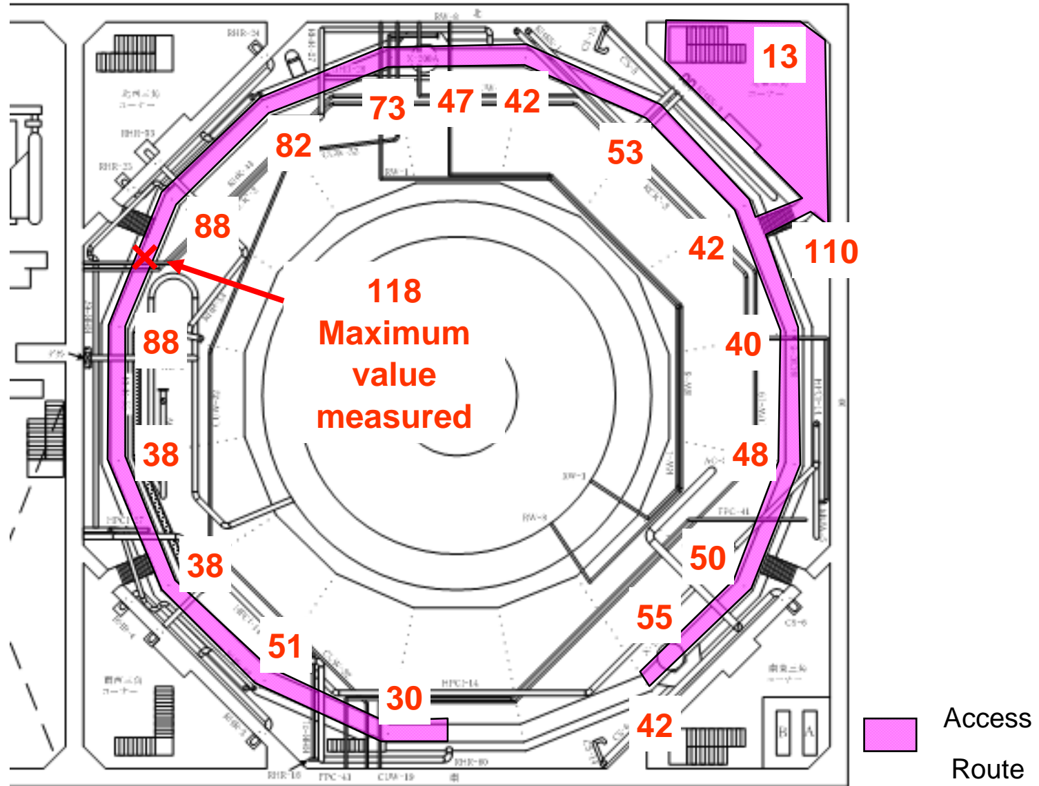
Air dose rate in the Torus Room (mSv/h)
