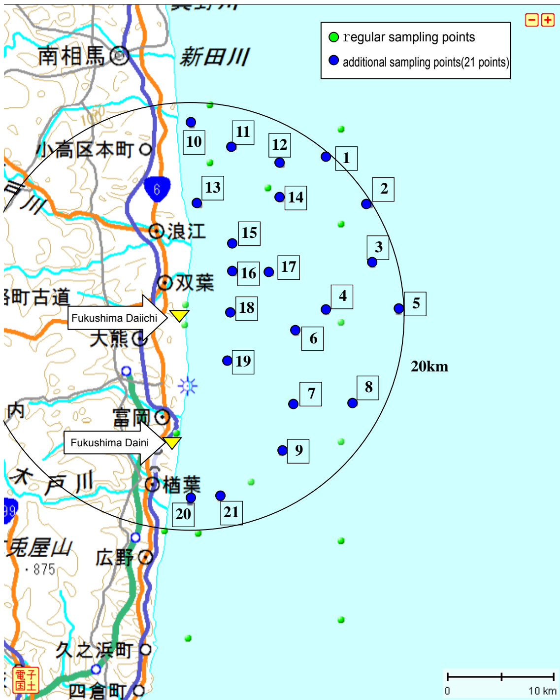
Sampling points of ocean soil within 20 kilometers of the Fukushima Daiichi Nuclear Power Plant for the inspection of marine products
