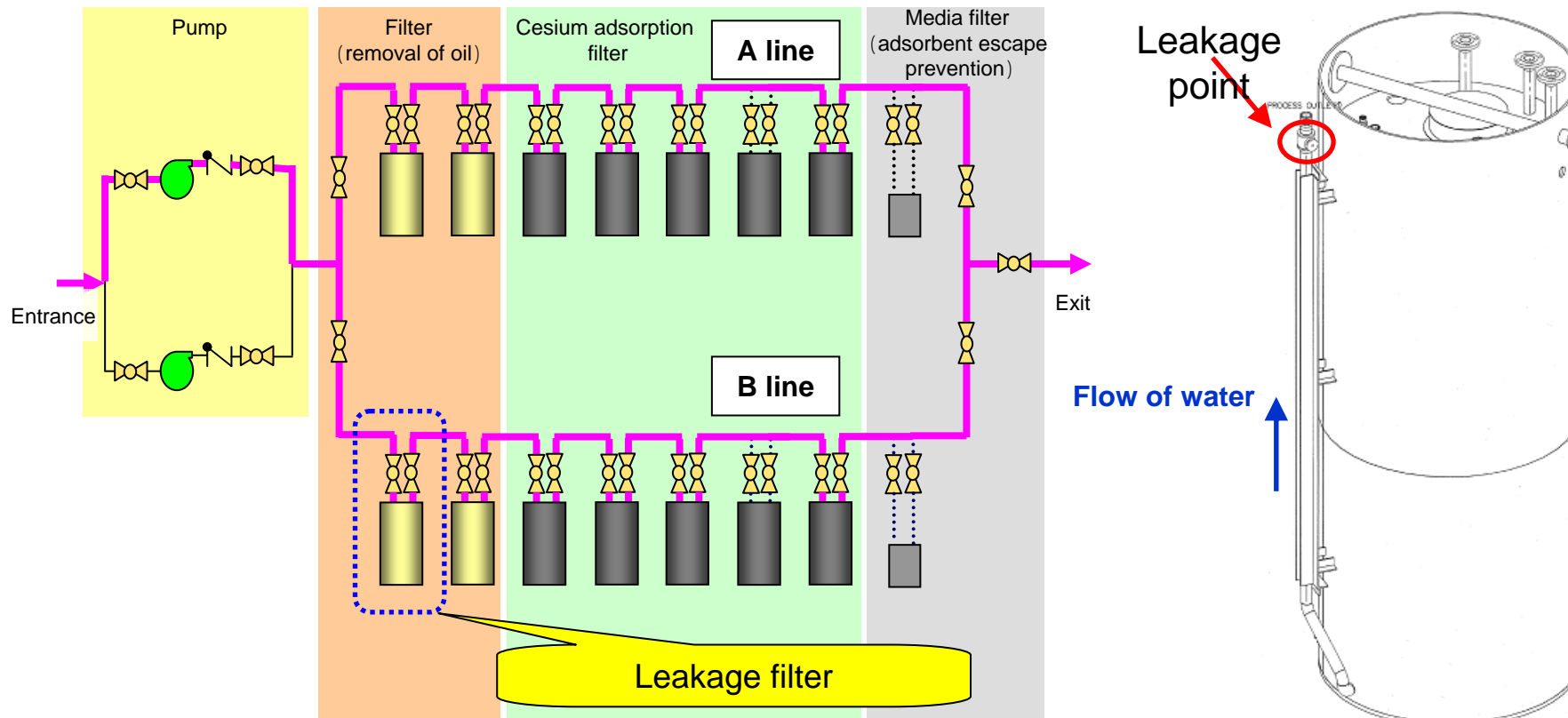
Image of 2nd Cesium adsorption apparatus (SARRY) system
