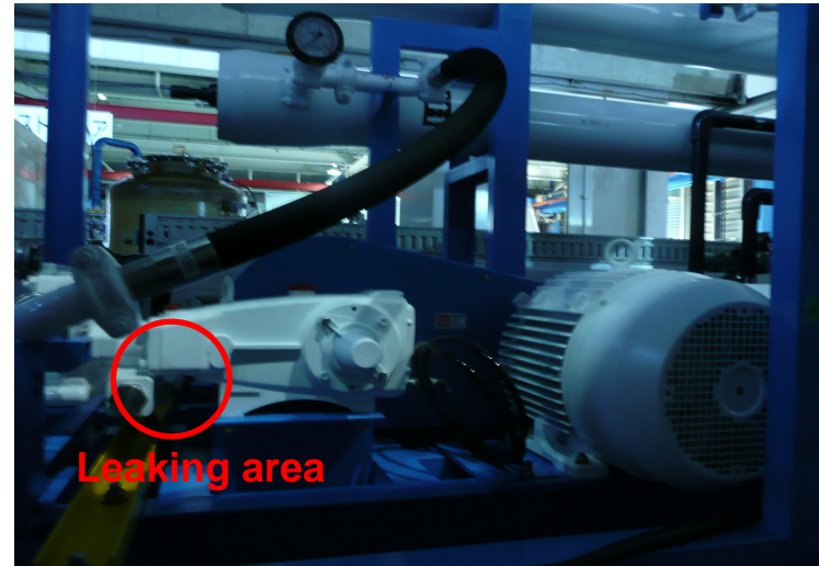
<High-pressure pump in reverse osmosis membrane unit>
