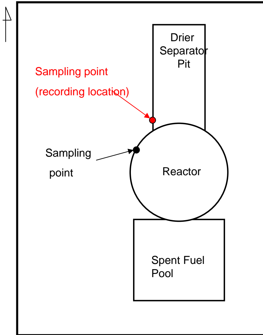
Layout drawing of 5 th floor of Unit 3 reactor building in Fukushima Daiichi Nuclear Power Station
