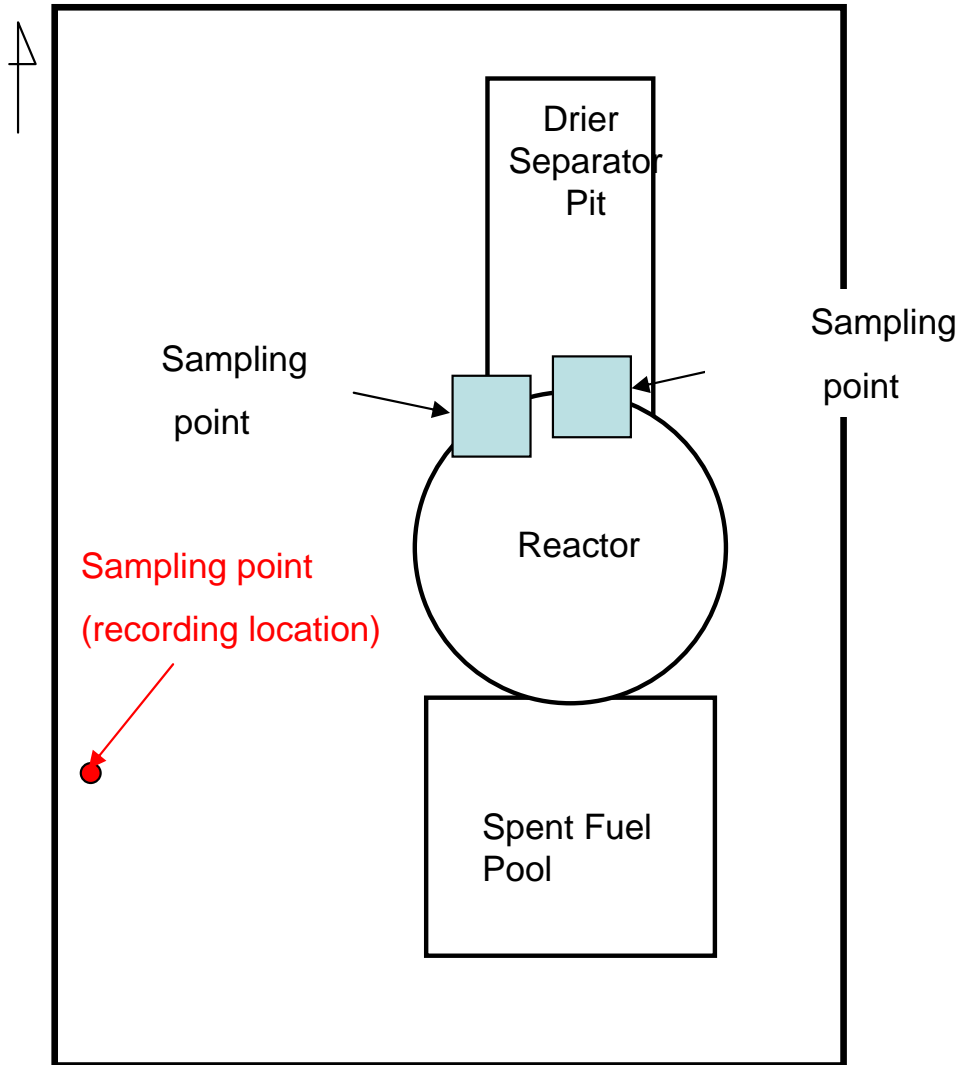
Layout drawing of 5 th floor of Unit 1 reactor building in Fukushima Daiichi Nuclear Power Station
