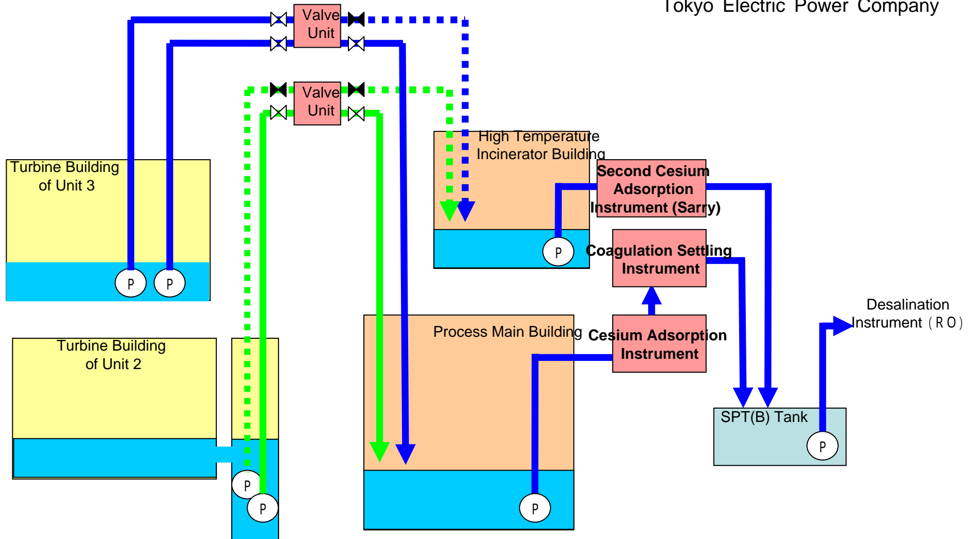
Image of Water Transfer Accumulated in Turbine Buildings of Unit 2 and Unit 3
