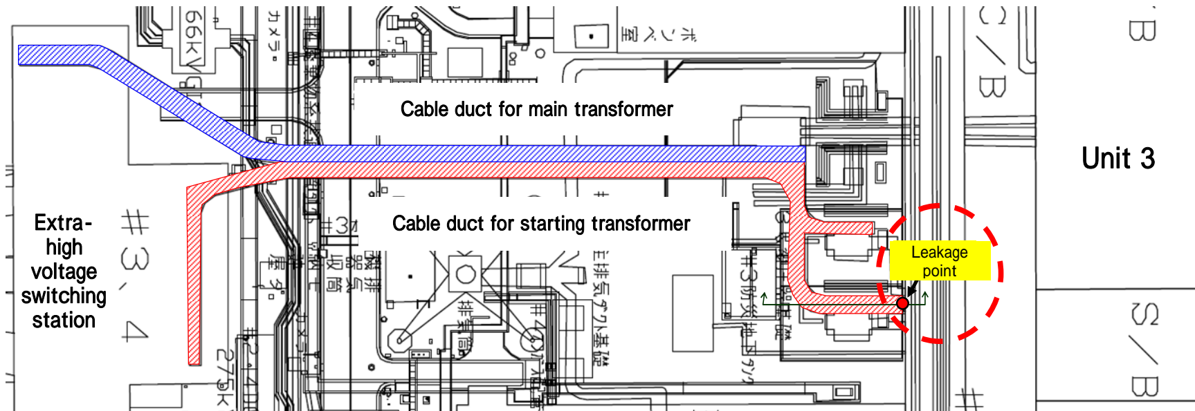
Ground plan of transformer yard, Unit 3
