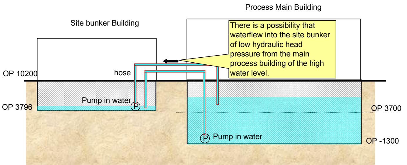
Cross-section diagram of site bunker and main process building (Line A-A)
