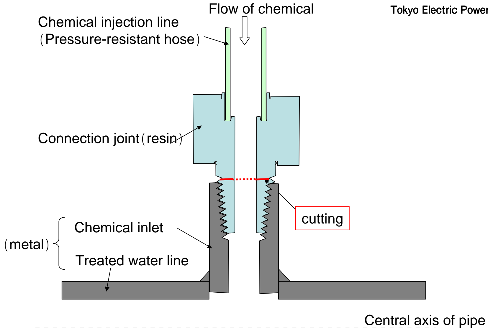
Outline structure of damaged part on chemical injection line for coagulation settling equipment
