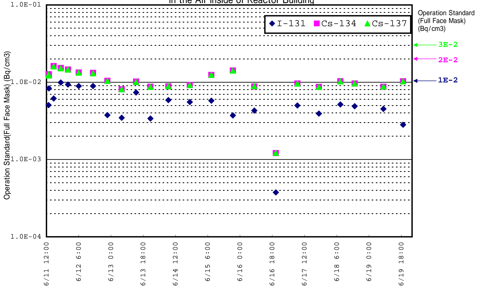
Unit 2 of Fukushima Daiichi Nuclear Power Station, Transition of Radioactive Materials Density in the Air inside of Reactor Building
