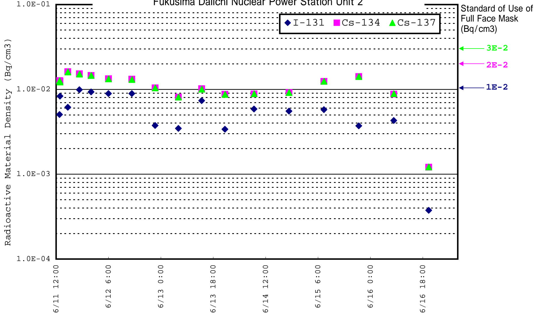
Change of Radioactive Material Density in the Air in the Reactor Building Fukushima Daiichi Nuclear Power Station Unit 2
