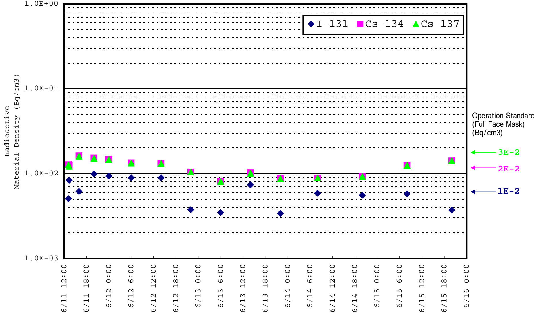
Unit 2 of Fukushima Daiichi Nuclear Power Station, Transition of Radioactive Materials Density in the Air inside of Reactor Building
