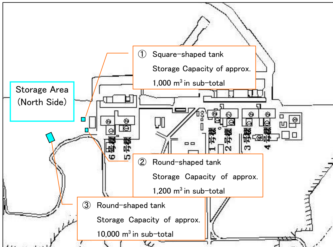
Fukushima Daiichi Nuclear Power Station Layout
