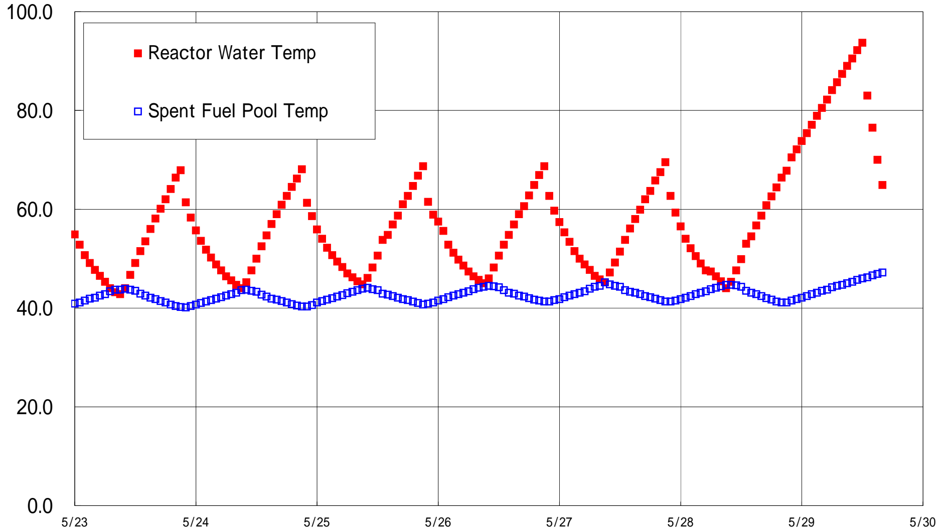
Temperature of Reactor Water and Spent Fuel Pool, Unit 5 Fukushima Daiichi NPS
