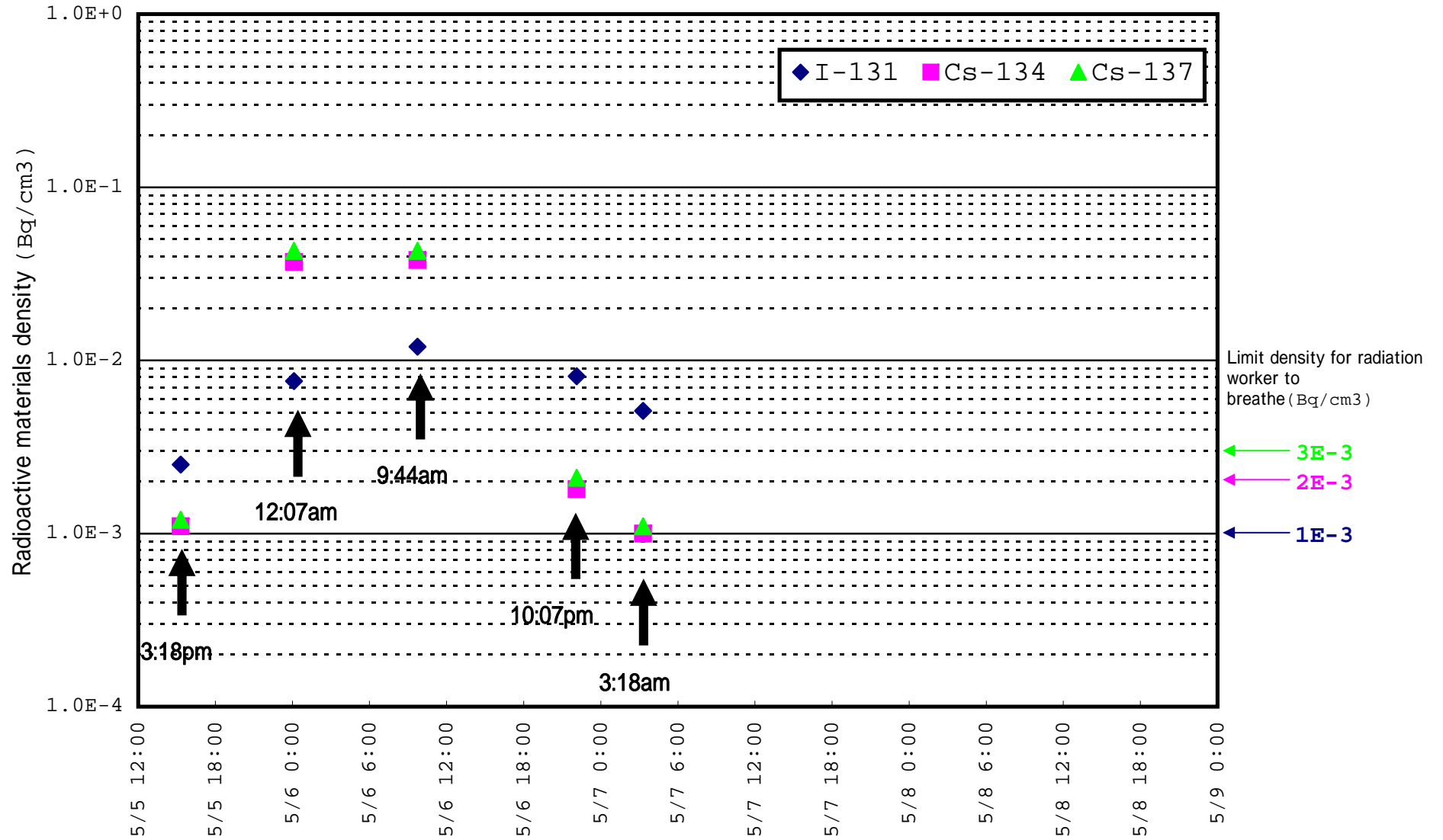
Unit1 Trend of air's radioactive materials density inside R/B
