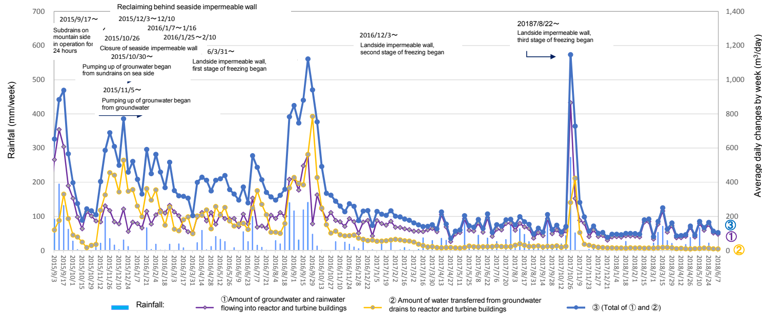
Amount of water transferred from groundwater drains to reactor and turbine buildings (From May 31, 2018 to June 6, 2018)
