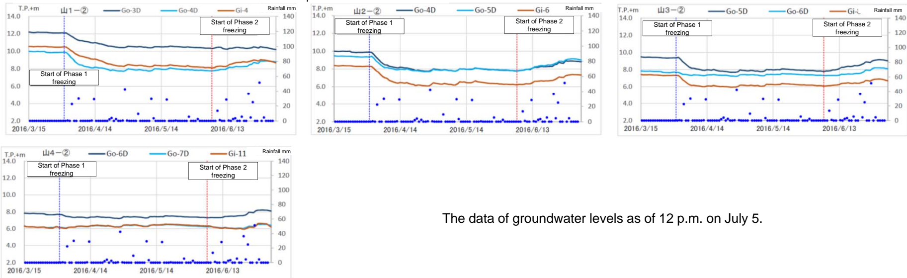
8. Groundwater levels inside and outside of the Landside Impermeable Wall
