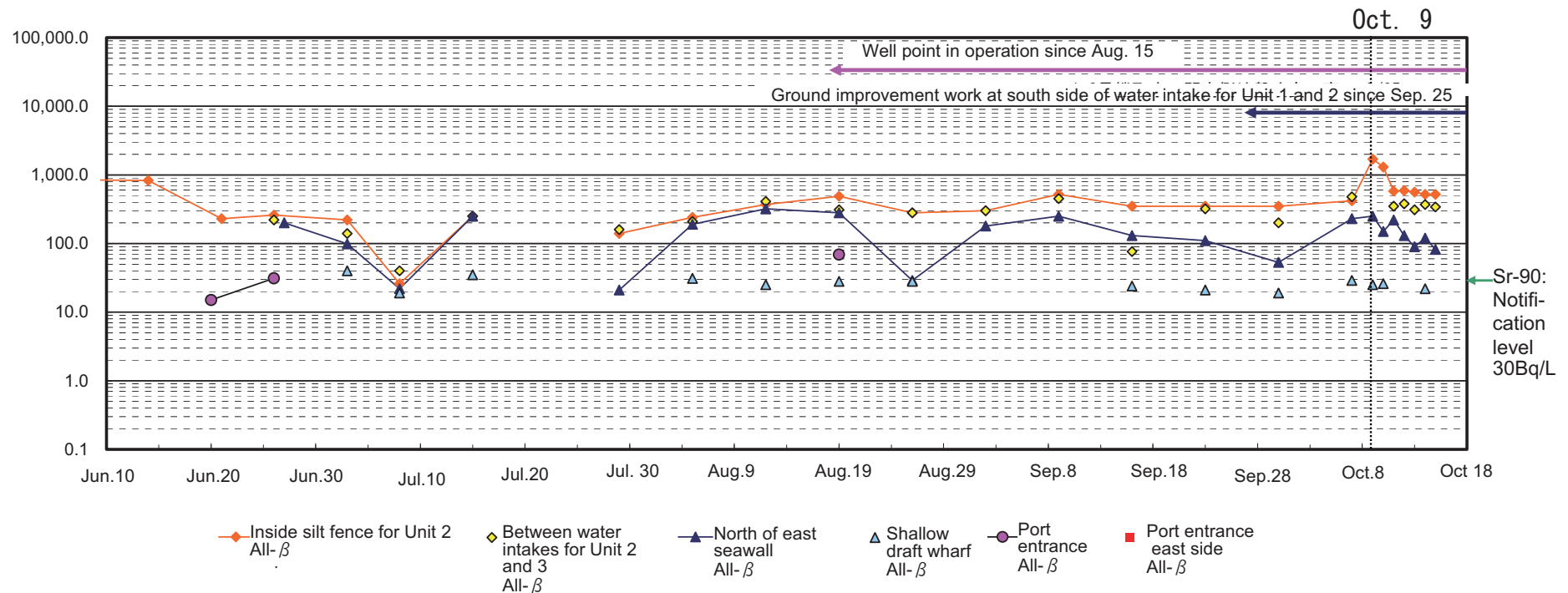
Transition in seawater concentration inside silt fence for Unit 2 and port entrance east side (All-β)
