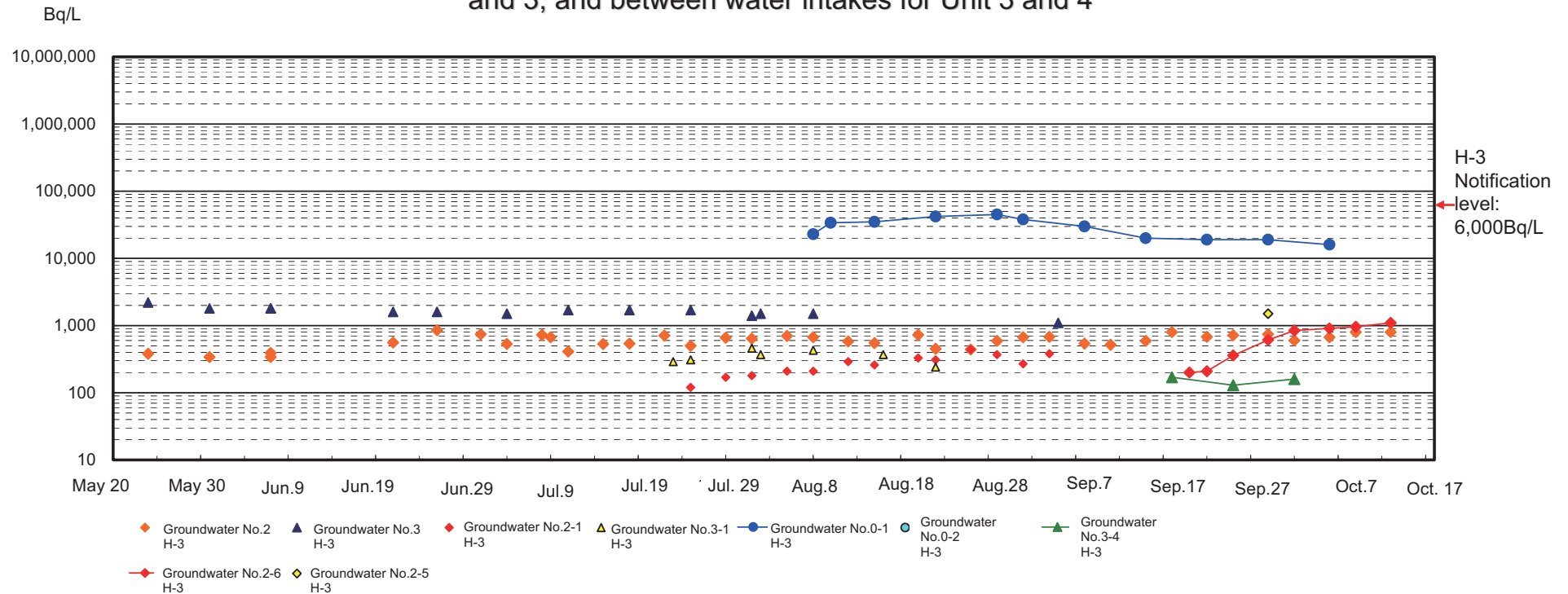
Transition in groundwater tritium concentration at north of Unit 1, between water intakes for Unit 2 and 3, and between water intakes for Unit 3 and 4
