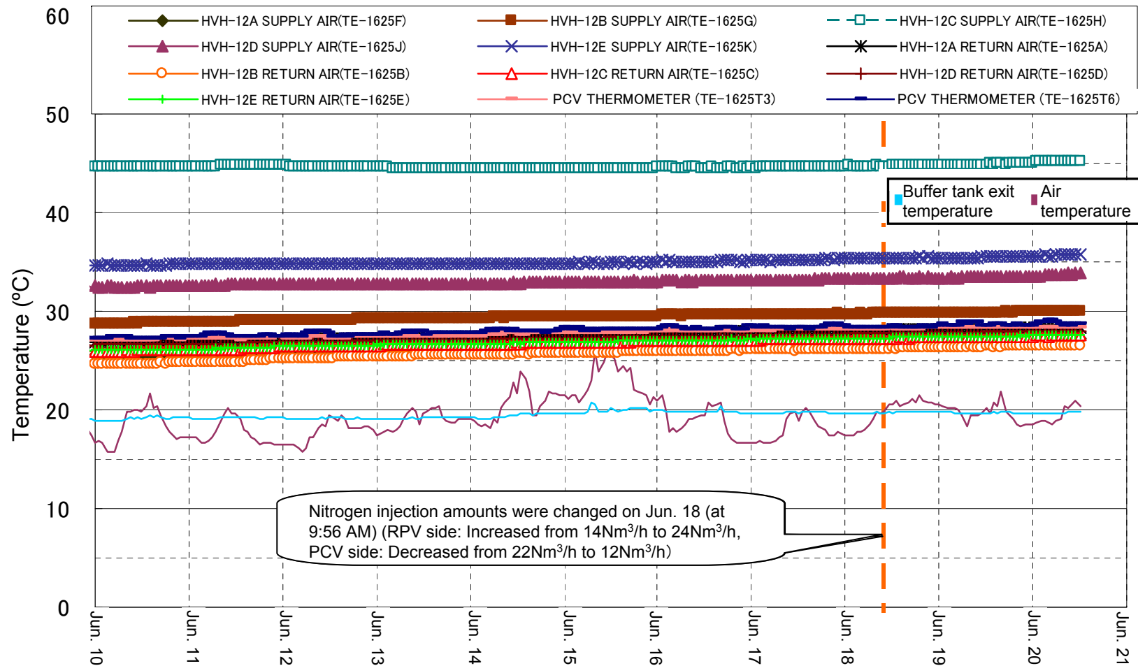
Graph of temperatures inside Unit 1 PCV
