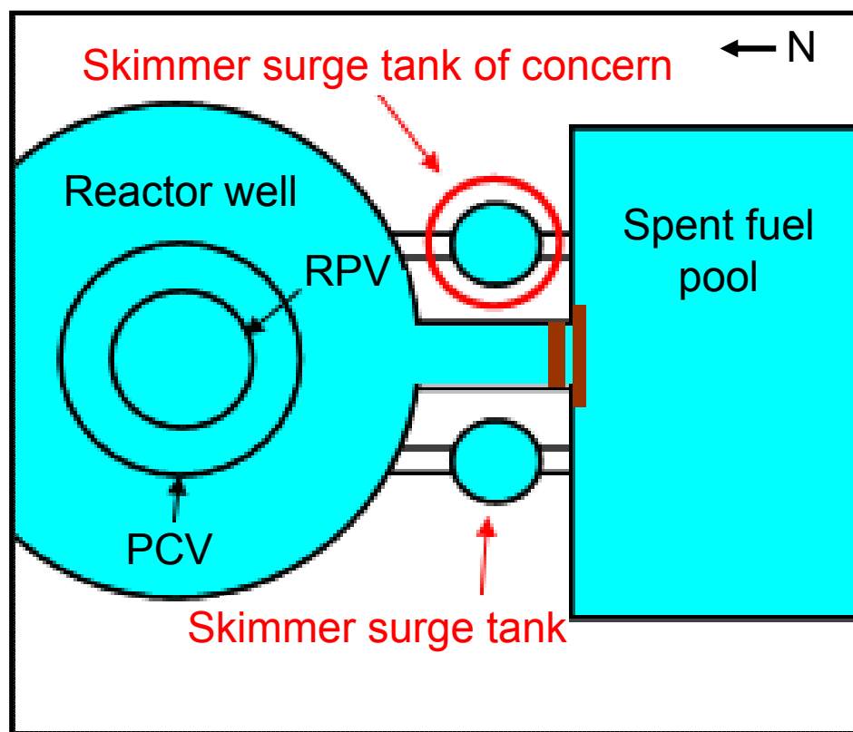
Location of the skimmer surge tank
