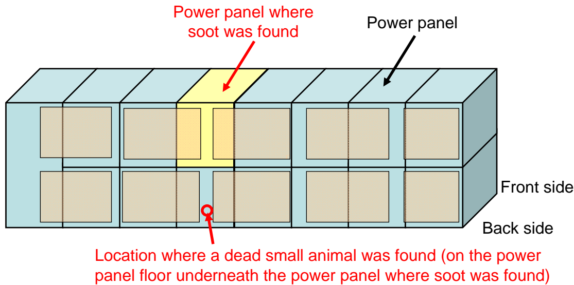
Units 3-4 temporary M/C M/C (A) power panel and its door
